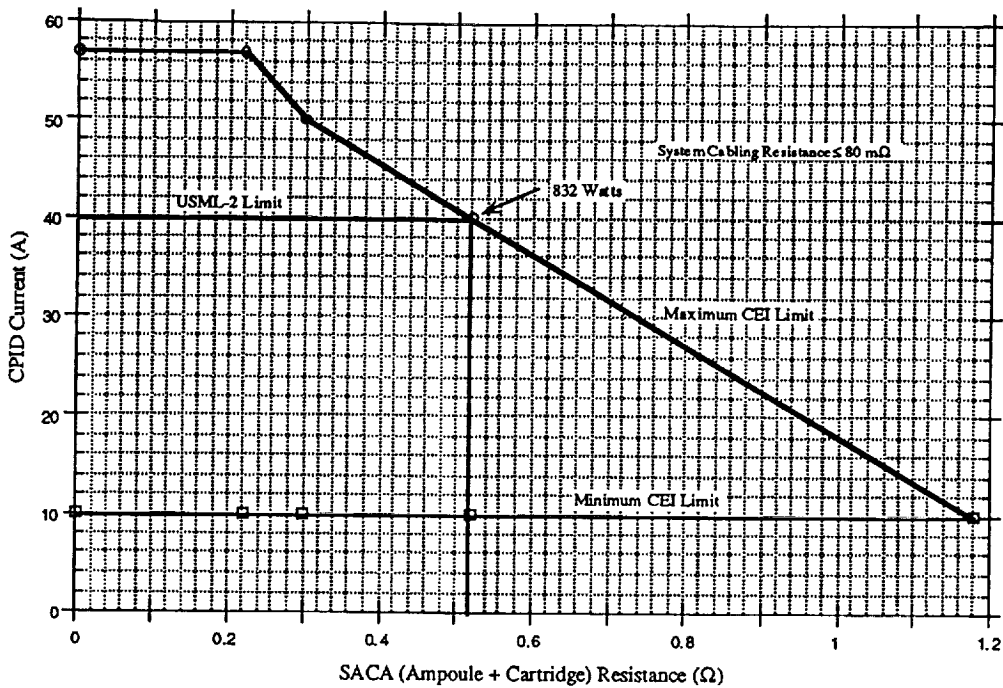
Fig. 1. CPID Current versus SACA Resistance.
