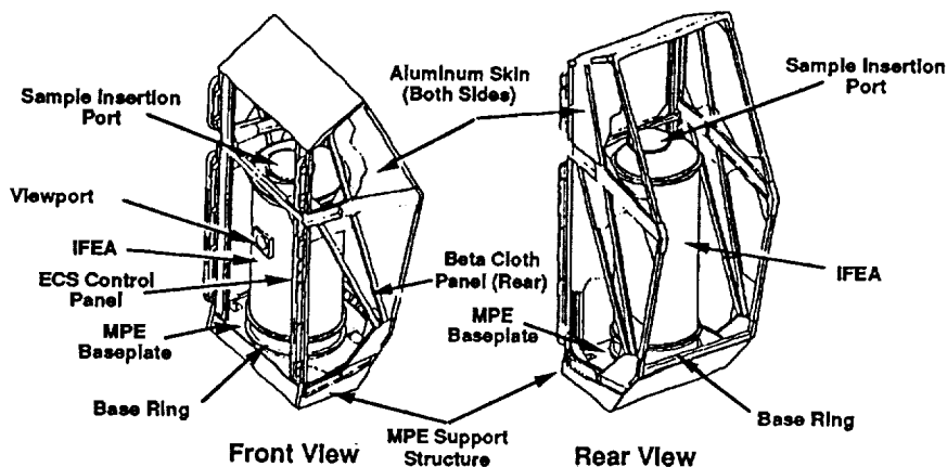
Fig. 5. IFEA Mounting in CGF Support Structure.
