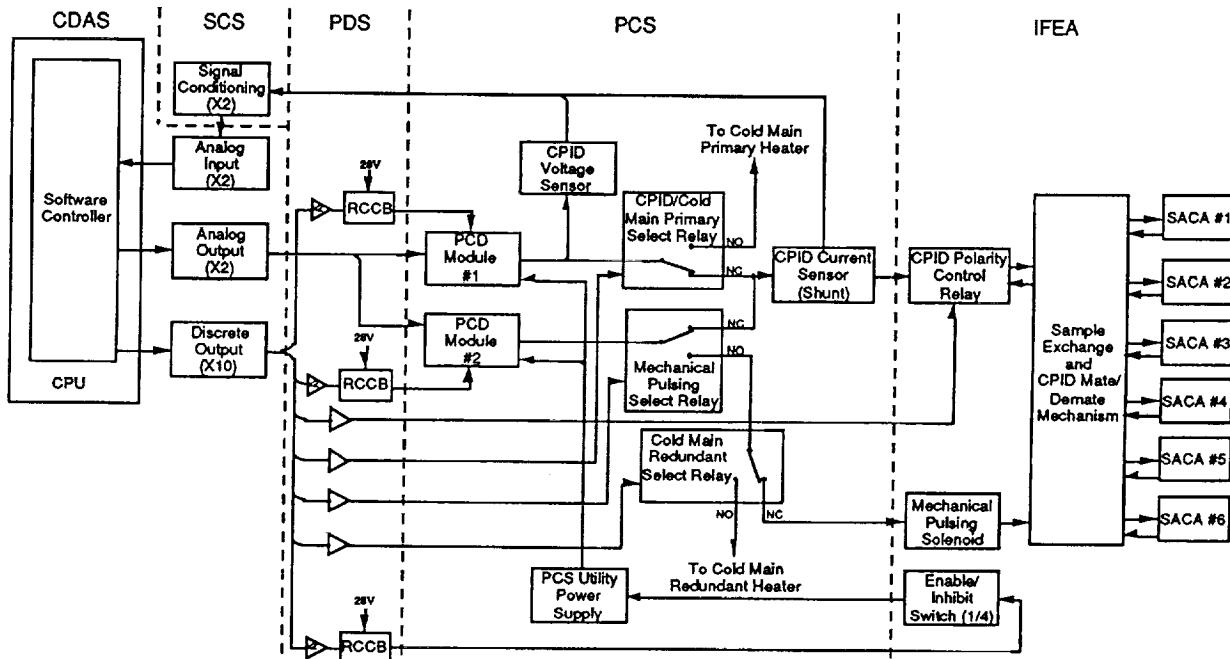
Fig. 2. CGF Sample Interface Demarcation System Block Diagram.
