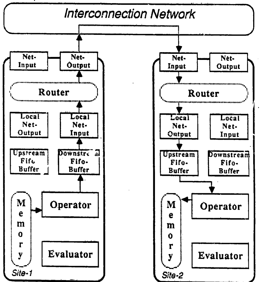
Figure 3: Network component interconnections. Packets travel in the direction marked by arrows. Flow control information flows in the opposite direction.
