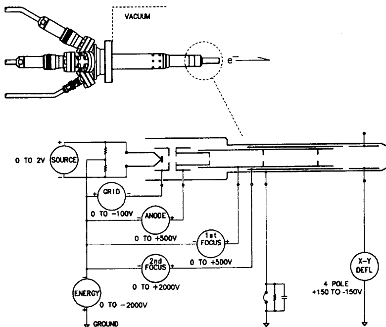
FIG. 3. Schematic diagram of the electrostatic electron gun and associated electronics [34]. A unipotential tungsten cathode produces an electron beam of low energy spread (~0.3 eV). The lens design enables a constant focal plane position and spot size to be maintained over the energy range in which measurements are made (0.2–1.8 keV). Typical beam currents are ~5 \mu A. The X and Y deflectors provide beam steering capability.
