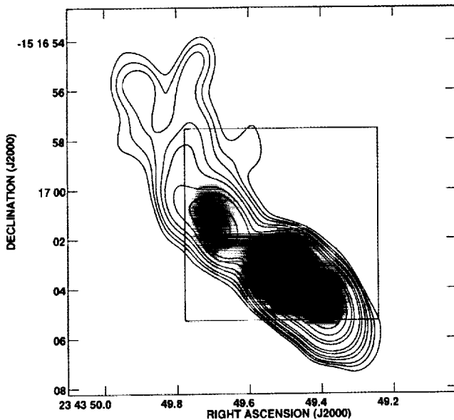
FIG. 2.—Gray-scale of the 1994 HST /FOC ultraviolet image ( \sim 2330 Å) that has been convolved with a 1''.67 \times 1''.25 FWHM Gaussian to permit same-resolution comparison with a 6 cm contour plot of the 1995 6 cm VLA image of the R Aqr jet. Radio contours are 0.08, 0.12, 0.16, 0.24, 0.32, 0.36, 0.64, 1.20, 1.60, 2.56, 3.84, and 5.12 \text{mJy beam}^{-1} , and the peak radio flux is \sim 10.0 \text{ mJy beam}^{-1} . The box delimits the field of view of the HST image relative to the VLA image. Comparison of the radio image with the nearly contemporaneous HST /FOC ultraviolet image suggests that the ultraviolet emission could encompass the radio emission in a sheath if a shock model applies.
