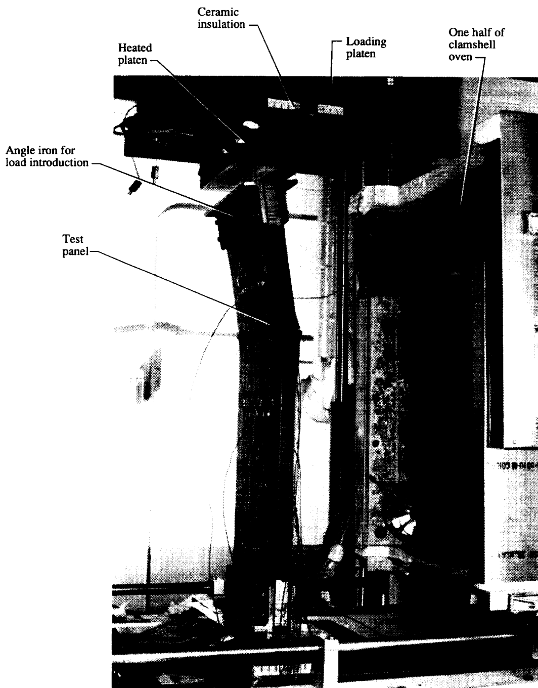
Figure 4. Photograph of failed panel located in test stand.
