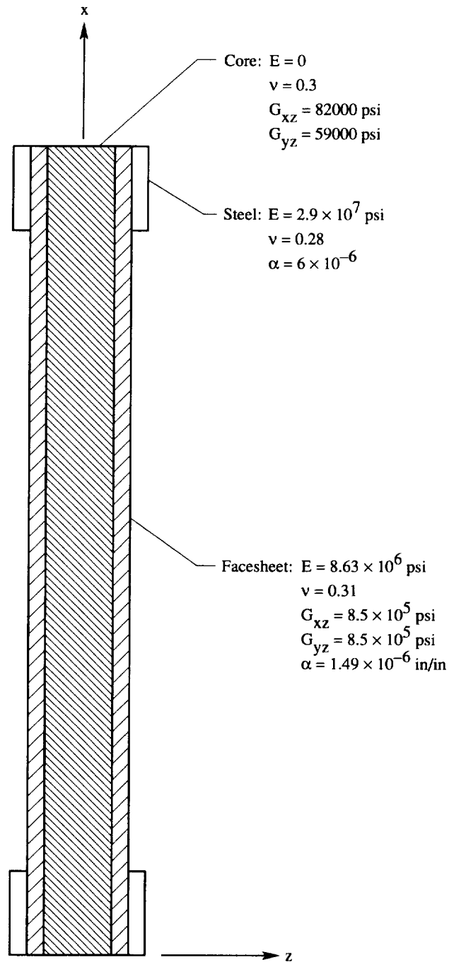
Figure 5. Schematic diagram of layers represented in the composite plate finite element model and their material properties. Note: drawing is not to scale.
