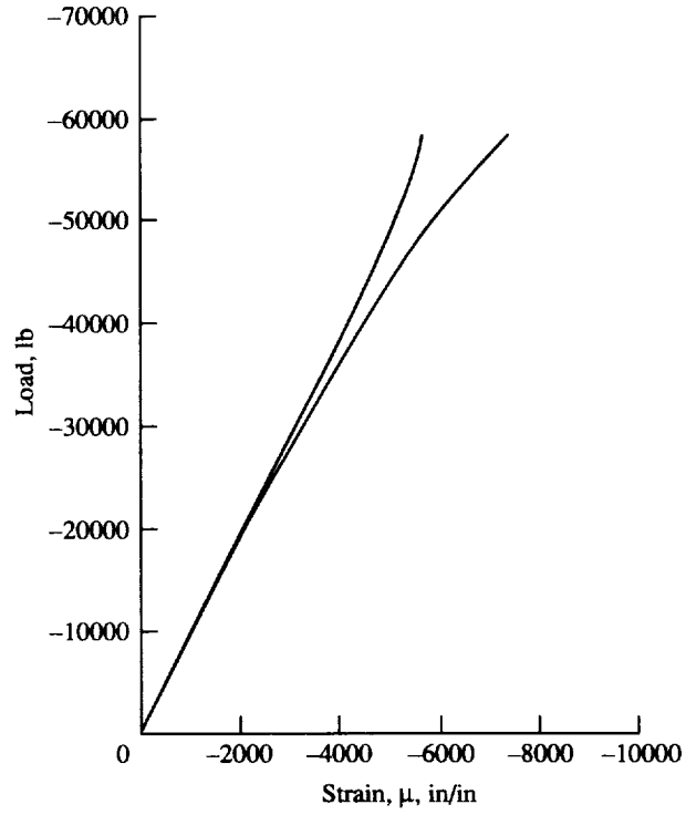
Figure 13. Back-to-back measured strains at center of panel facesheets for Panel 1 having 8-ply facesheets.
