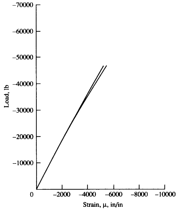
Figure 14. Back-to-back measured strains at center of panel facesheets for Panel 5 having 8-ply facesheets.
