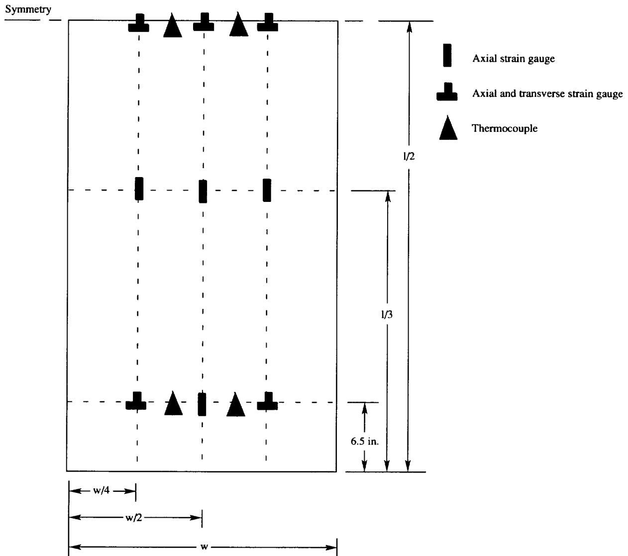
Figure 3. Typical instrumentation diagram where all gauges are mounted back-to-back and mirrored in the length, l , direction.
