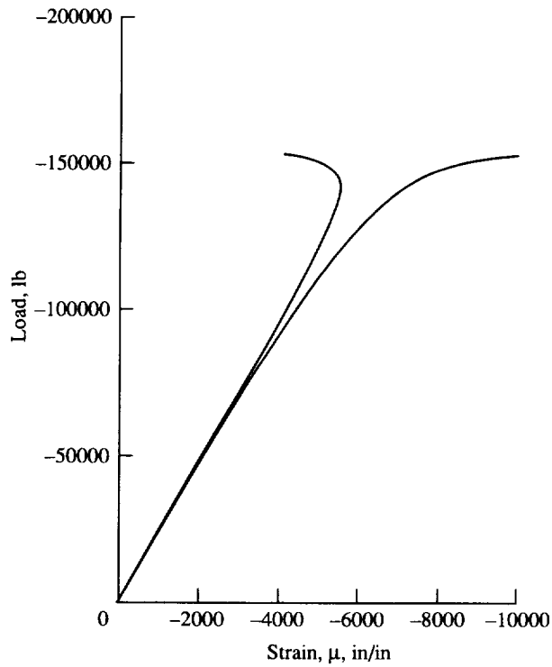
Figure 15. Back-to-back measured strains at center of panel facesheets for Panel 11 having 8-ply facesheets.
