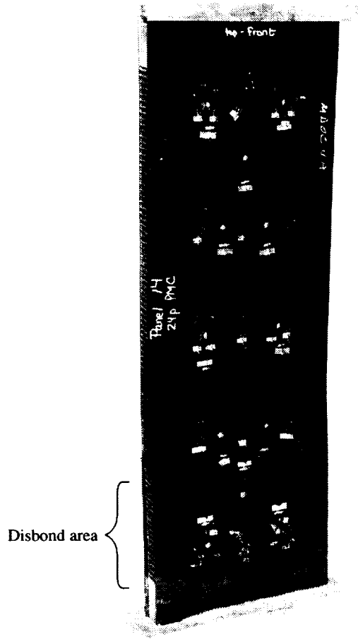
Figure 10. Photograph of Panel 14, with 24-ply facesheets and potted ends only, after testing to failure.
