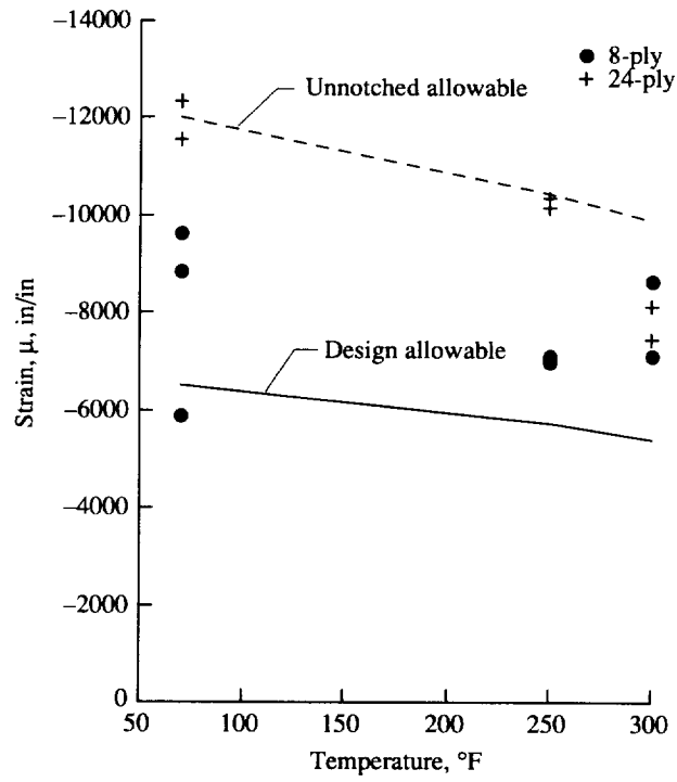
Figure 11. Maximum measured failure strain data.
