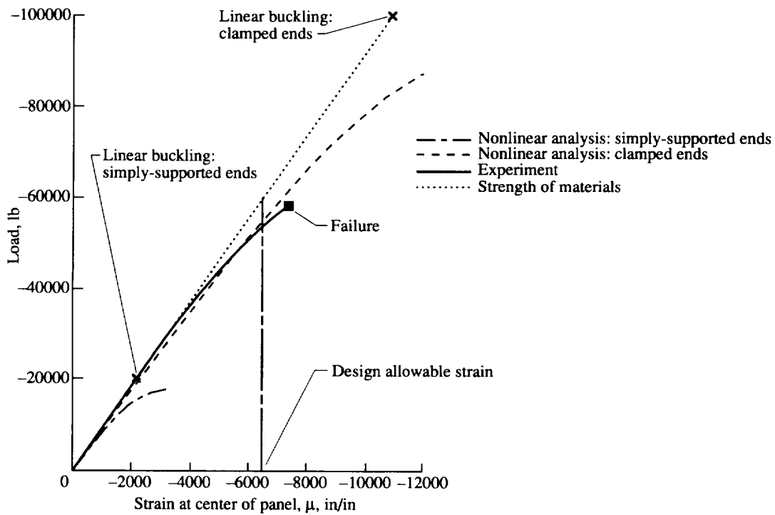
Figure 16. Room temperature NASTRAN nonlinear composite plate finite element analysis for Panel 1 (Geometric imperfection modeled from first cosine shape buckling mode).
