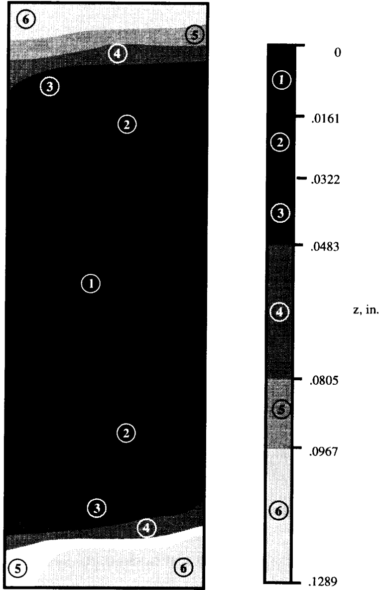
Figure 7. Contour plot of Panel 2 out-of-plane measurements.
