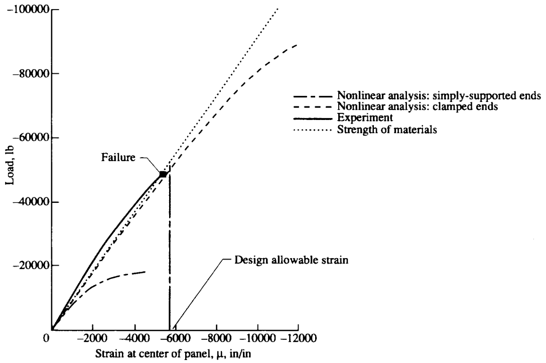
Figure 17. NASTRAN nonlinear composite plate finite element analysis for Panel 2 at 300°F (Geometric imperfection modeled from actual out of plane measurements mapped to nodal points).
