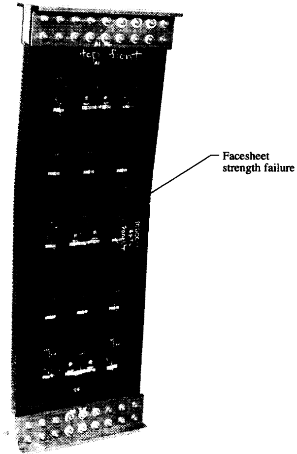
Figure 8. Photograph of Panel 4, with 8-ply facesheets, after testing to failure.
