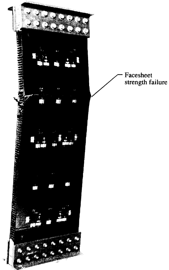
Figure 9. Photograph of Panel 11, with 24-ply facesheets, which buckled prior to failure.
