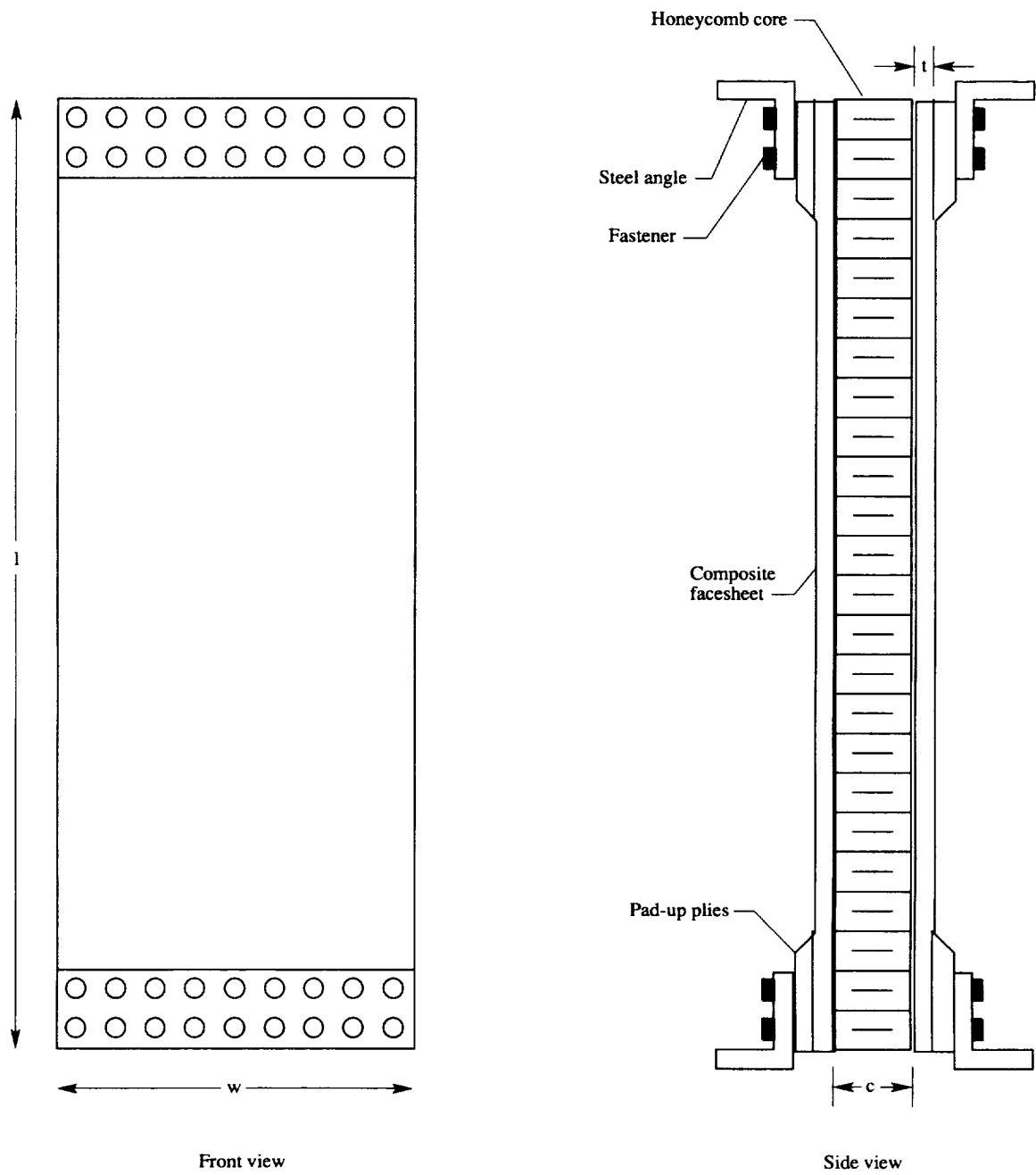
Figure 2. Schematic diagram of test specimen. Note: drawing is not to scale.
