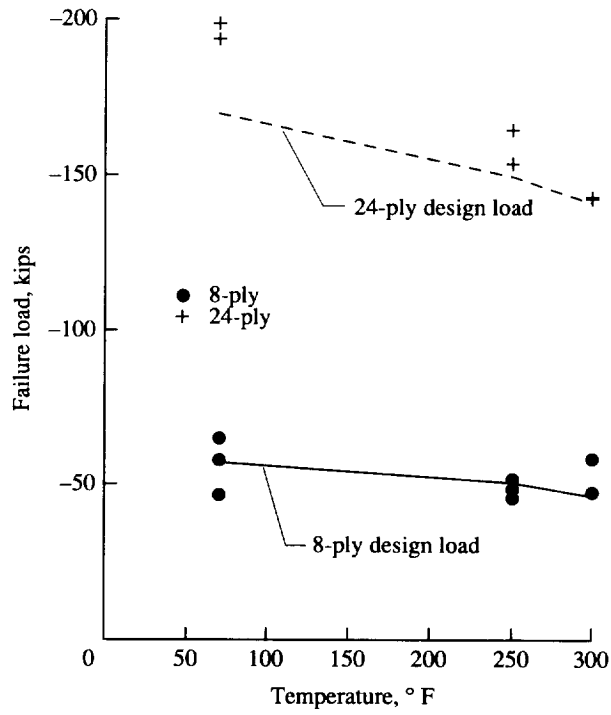
Figure 12. Panel failure load test data.
