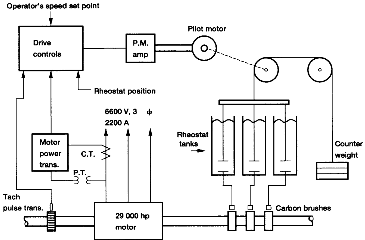
Figure 3.—Drive motor speed control schematic.
