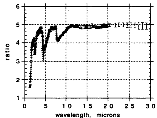
Fig. 1. Ratio of a \tau to a CMA.
