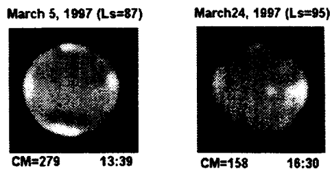
Fig. 1. Equatorial cloud belt in March of 1997 (blue).
