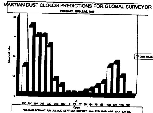
Fig. 1. The above chart shows the ALPO Mars section dust clouds prediction for NASA Global Surveyor. When the spacecraft commences regular imaging next March, Mars will be at the height of its dust season. While dust storms can occur during any martian season, there are two main peaks of activity as shown in the above chart. High dust activity just a month before the prime mission starts imaging Mars is predicted. This is reminiscent of the Mariner 9 global dust storm. The 1973 dust started at L_s = 300^\circ and in March 1998 we will be at L_s = 285^\circ . Global dust is very rare, but we do expect to see a few strong dust storms at this time. The seasonal index is a simple index and graphically indicates the average departure from the "normal" for any given martian subseason. It is arbitrarily set so that the average value for all 12 sub
