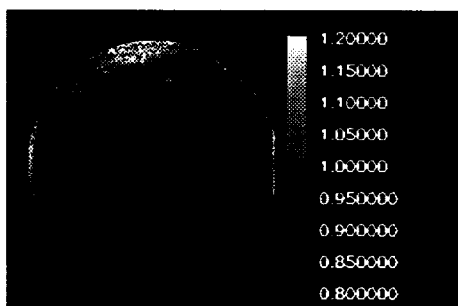
Fig. 3. Band-depth map centered at 3.69 \mu\text{m} using local continuum images at 3.40 \mu\text{m} and 3.80 \mu\text{m} . The value at the north polar region is greater than one, indicating a fine-grained frost.
