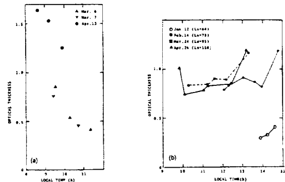
Fig. 3. Diurnal variation of opacity for (3a) morning cloud at 120°W and 10°N in 1995 and (3b) Olympus cloud in 1997.
