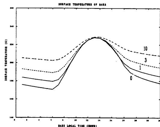
Fig. 2. Effect of polar hood. Latitude = 60^{\circ}\text{N} ; L_s = 180^{\circ} . Optical thickness of \text{H}_2\text{O} ice = 0, 1, 3, 10.
