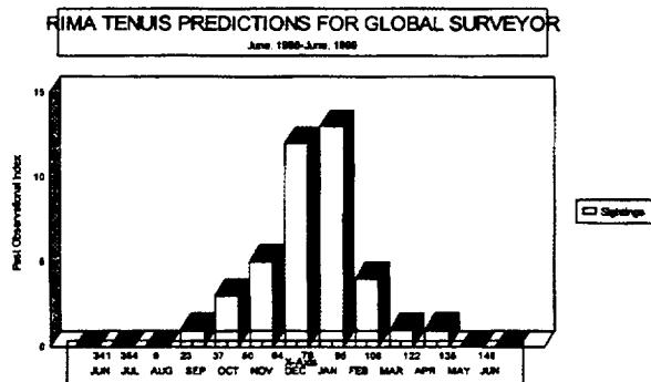
Fig. 2. This chart shows the ALPO Mars section predictions for when the Rima Tenuis might next be visible. Both the G. S. and HST have the opportunity, along with groundbased observers, to look for it. This will be the last chance to hunt for it until 2007. If we can confirm that the Rima Tenuis is an NPC dust event, then we can go back to look at past observations and study the long-term variation of NPC dust clouds. Chart prepared by D. M. Troiani.
