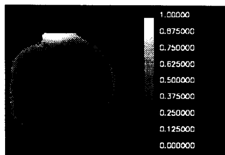
Fig. 4. North polar region endmember fractional abundance map. Morning and evening regions are shown to be modeled with up to 50% of this endmember, indicating the existence of fine water frost in these regions.
