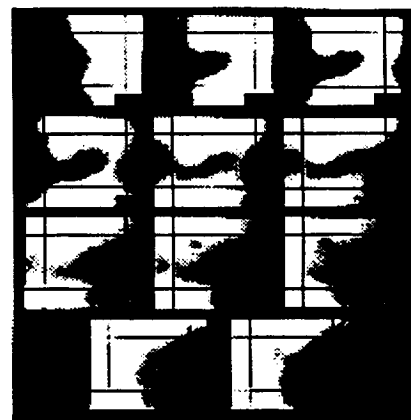
Fig. 2. Time series of 11.7- \mu\text{m} thermal emission images of the Cerberus region of Mars. The black rectangle in each frame shows the bounds of the Elysium quadrangle (0°–30°N and 180°–225°W).
