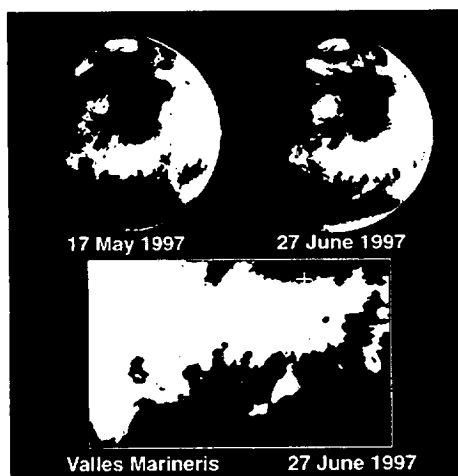
Fig. 1. Dust storm in Valles Marineris. Two full-disk HST images are shown (north is to the top); an extensive dust storm is evident in the June 27 image. A simple cylindrical projection map of the Valles Marineris region is shown at the bottom, extending from 25°S to 25°N latitude and 10° to 90° longitude. The Pathfinder landing site is marked by a +.
