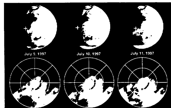
Fig. 3. Development of condensate clouds over three consecutive days. Full-disk HST images are shown (north to the top), with the Pathfinder landing site denoted by a +. Polar projection maps are shown below; 0° longitude is to the bottom and latitude circles are drawn at 40°N, 60°N, and 80°N. Note the movement of the prominent cloud (located near 45° longitude on July 9).
