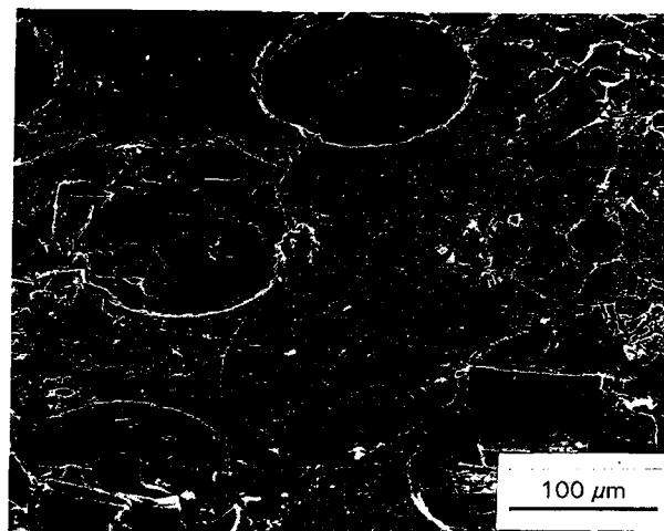
Figure 8 Surface morphology of type B' coated SiC-RBSN at end of composite after 170 h oxidation in 100 \text{ cc min}^{-1} dry flowing oxygen at 1000°C.
