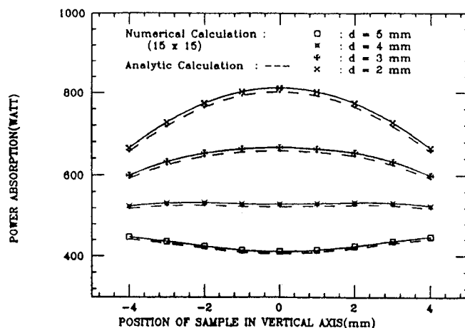
Fig. 11. Effects of coil separation and the sample positions on the power absorption (for 1 g iron drop with in-phase 300 A current 450 kHz; by the coils of [24], d: half distance between upper and lower coils).
