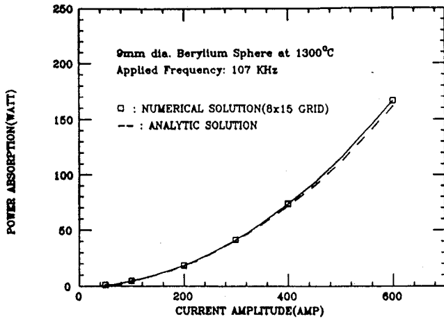
Fig. 4. Variation of power absorption with applied current (by the coils of [4]).
