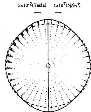
Fig. 17. Computed shape of the squeezed sample by the present electromagnetic calculation scheme (for 10 mm dia silver drop with 280 A, 144 kHz).
