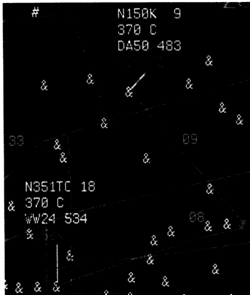
Figure 3. Conflict lines from aircraft to the point of first loss of separation.
