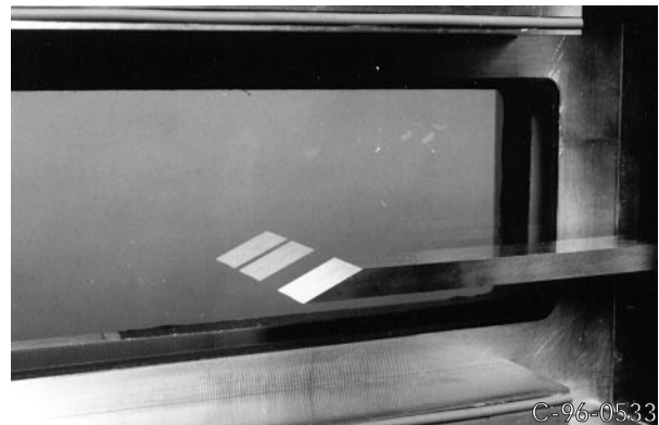
Figure 23.—Optical reflection of the wedge face on the channel back sidewall.
