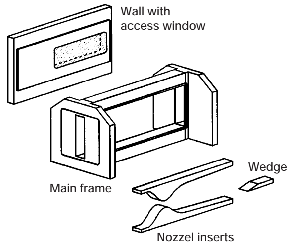
Figure 3.—Three-dimensional view of the test section.
