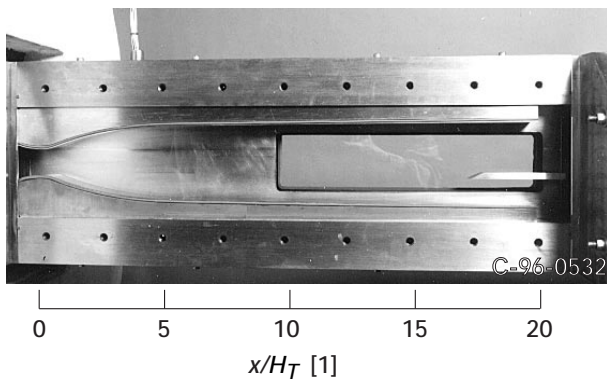
Figure 2.—Test section with front sidewall removed ( H_T = 36 \text{ mm} ).
