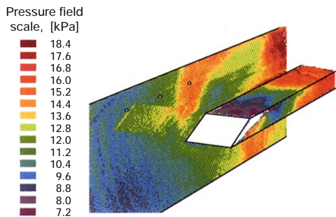
Figure 24.—PSP signal reflection of the wedge face pressure field on the channel backwall pressure field (test condition C-140).
