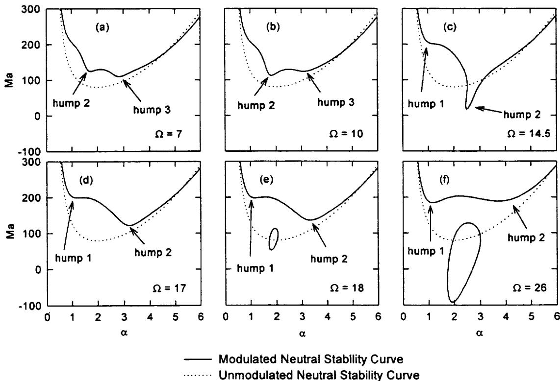
Figure 1 Neutral Stability Curves for \text{Pr}=1. , g_0=0 , g_1=5 , \text{Ra}=1000
