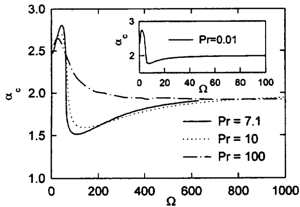
Figure 3 Critical wavenumber, \alpha_c , versus modulation frequency, \Omega , for varying Pr values. Ra = -1000 , g_0 = 0 , g_1 = 5 .
