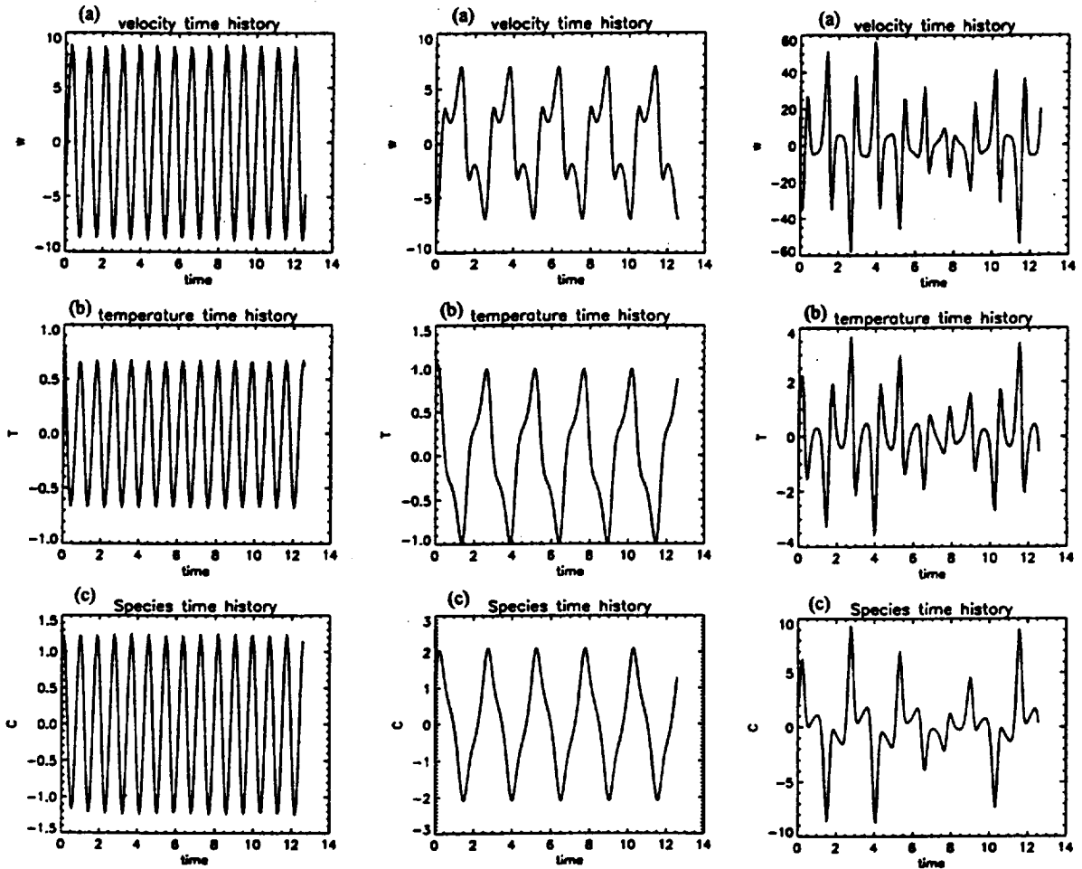
Figure 11 unmodulated oscillatory behavior Figure 12 subharmonic behavior Figure 13 quasiperiodic behavior
