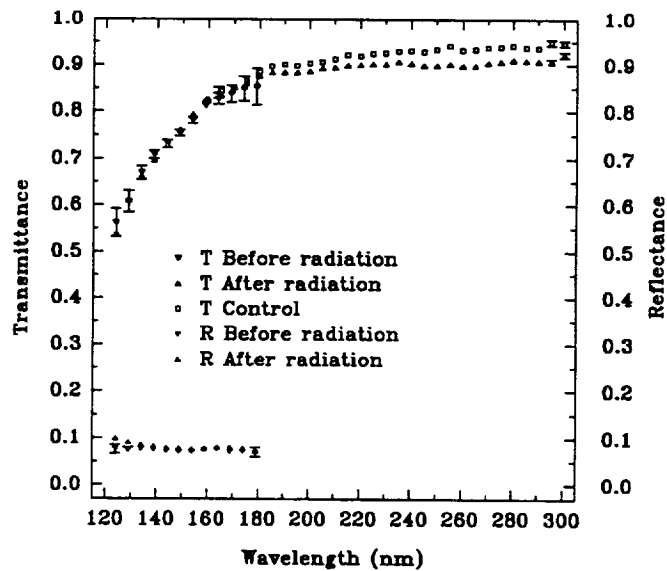
Figure 5: Reflectance and transmittance of a CaF 2 thin film on a MgF 2 substrate. Comparison is shown in the 120 nm to 180 nm range before and after radiation exposure of a single sample. In the 160 nm to 300 nm range, comparison is between the radiation exposed sample and a control sample with no radiation exposure.
