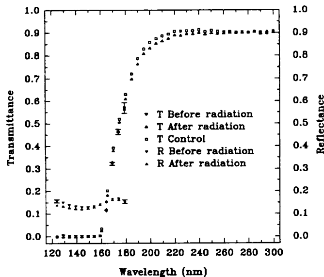
Figure 3: Reflectance and transmittance of an Al 2 O 3 thin film on a fused silica substrate. Comparison is shown in the 120 nm to 180 nm range before and after radiation exposure of a single sample. In the 160 nm to 300 nm range, comparison is between the radiation exposed sample and a control sample with no radiation exposure.
