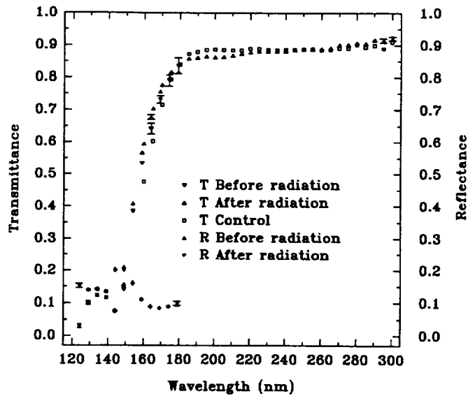
Figure 4: Reflectance and transmittance of a BaF 2 thin film on a MgF 2 substrate. Comparison is shown in the 120 nm to 180 nm range before and after radiation exposure of a single sample. In the 160 nm to 300 nm range, comparison is between the radiation exposed sample and a control sample with no radiation exposure.
