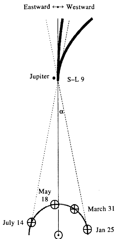
Fig. 1. Lines of sight from Earth \oplus to S-L 9 are shown for selected HST observations acquired in 1994. A continuous stream of dust grains larger than about 5 \mu\text{m} contribute curved tails that always appear west of the fragment (dark grey curve), whereas smaller grains contribute straighter tails that appear east of the fragment (light grey curve) when observed after solar opposition. Dust tails are not drawn to scale
