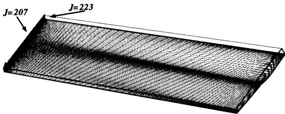
Figure 6.8: WING-WAKE-CORE extruded boundaries and generated outer domain.
