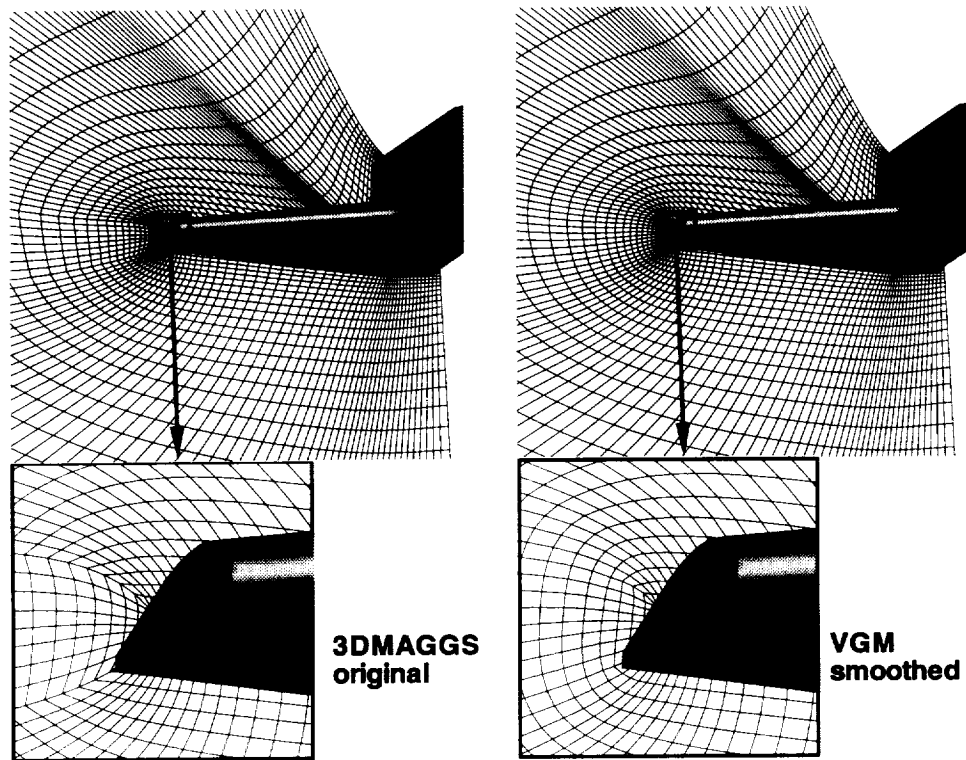
Figure 7.3: Elevation parametric design change volume grid with improved wingtip grid-line quality.
