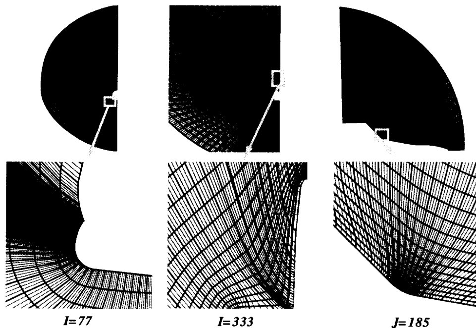
Figure 4.7: Evolution of viscous basis grid from 3DMAGGS to VGM.
