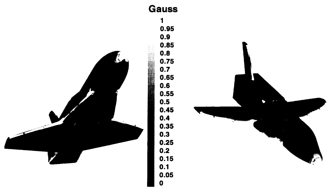
Figure 3.4: Gaussian curvature on the baseline geometry.
