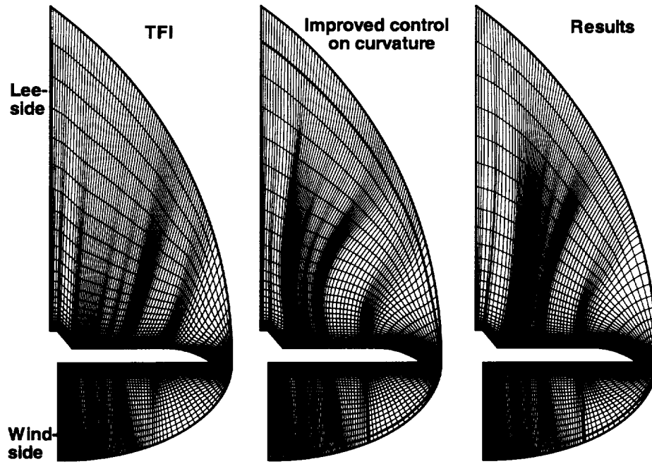
Figure 4.3: Viscous grid - symmetry surface generation process.
