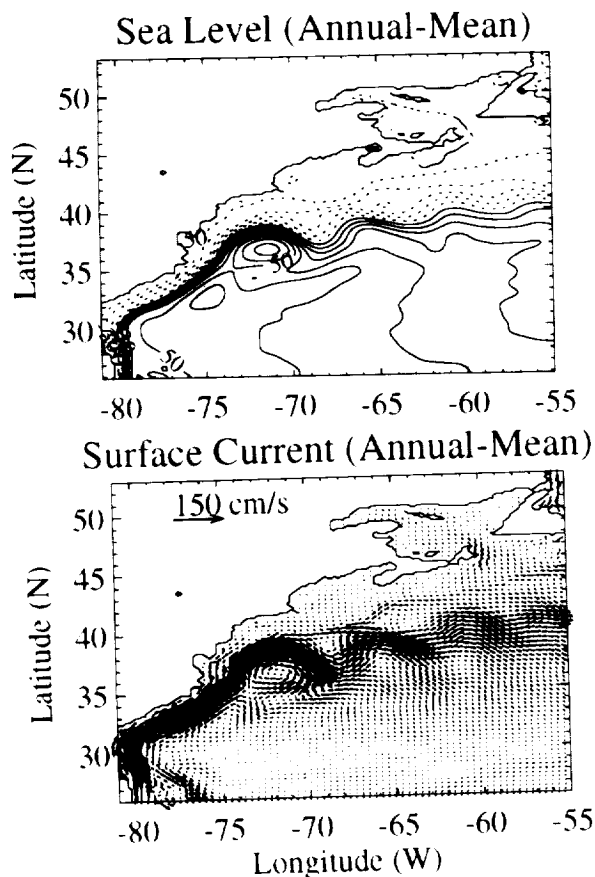
Figure 1. Climatological annual-mean maps of (top) sea surface height and (bottom) surface current simulated by the present model averaged over the last ten years of the third experiment. The contour interval is 10 cm.
