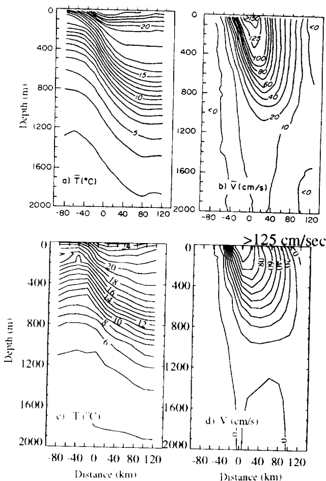
Figure 4. The observed (a and b) and simulated (c and d) temperature and downstream velocity calculated in the stream coordinate system. The contour interval is 1^\circ\text{C} for temperature, 10\text{ cm s}^{-1} for velocity less than 100\text{ cm s}^{-1} and 25\text{ cm s}^{-1} otherwise.
