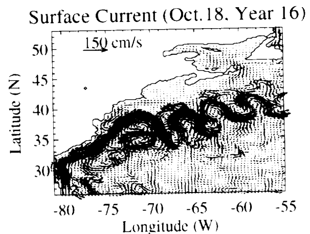
Figure 2. Instantaneous map of surface current simulated by the present model on October 18 of year 16.
