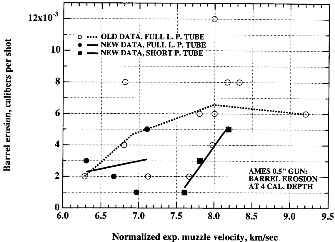
Figure 12. Experimental erosion (calibers/shot) for the Ames 0.5" gun for old 1960s data and for the seven recent shots shown in figure 11. The gun erosion is measured at 4 calibers depth in the barrel. "Full L.P. Tube" denotes full length pump tube and "Short P. Tube" denotes the shortened pump tube.
