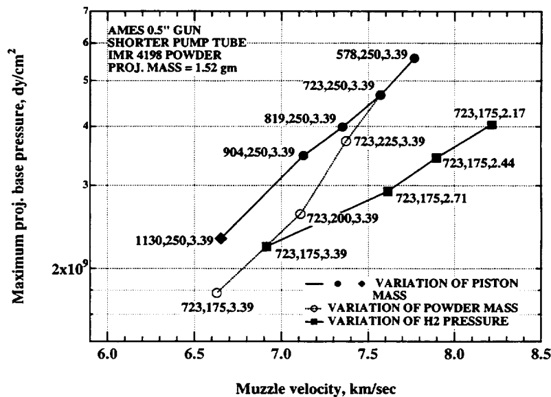
Figure 9. Maximum projectile base pressure versus muzzle velocity, showing the effects of varying piston mass, powder mass, and hydrogen fill pressure. Numbers beside data points are piston masses (gm), powder masses (gm), and hydrogen fill pressure (bar).
