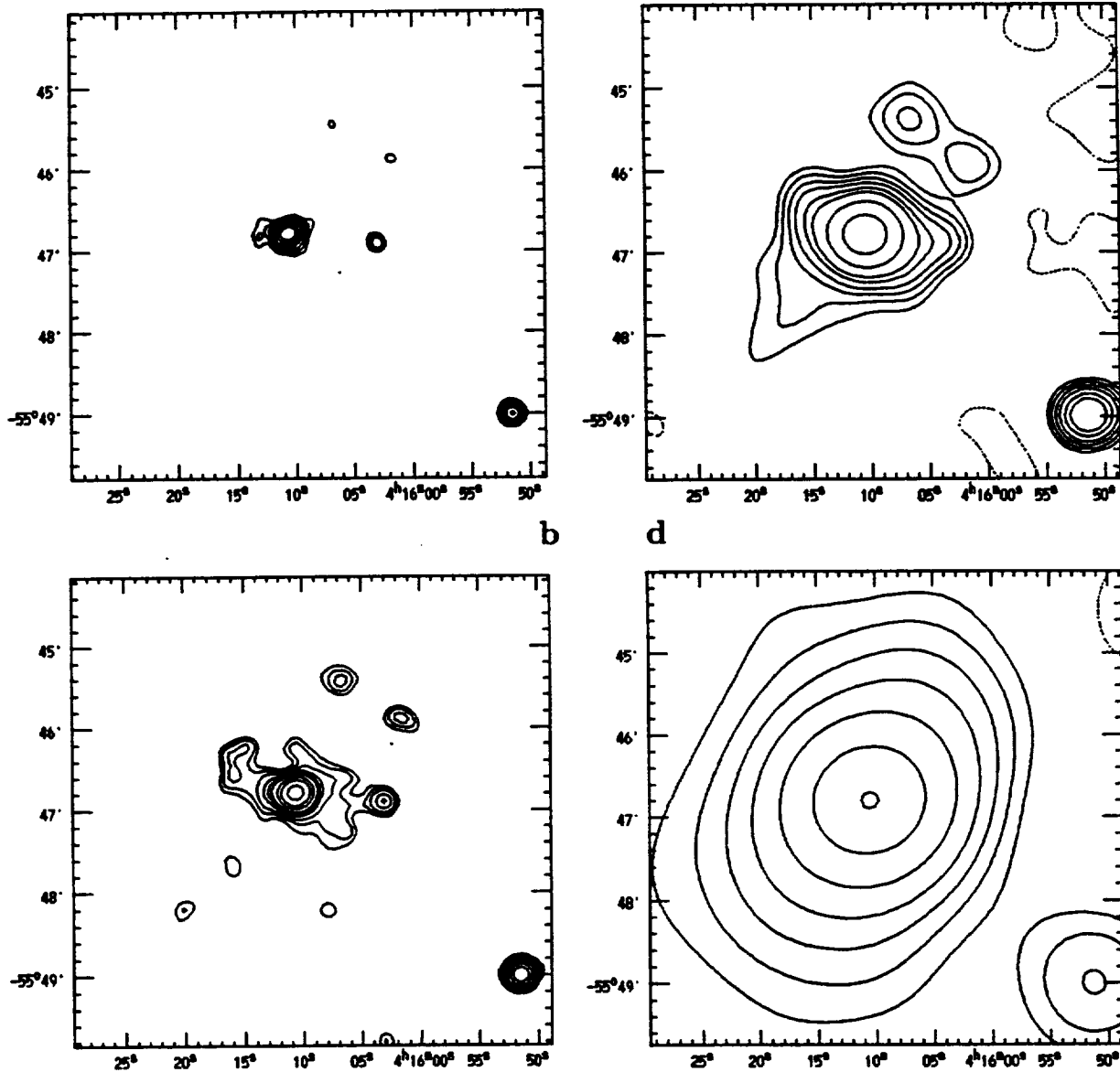
Fig. 4. Iso-intensity contour maps of NGC 1553. Images of different pixel size have been smoothed with Gaussian smoothings of different \sigma as indicated later. A locally determined background is subtracted (see text). The dashed contour indicates 0 counts/pixel. a: \sigma = 4'' , from an image with a pixel size of 2'' . Contour levels are 0.45, 0.63, 0.9, 1.5, 2.8 counts/pixel; b: \sigma = 6'' , from an image with a pixel size of 3'' . Contour levels are 0.39 0.5 0.63 0.86 1.05 1.25 1.8 2.5 4 counts/pixel; c and d: \sigma = 16'' and \sigma = 40'' respectively, from an image with a pixel size of 4'' . Contours at 0.33 0.41 0.50 0.6 0.75 0.9 1.3 2 2.8 counts/pixel and 0.13 0.18 0.24 0.32 0.45 0.65 0.85 counts/pixel respectively.
