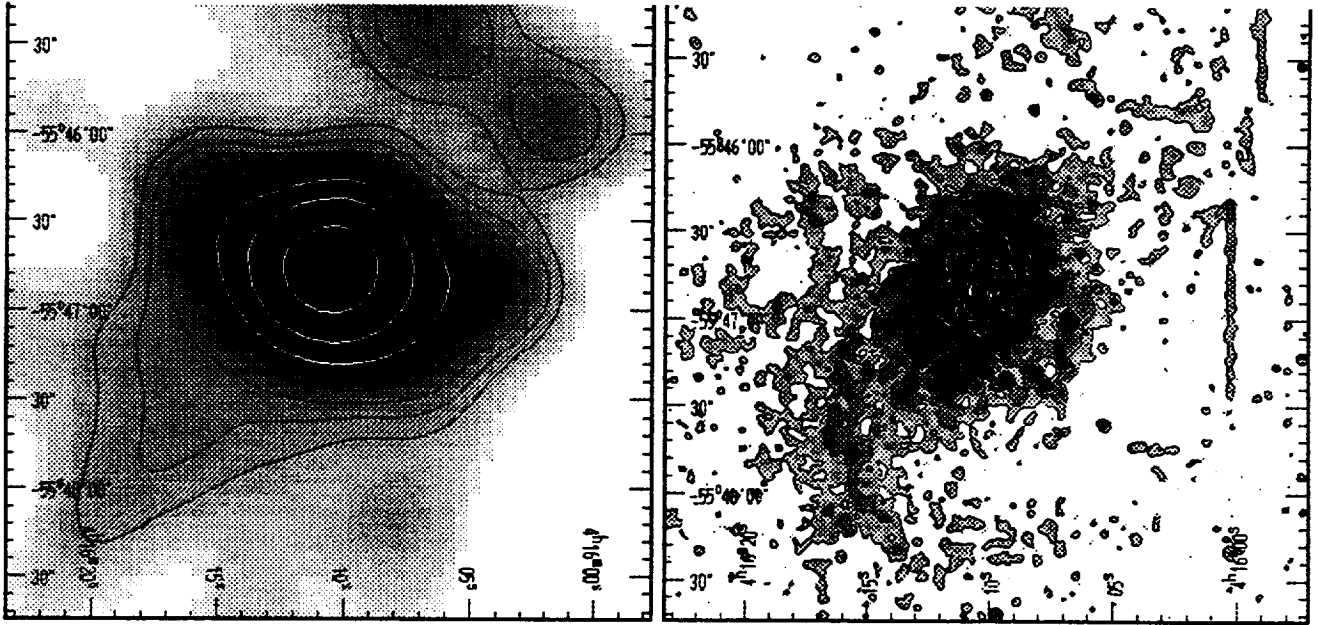
Fig. 11. Comparison between the H \alpha and X-ray morphologies for NGC 1553. The X-ray data (left) are on the same scale as the H \alpha data (right) from di Serego et al (in preparation). The celestial coordinates of the H \alpha map have been assigned a posteriori without proper absolute calibration (the peak position was assigned the RC3 coordinates of the nucleus of NGC 1553). A Gaussian smoothing with \sigma = 2.5 pixel ( \sim 1'' ) is applied to the raw data to enhance the low surface brightness features.
