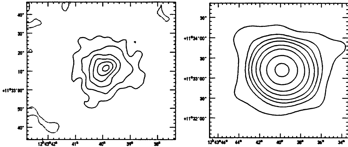
Fig. 5. As in Fig. 4 for NGC 4649. The scale in a is \sim 1/3 that in b. a: \sigma = 2'' , from an image with a pixel size of 2'' . Contours at 0.3 0.6 0.9 1.4 1.8 2.2 counts/pixel; b: \sigma = 15'' , from an image with a pixel size of 3'' . Contours at 0.2 0.3 0.4 0.6 0.9 1.3 2.3 3.7 counts/pixel.
