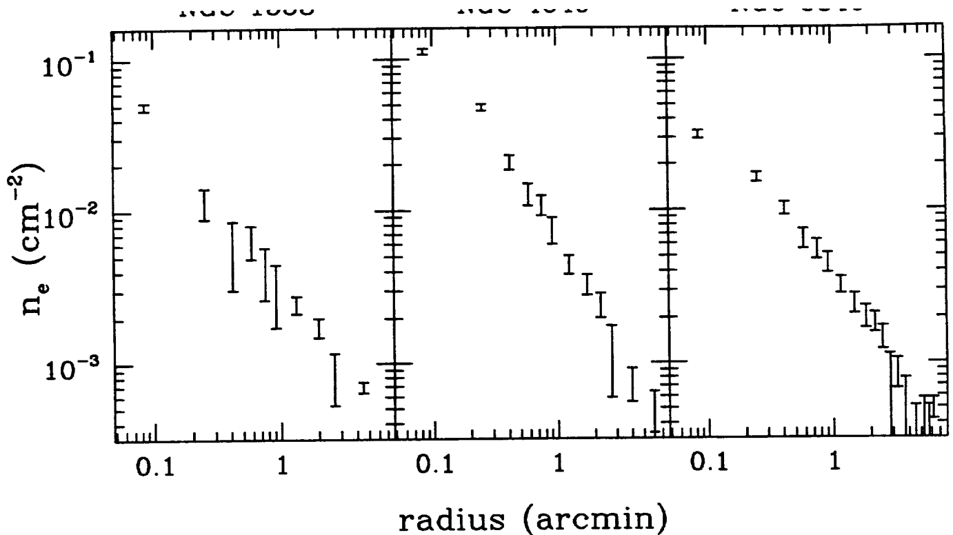
Fig. 10. Density profiles derived from the average surface brightness deprojected under the assumption of spherical symmetry. Central densities have been derived without taking into account the effects of the PSF.
