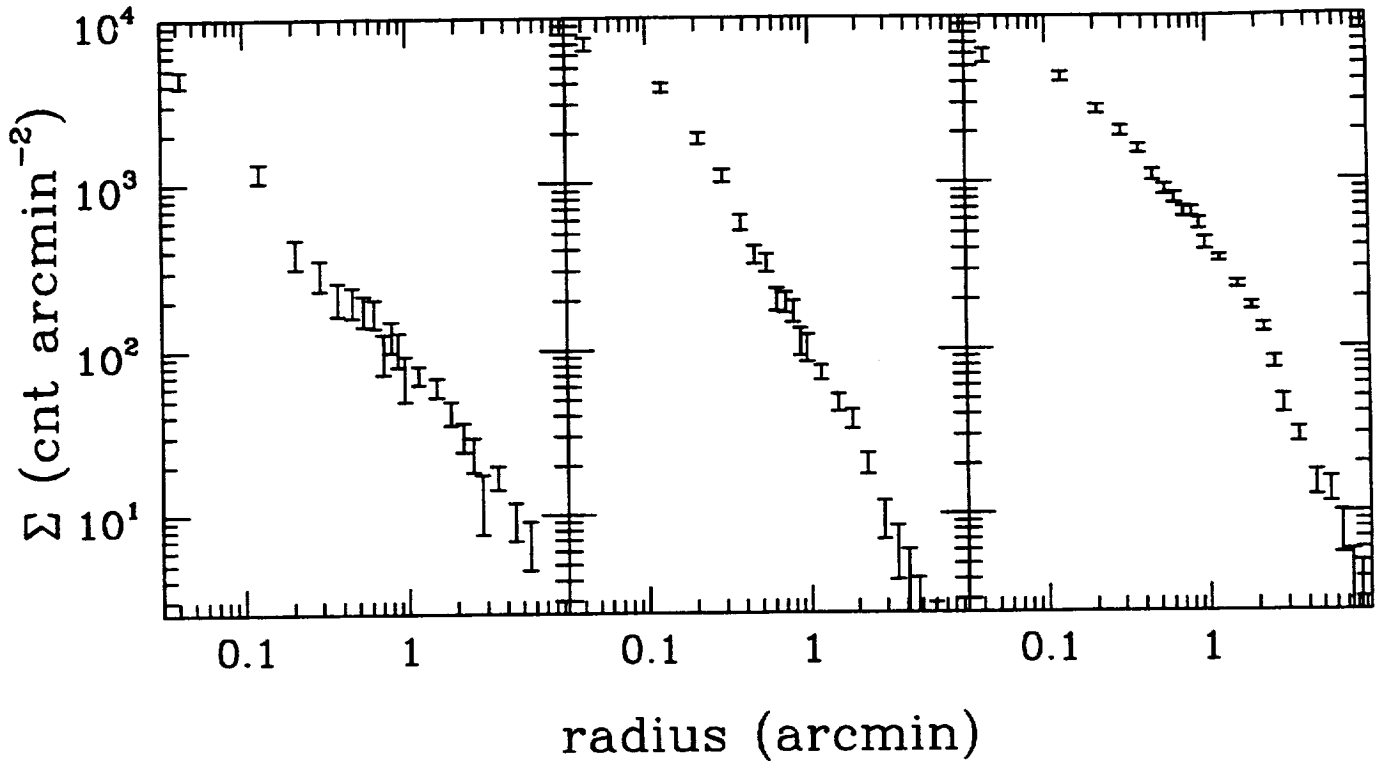
Fig. 8. Radial distribution of the net surface brightness emission from the sample galaxies
