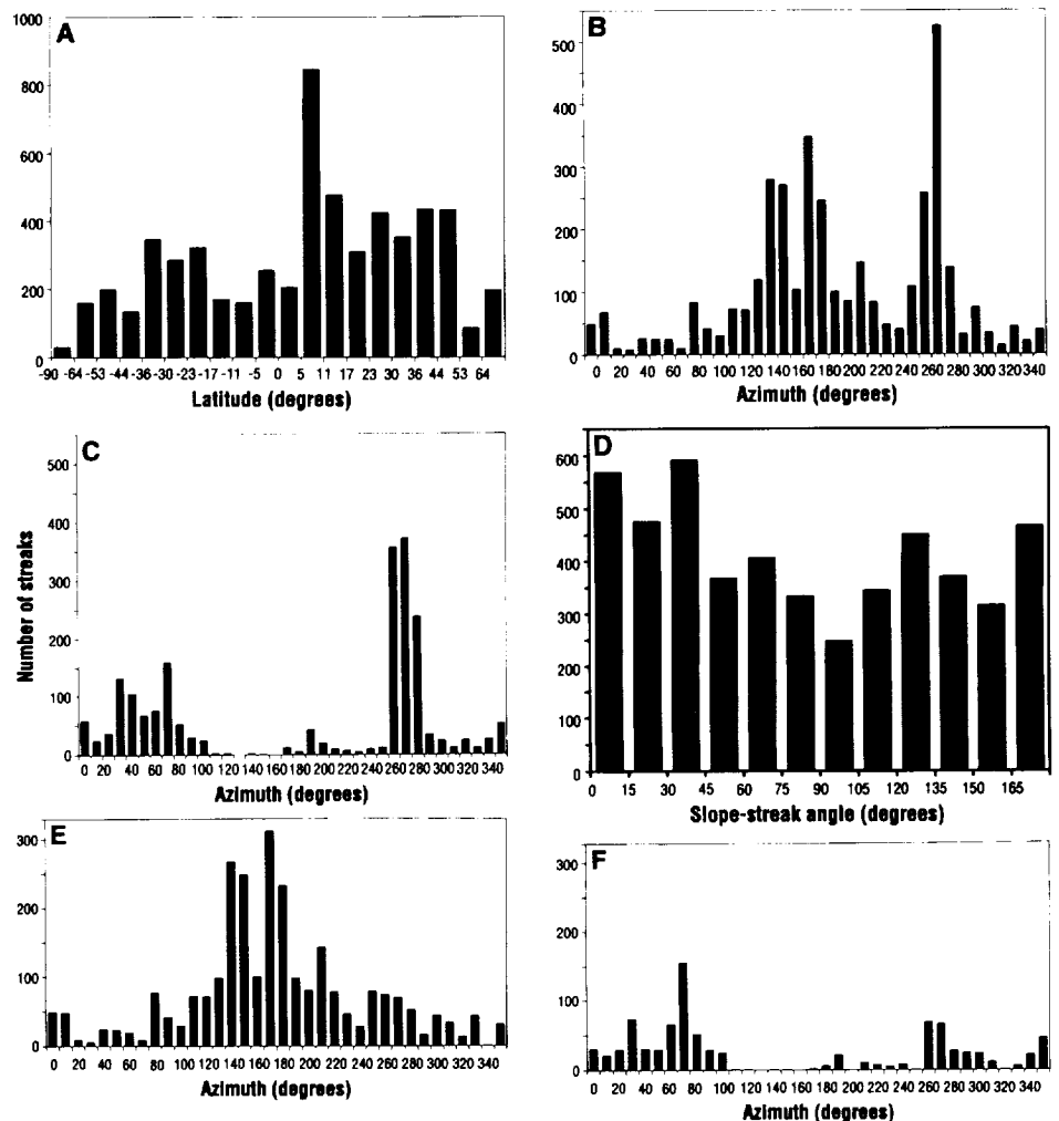
Fig. 2. (A) Histogram of venusian wind streaks in bands of equal area latitude. (B) Azimuths of all wind streaks in the global data base for the northern hemisphere, with north at 0°. (C) Azimuths of all wind streaks in the global database for the southern hemisphere, with north at 0°. (D) Distribution of wind streak orientations with respect to local slope, showing that streaks occur randomly with regard to slope. The downslope is at 0° and the upslope is at 180°. Angle is the difference in degrees between downslope azimuth and streak azimuth. (E) Azimuths of subset of database (3666 streaks) in which Type P wind streaks that may have formed in response to transient events have been deleted (northern hemisphere). North is at 0°. (F) Azimuths of subset of data with deletion of Type P wind streaks that may have formed in response to transient events (southern hemisphere). North is at 0°.
