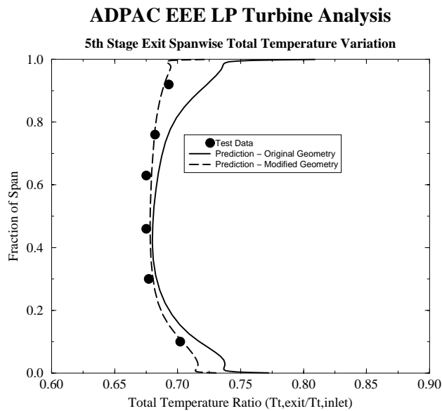
Fig. 10 Comparison of predicted and experimental spanwise variation in fifth stage exit total temperature distributions for EEE LP turbine analyses with variations in first vane reset and endwall modeling.
