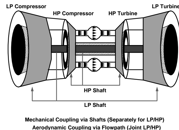
Fig. 21 Illustration of aerodynamic/mechanical balance required for single-spool and twin-spool gas turbine engines.
