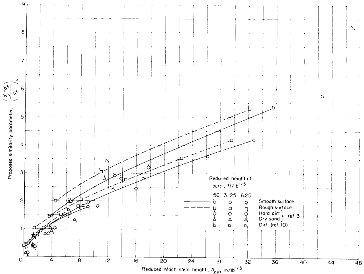
FIGURE 21. Approximate similarity of path of triple-point rise with height of burst based on \left(\frac{d_v-d_e}{d_e}\right)_o .
