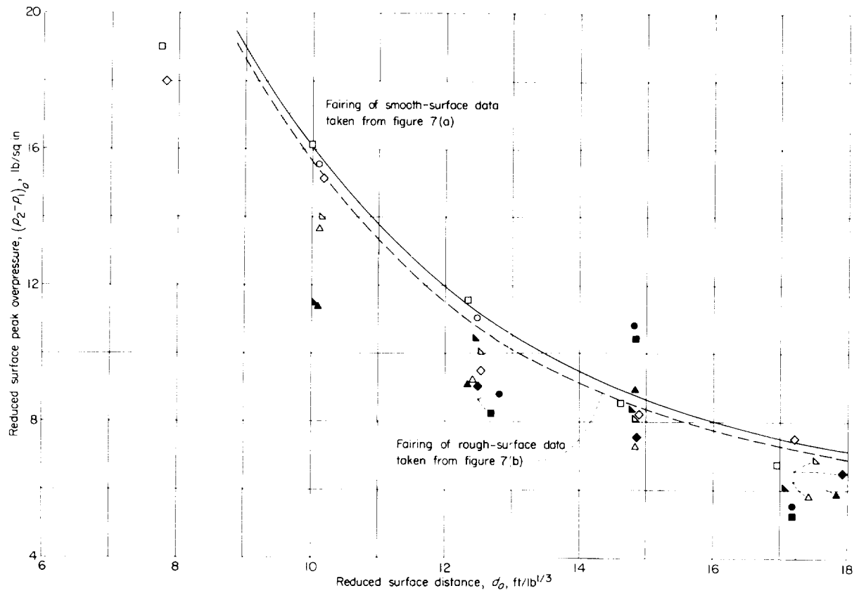
FIGURE 11.—Comparison of surface peak overpressures obtained from pressure pickups and fairing of schlieren data for a reduced height of burst of 6.25 ft/lb 1/3 . Solid symbols represent smooth-surface data; open symbols represent rough-surface data; each type of symbol represents a separate test.
