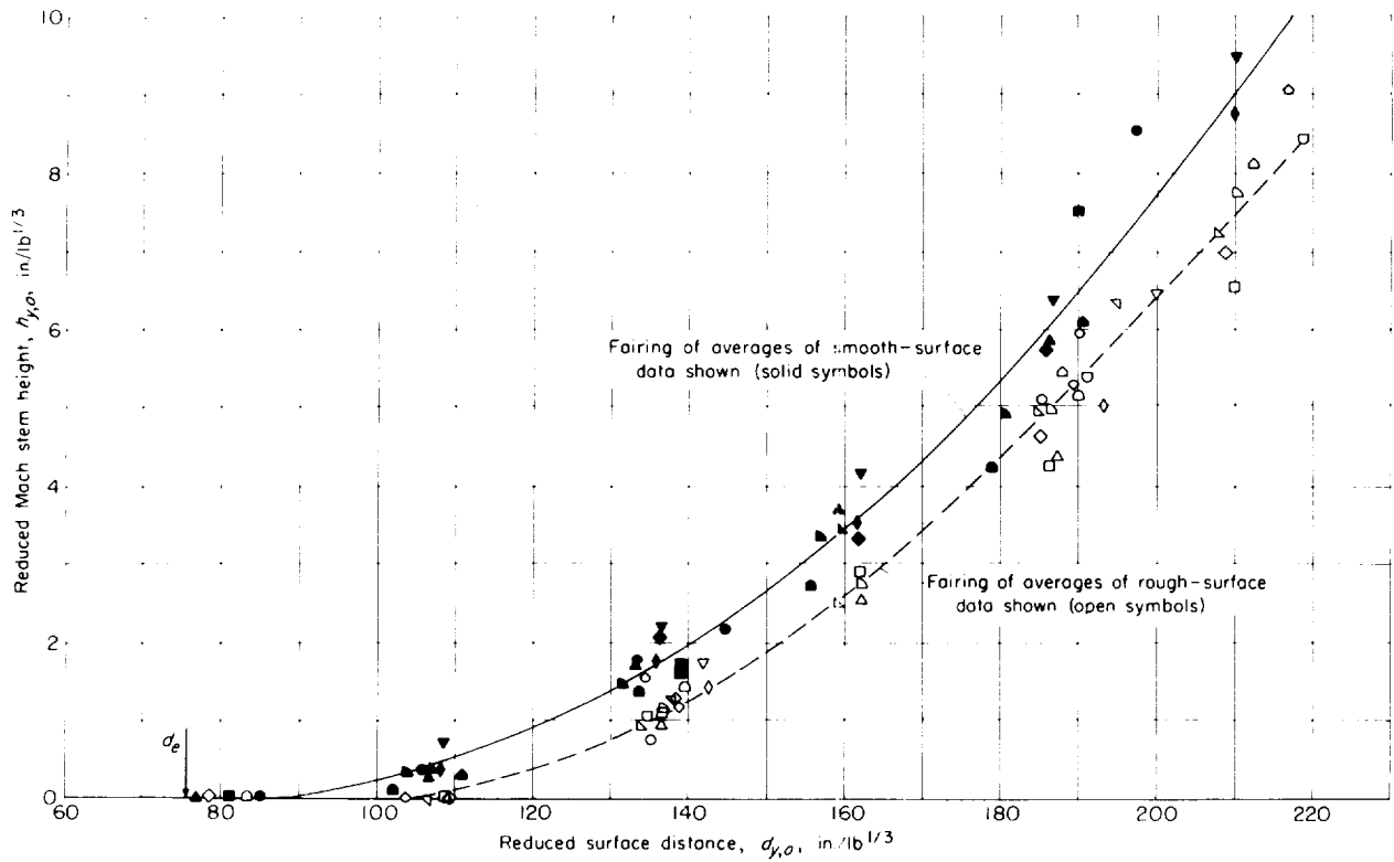
FIGURE 15. Comparison of Mach stem growth over smooth and rough surfaces for a reduced height of burst of 6.25 ft/lb 1/3 . Each type of symbol represents a separate test.
