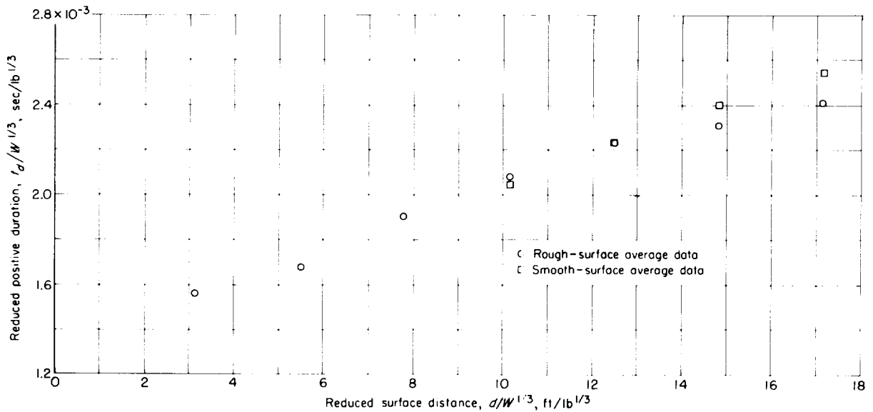
FIGURE 12.—Comparison of duration of positive overpressures of smooth- and rough-surface data for the reduced height of burst of 6.25 ft/lb 1/3 . Data are not reduced to standard atmospheric conditions.
