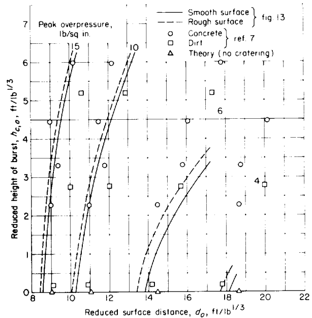
FIGURE 14.—Comparison of height-of-burst curves of smooth and rough surfaces with reference data.
