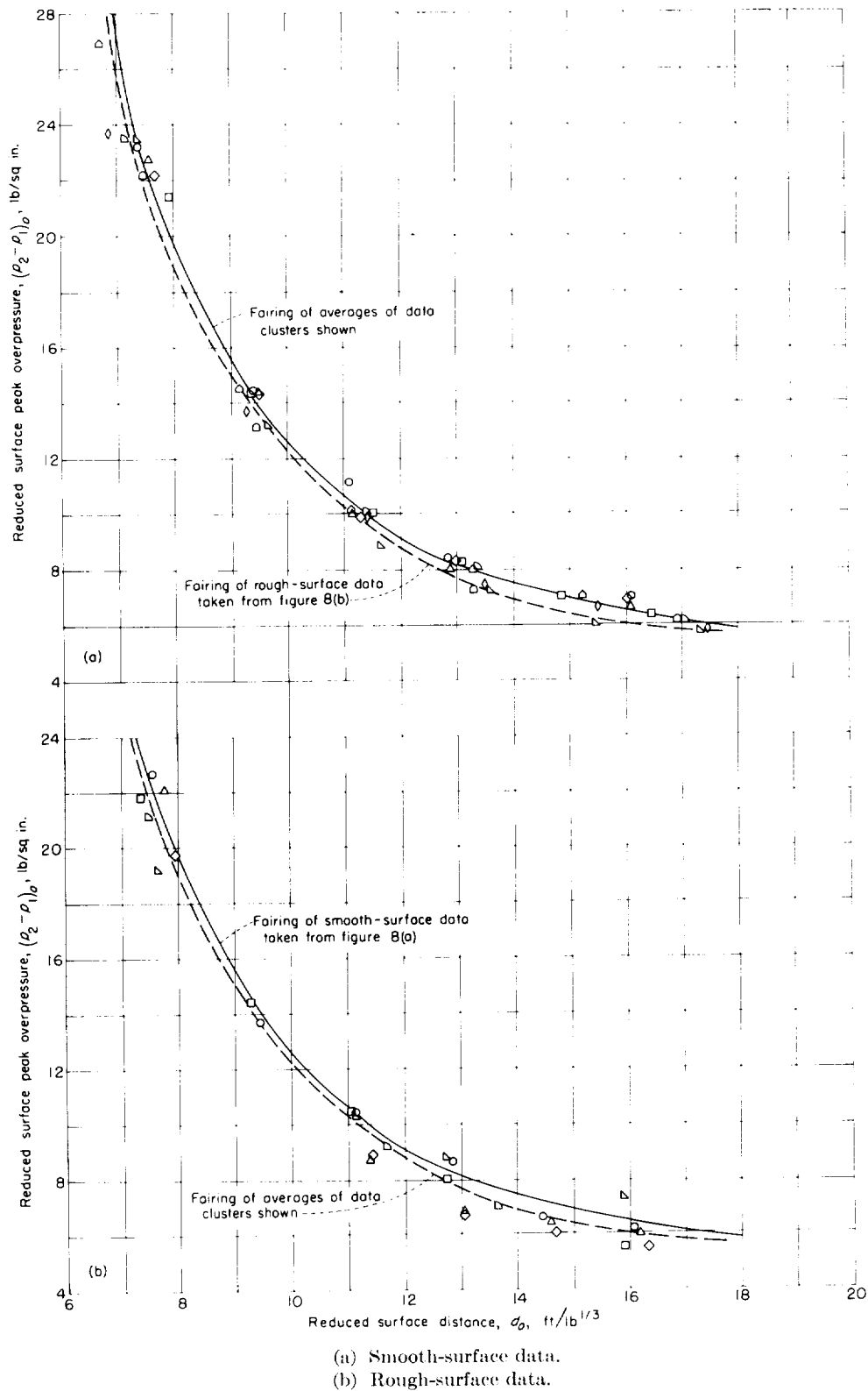
FIGURE 8. Surface peak overpressures obtained from schlieren data for a reduced height of burst of 3.125 \text{ ft/lb}^{1/3} (1-foot actual charge height). Each type of symbol represents a separate test.
