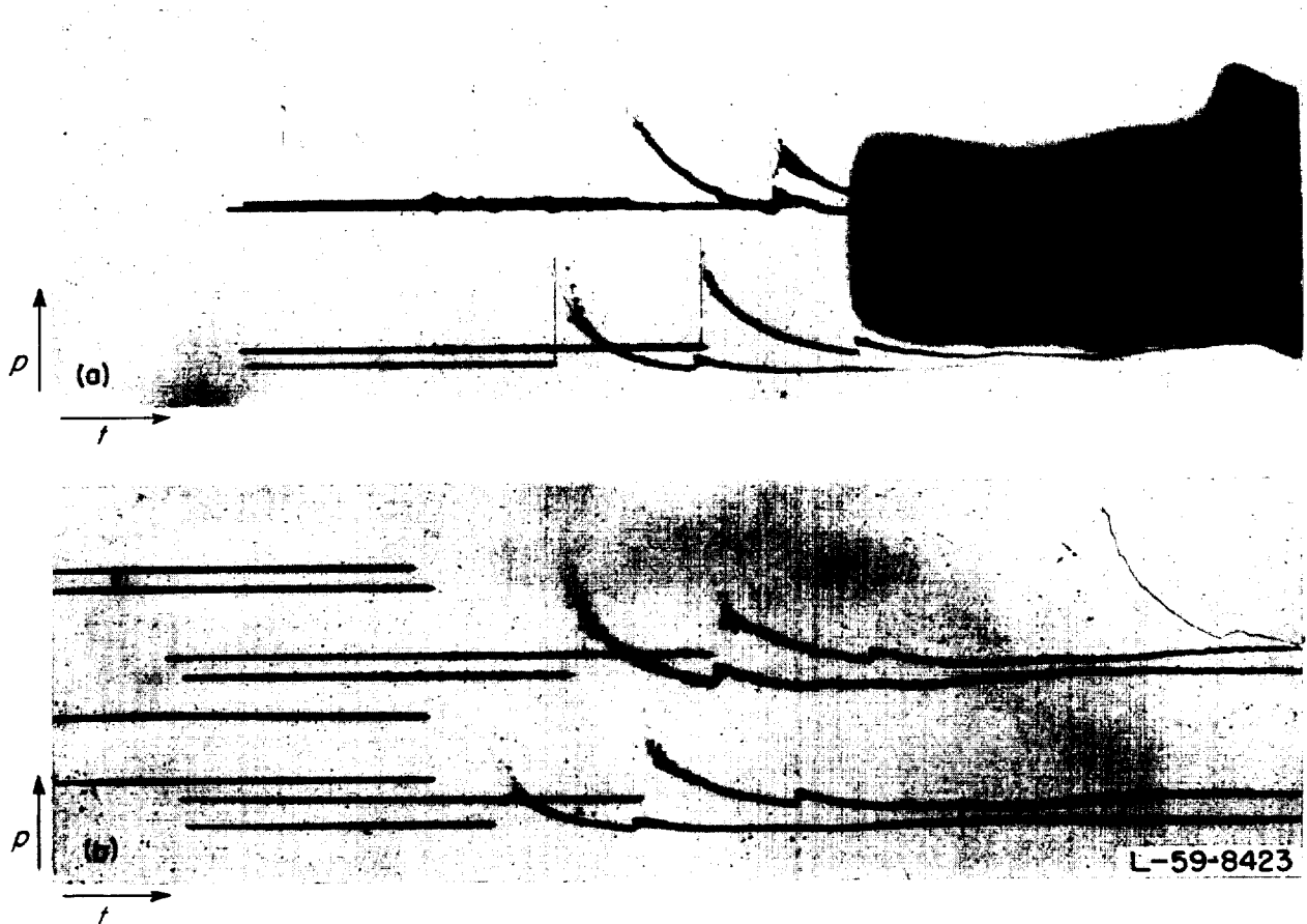
(a) Drum-camera pressure records for smooth surface for a 2-foot charge height. (b) Drum-camera pressure records for rough surface for a 2-foot charge height.
