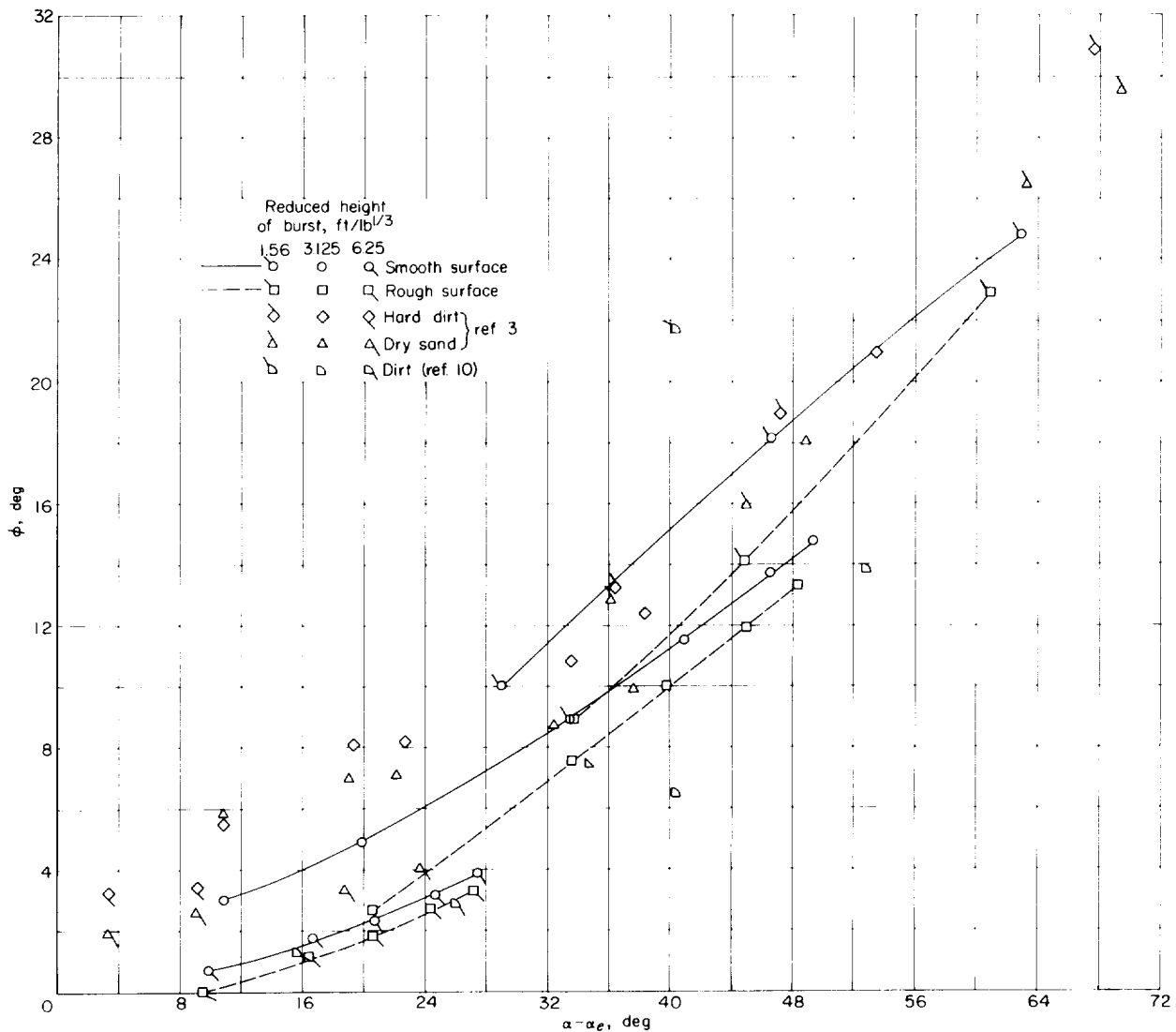
FIGURE 20. - Path of triple point based on height-of-burst similarity parameter in reference 10.
