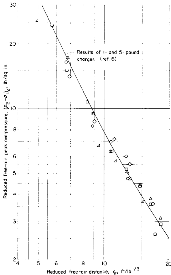
FIGURE 6.—Free-air pressures obtained from schlieren data. Each type of symbol represents a separate test.
