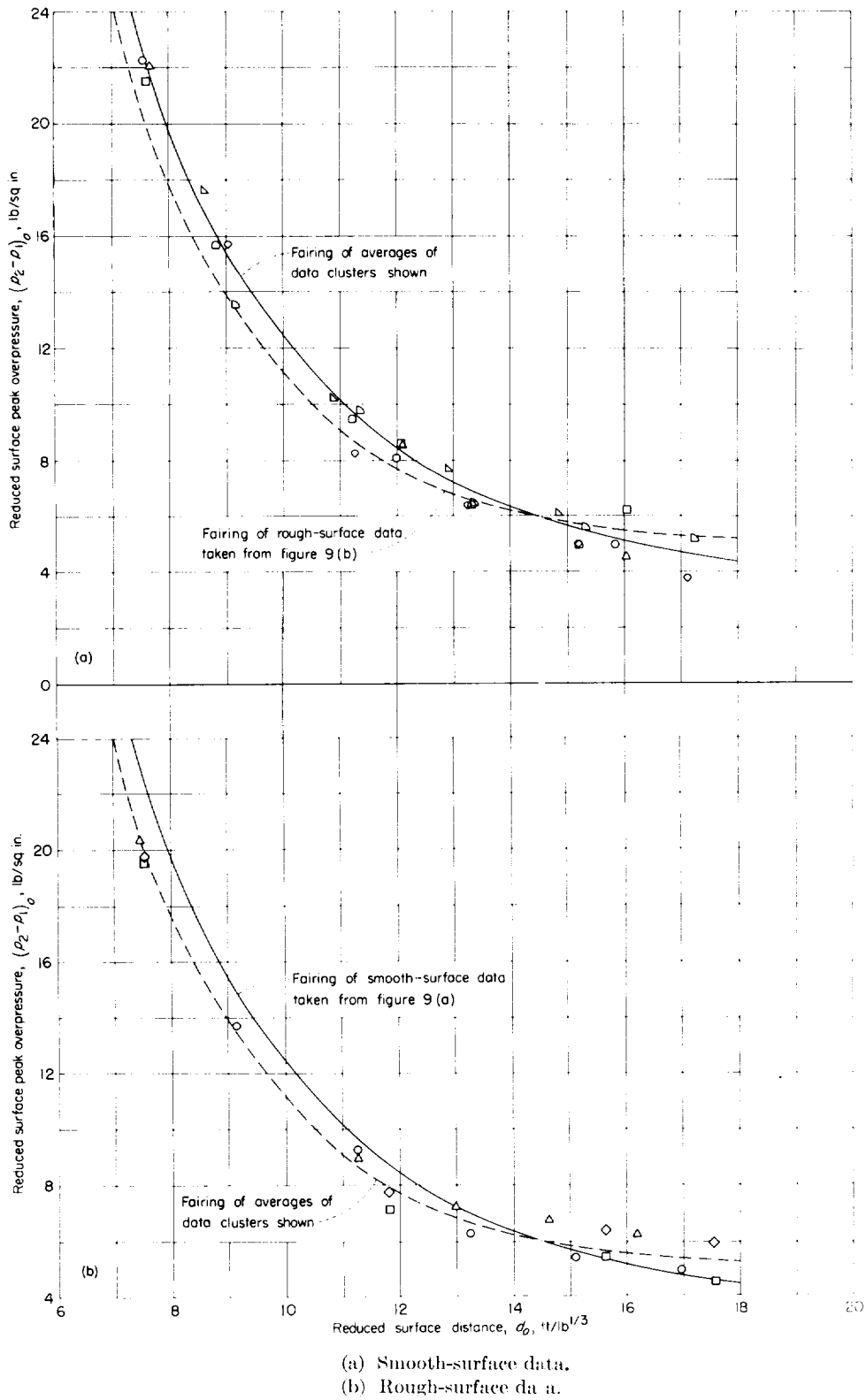
FIGURE 9.- Surface peak overpressures obtained from schlieren data for a reduced height of burst of 1.56 (t/b)^{1/3} (6-inch actual charge height). Each type of symbol represents a separate test.
