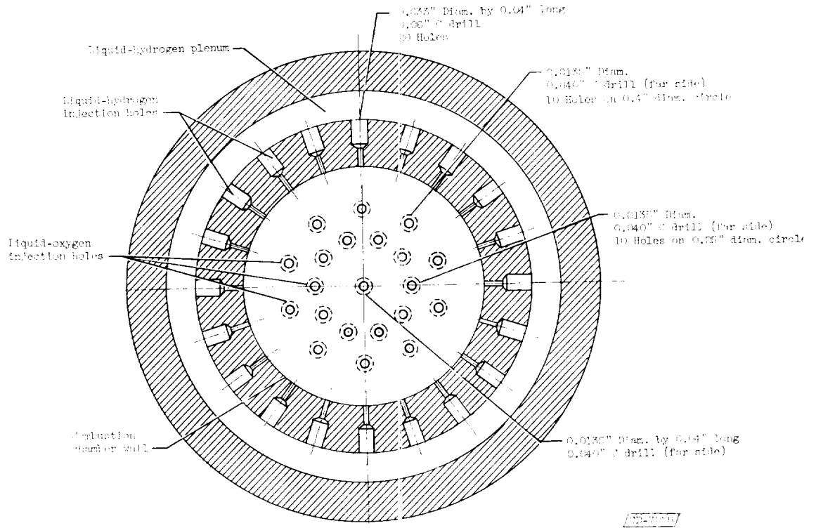
Figure 2. Detector details.
