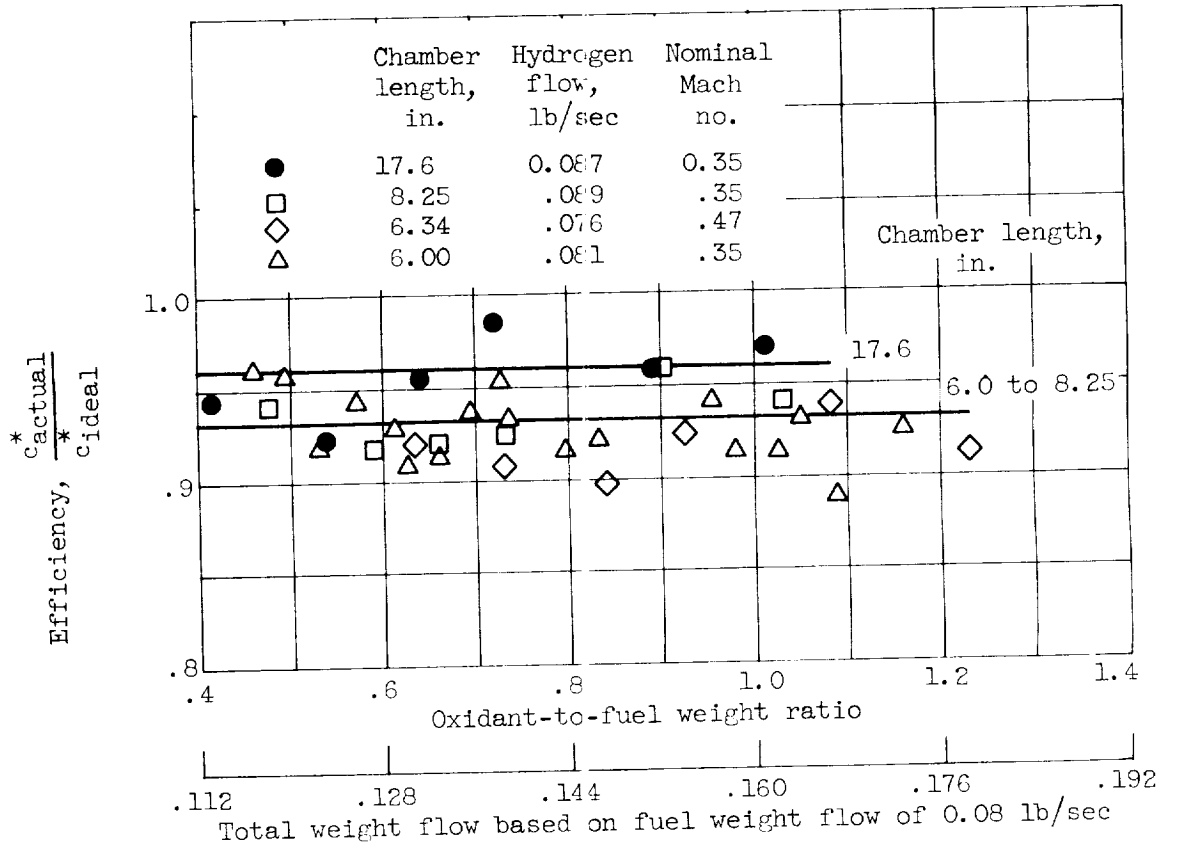
(b) Variation of combustion efficiency with oxidant-to-fuel weight ratio.
