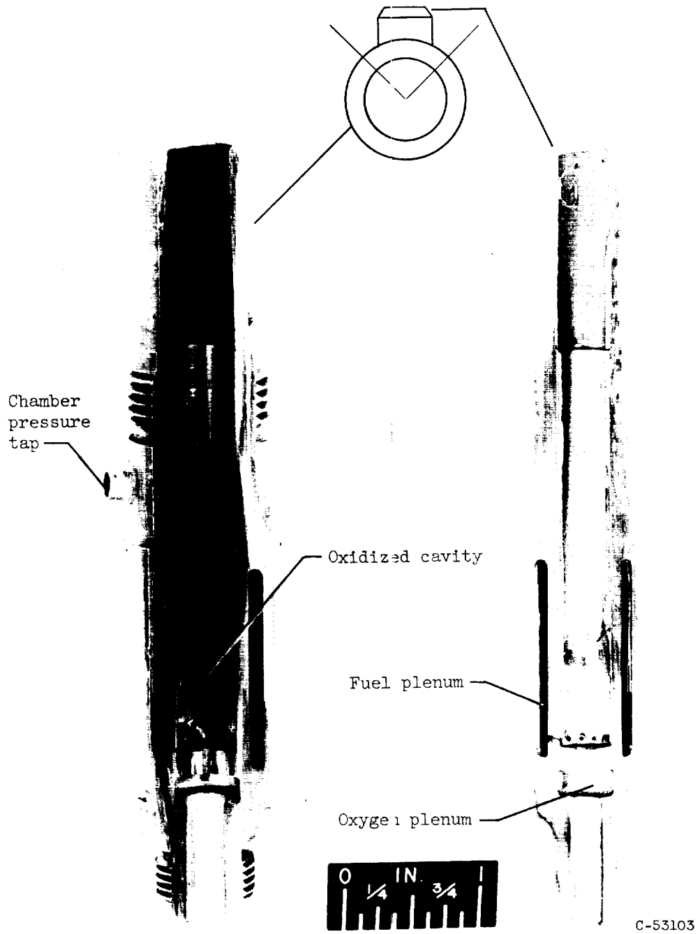
(b) Gas-generator burnout caused by contact of liquid oxygen with wall.
