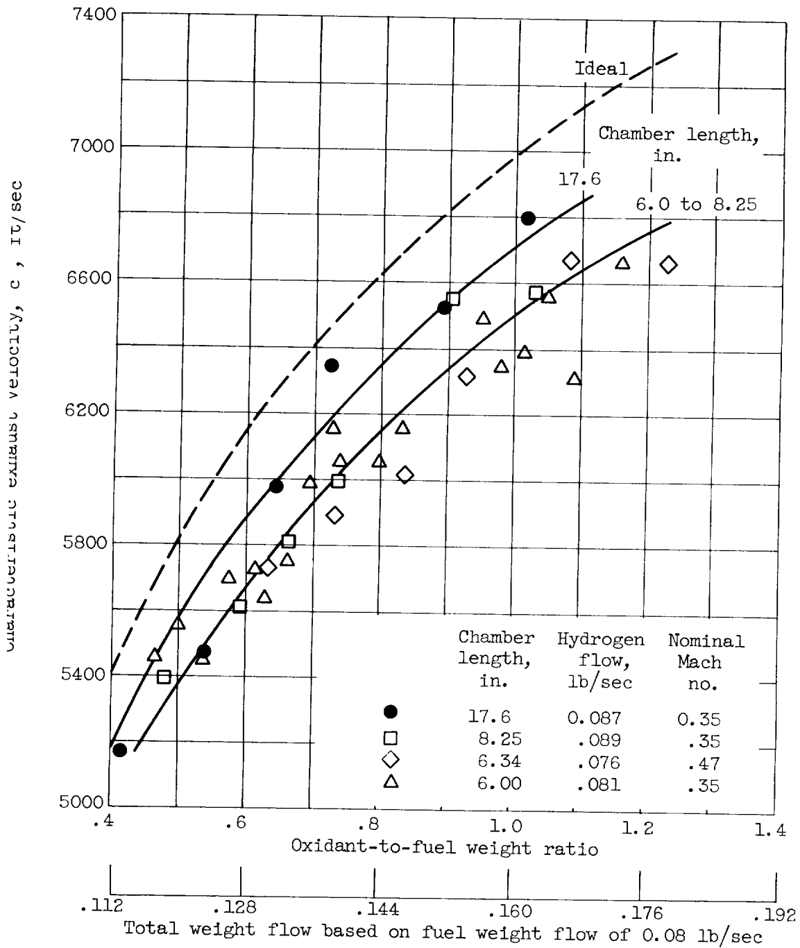
(a) Variation of characteristic exhaust velocity with oxidant-to-fuel weight ratio.
