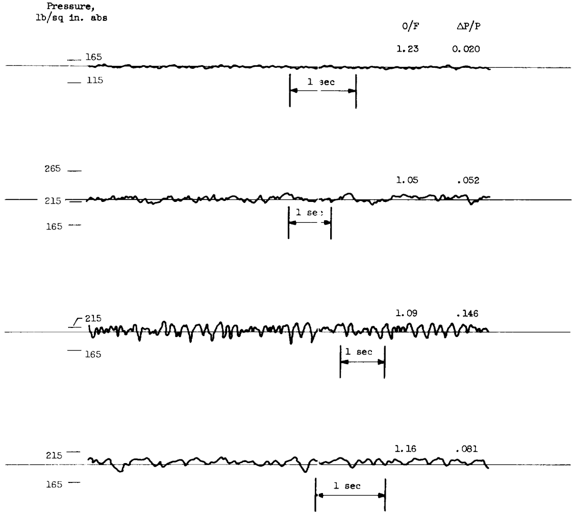
(a) Four runs at high oxidant-to-fuel weight ratios.
