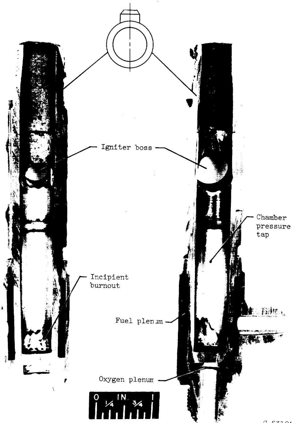
Figure 7. - Gas generator after 24 minutes operation with ten starts and stops.
