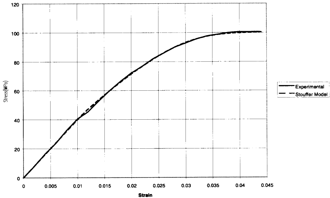
Figure 12: Model Correlations for PEEK at Tensile Strain Rate of 1E-04 /sec.
