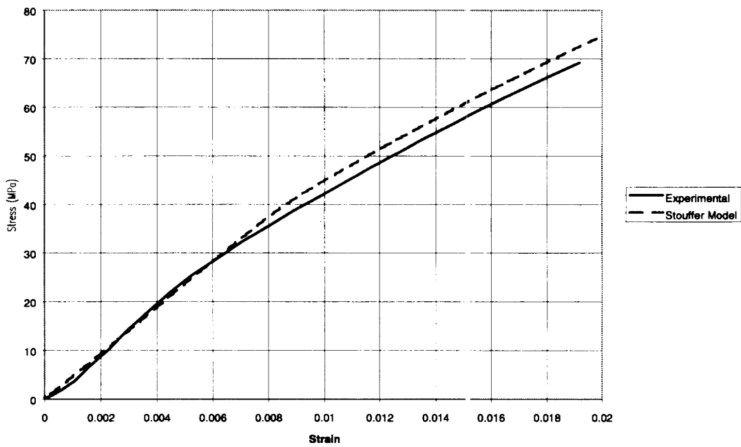
Figure 10: Model Correlations for 977-2 Resin at Tensile Strain Rate of 0.1 /sec.
