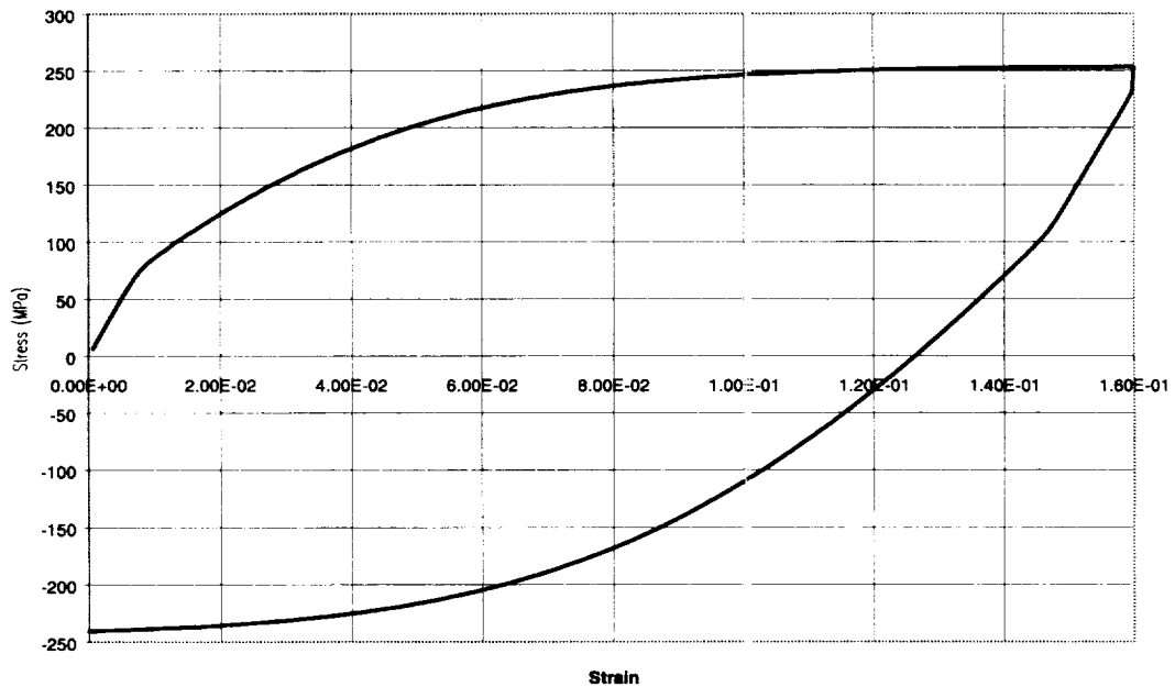
High Rate Compression: 977-2 Resin, Strain Rate=500 /sec., Stouffer Model, Load-Unload Prediction
