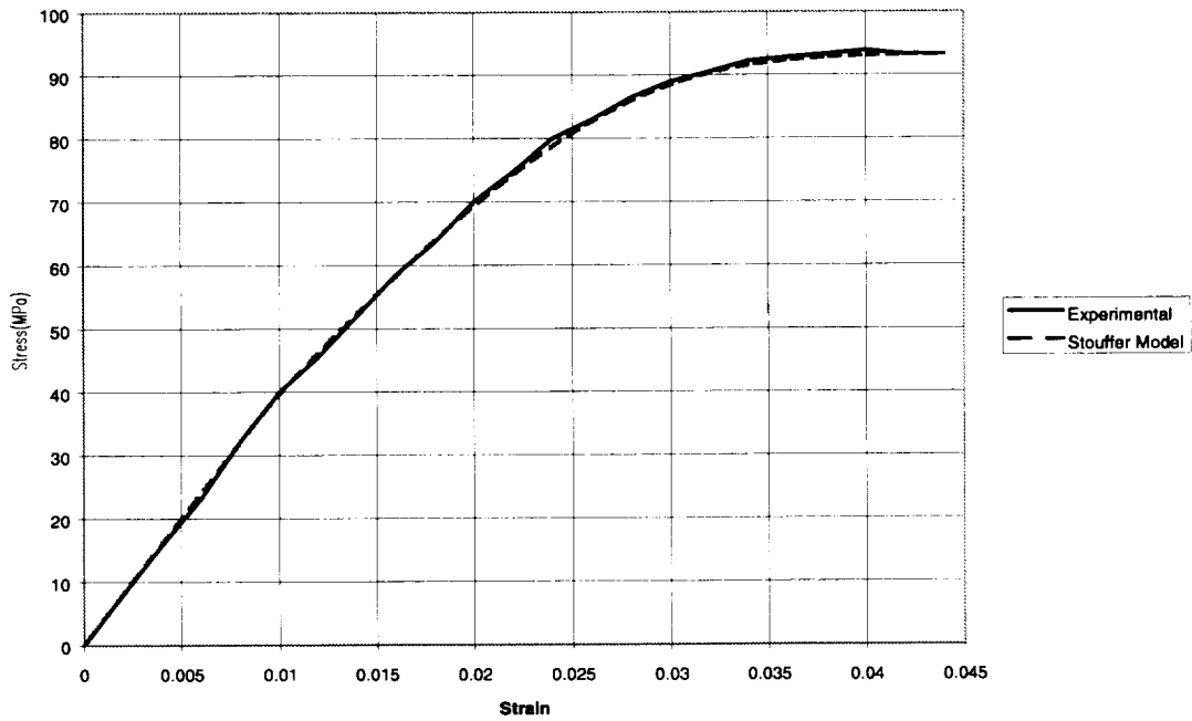
Figure 11: Model Correlations for PEEK at Tensile Strain Rate of 1E-06 /sec.
