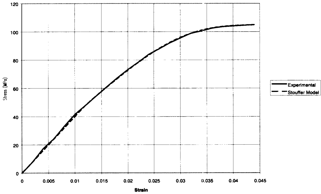
Figure 13: Model Correlations for PEEK at Tensile Strain Rate of 1E-03 /sec.
