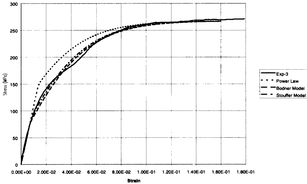
Figure 5: Model Correlations for 977-2 Resin at Compressive Strain Rate of 1500 /sec.
