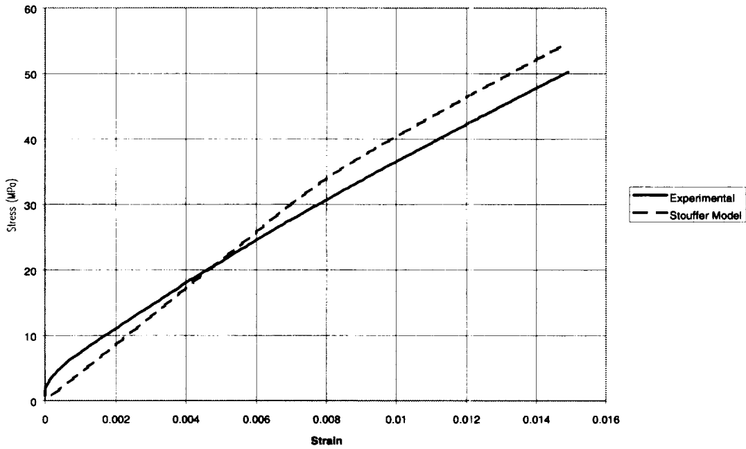
Figure 9: Model Correlations for 977-2 Resin at Tensile Strain Rate of 0.01 /sec.
