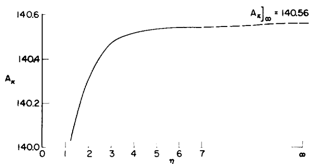
FIGURE 12.—Convergence of A_x for \text{MoO}_3 .
