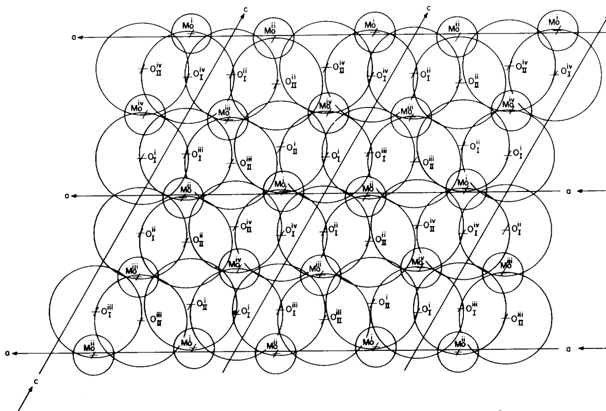
FIGURE 6.— Projection of \text{MoO}_2 model on ac -plane. 1 inch = 2 \text{ \AA} .
