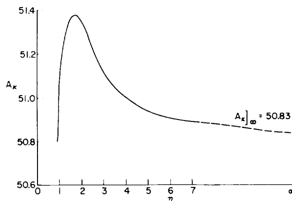
FIGURE 11.—Convergence of A_\kappa for \text{MoO}_3 .
