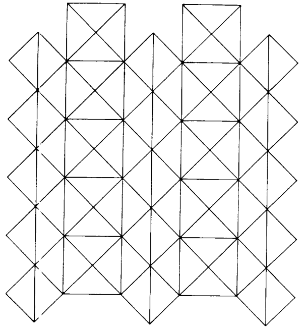
FIGURE 5.—Schematic structure of \text{MoO}_3 .
