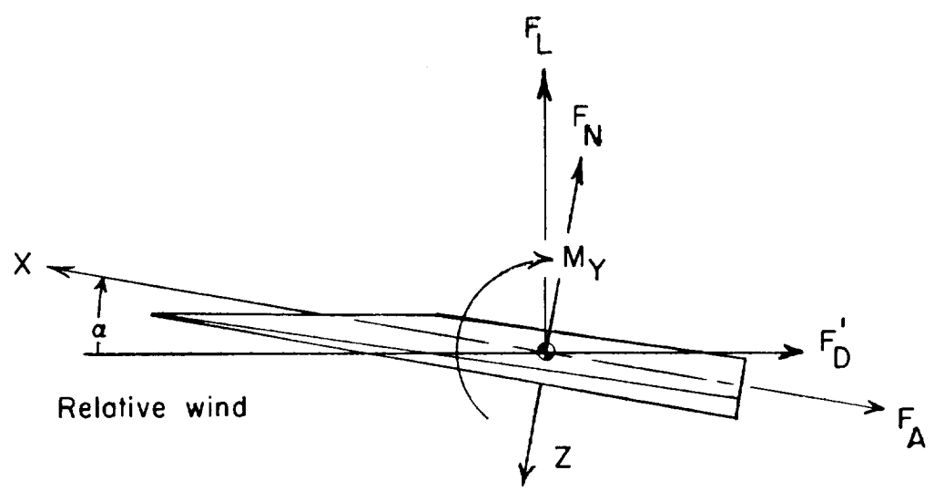
Figure 1.- Axis system. Arrows indicate positive directions.
