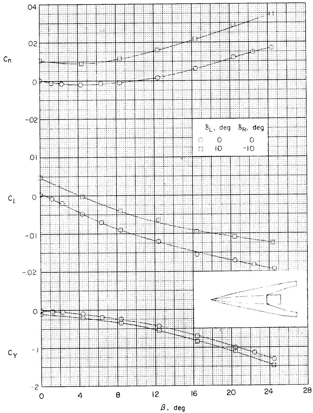
Figure 36.- Effects of deflected roll control of model 7 on the lateral aerodynamic characteristics in sideslip. \alpha = 3.4^\circ ; M = 2.01 .
