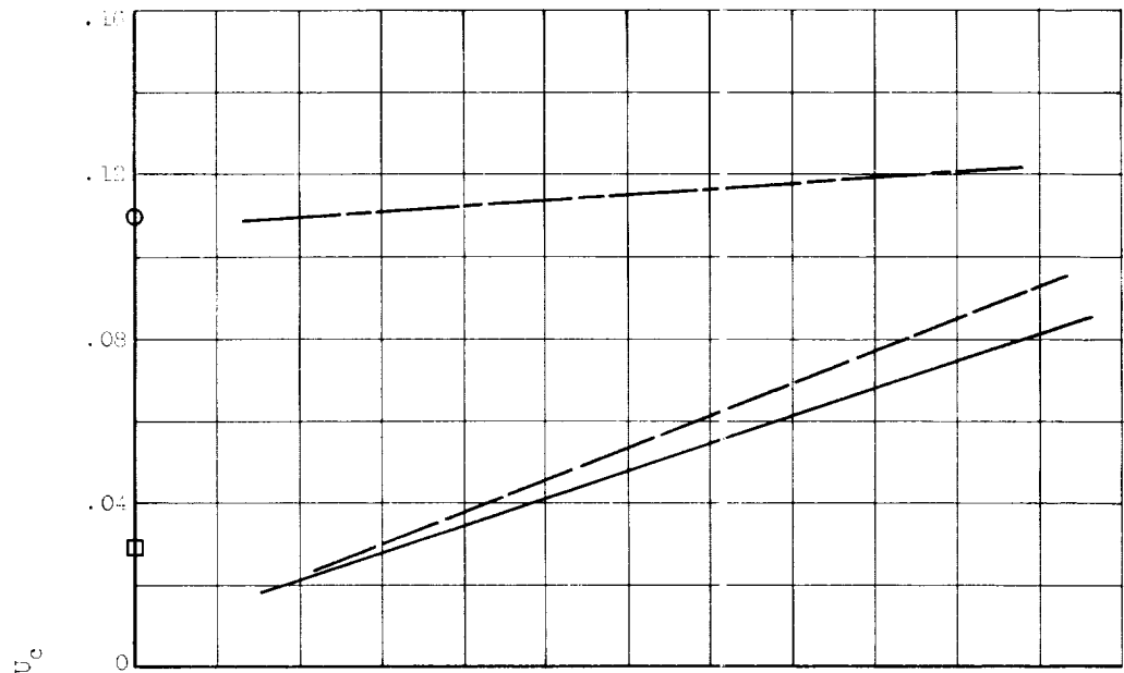
(a) x/D = 1.0 .
