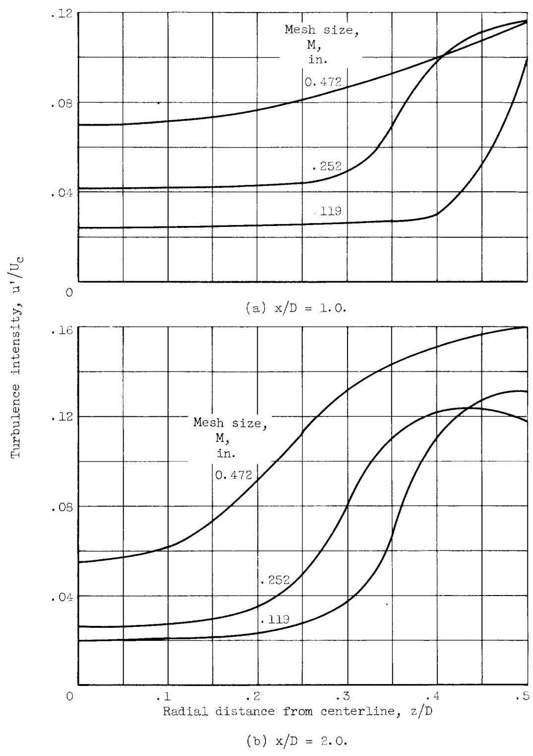
Figure 10. - Intensity of turbulence as function of mesh size and distance from nozzle exit.
