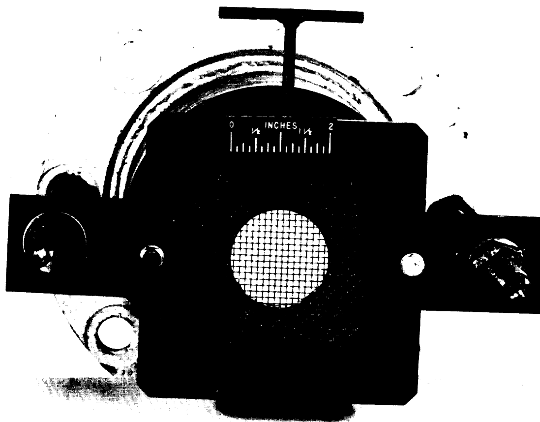
Figure 4. - Screen holder bolted to nozzle.
