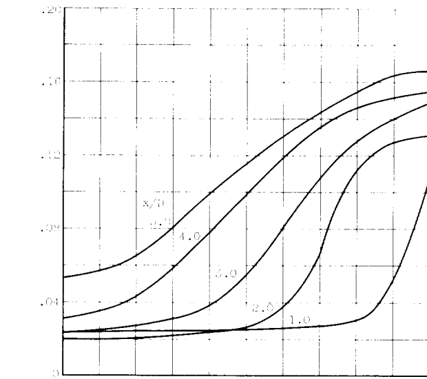
(a) Mesh size, 0.119 inch.
