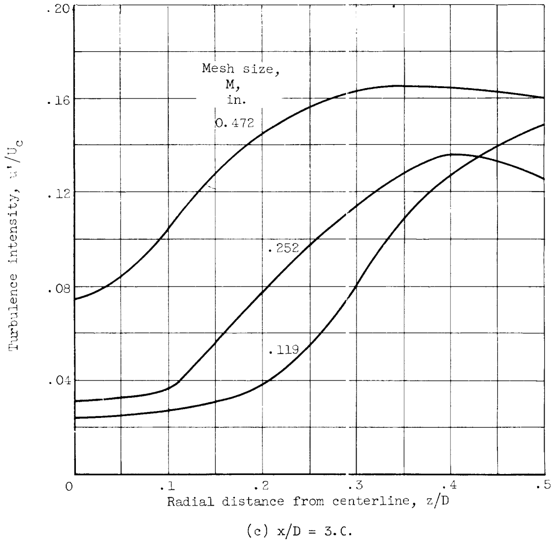
Figure 10. - Continued. Intensity of turbulence as function of mesh size and distance from nozzle exit.
