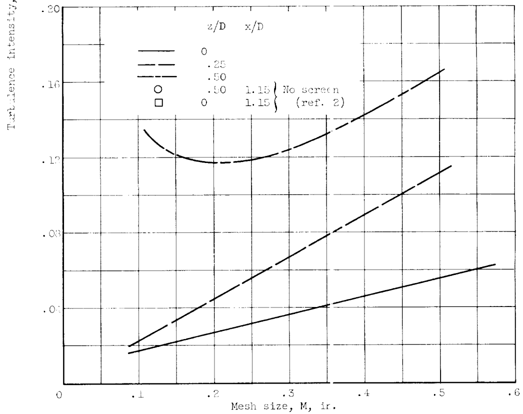
(b) x/D = 2.0 .
