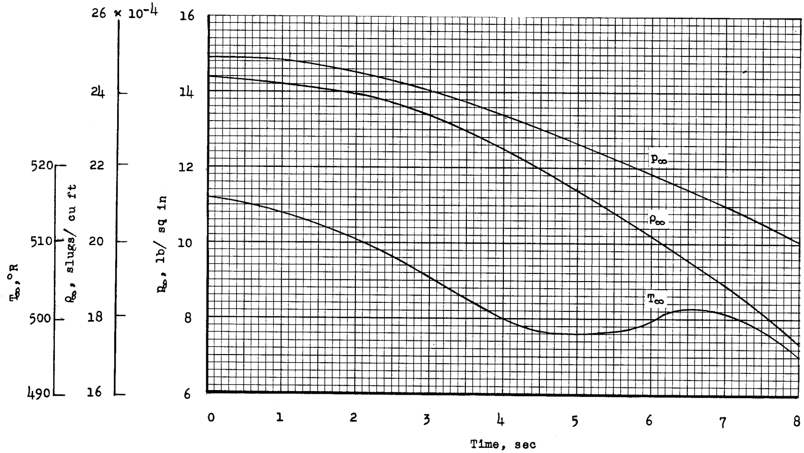
Figure 6.- Free-stream conditions related to model flight time.
