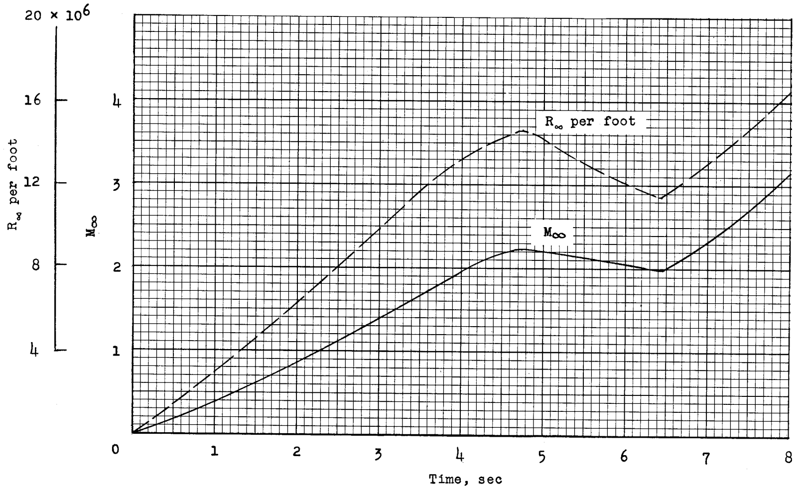
Figure 7.- Free-stream Mach number and Reynolds number per foot.
