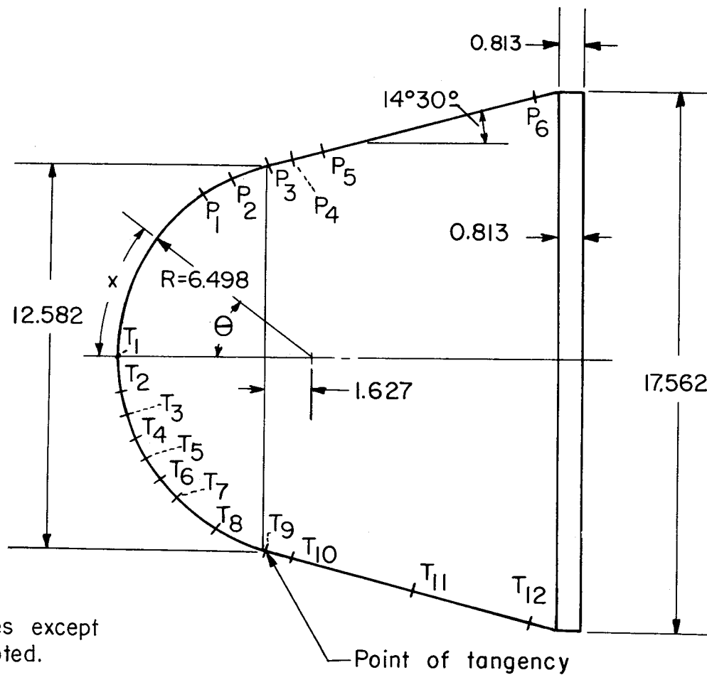
Figure 5.- Sketch of nose showing location of temperature and pressure pickup stations. (P 1 to P 6 are pressure tubes and T 1 to T 12 are thermocouples.)
