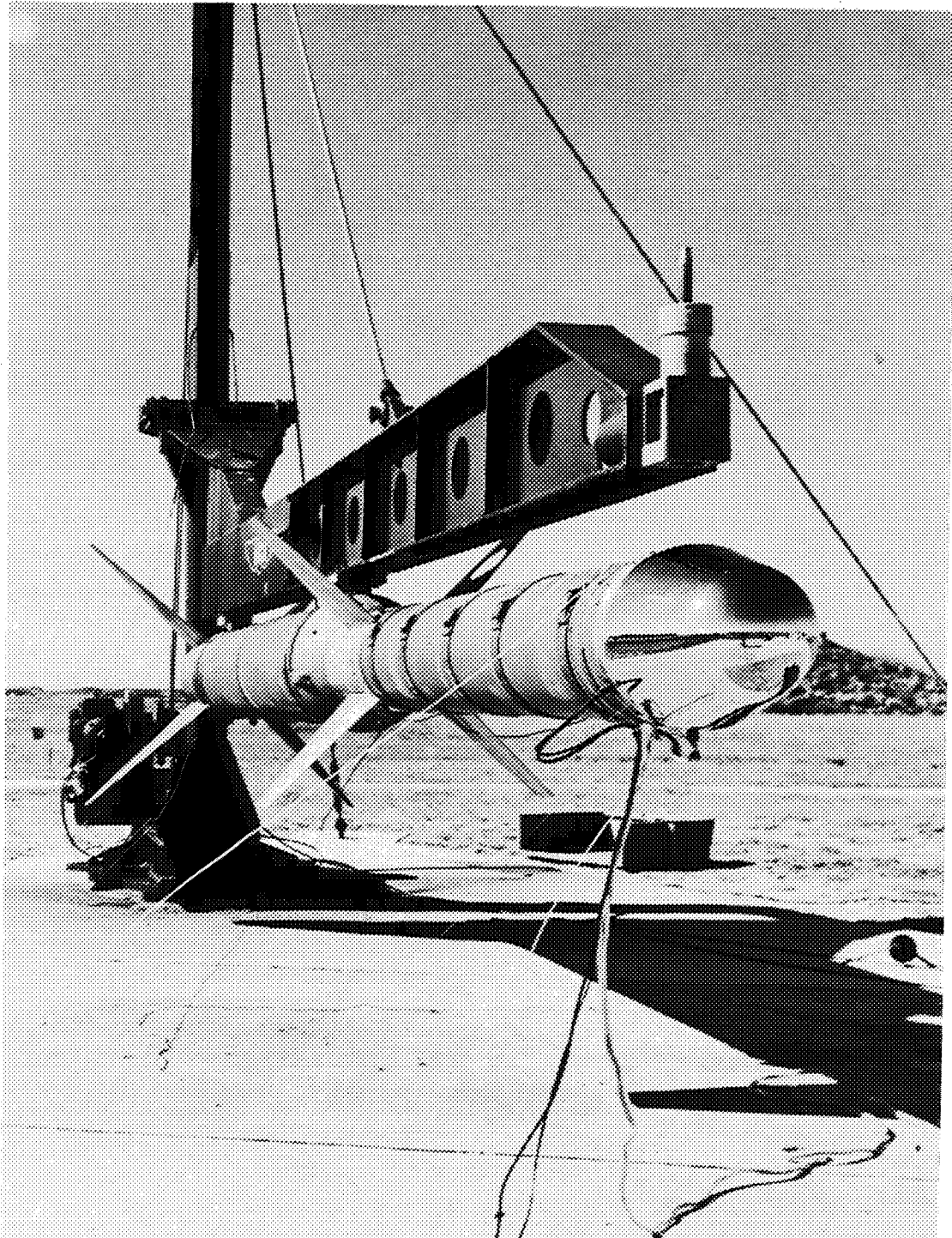
Figure 1.- Photograph of model and booster on launcher.
