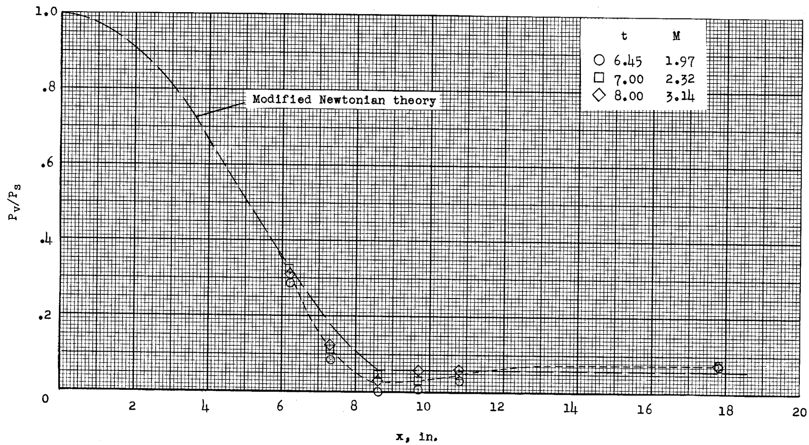
Figure 8.- Ratio of local to stagnation-point pressure coefficient.
