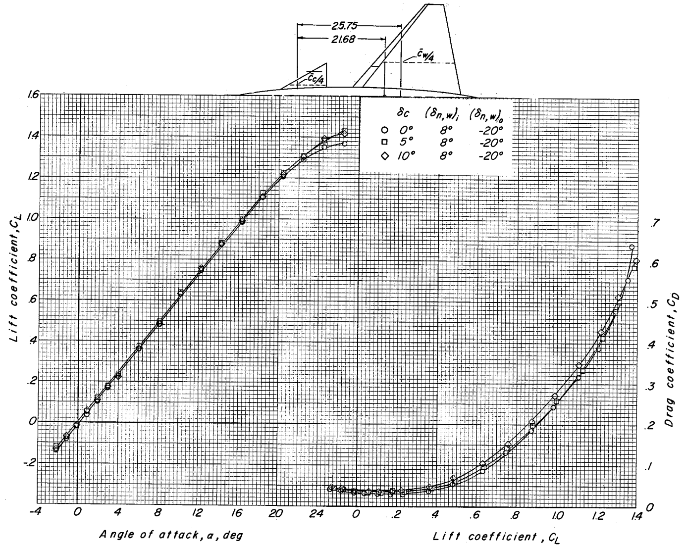
Figure 17.- Longitudinal control characteristics of the configuration having a delta canard with a fence and the wing having differentially deflected full-span leading-edge chord-extension, WBC_{2,f} .
