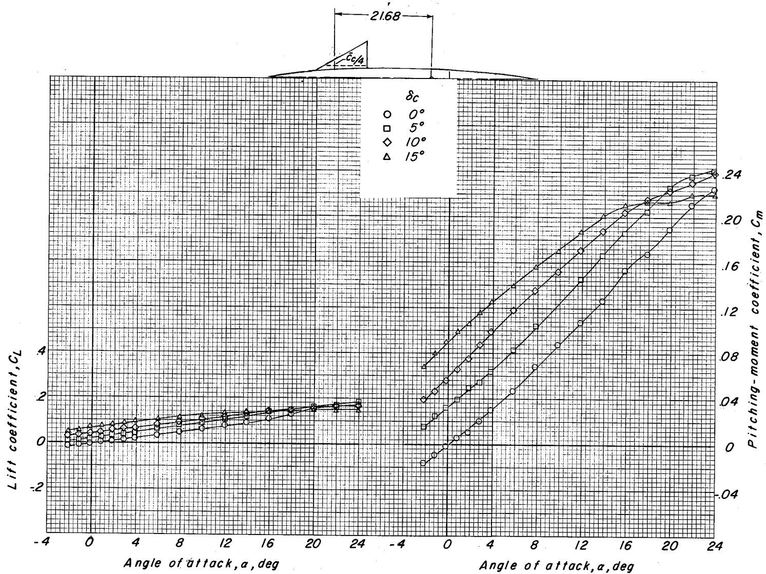
Figure 13.- Longitudinal control characteristics of the configuration having a delta canard with wing off, BC 2 .
