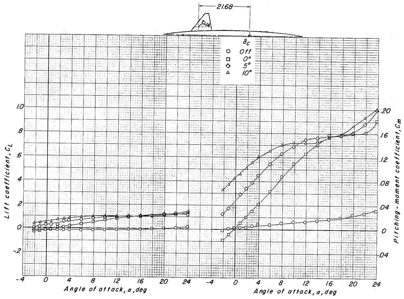
(a) Basic trapezoidal canard.
