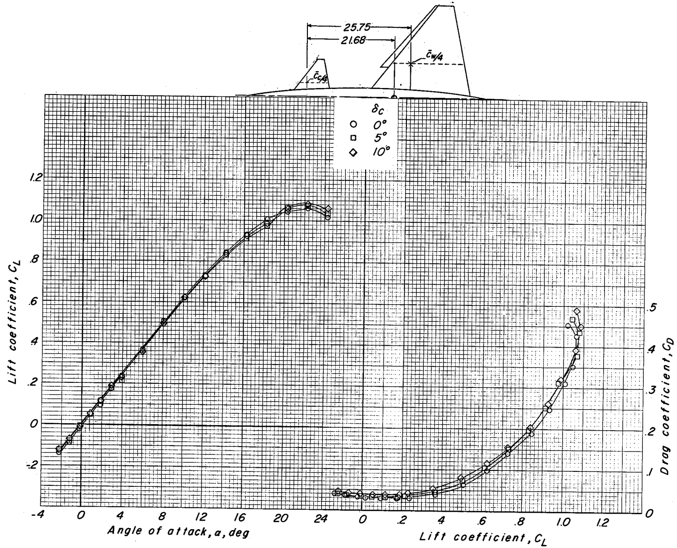
Figure 9.- Longitudinal aerodynamic characteristics of the configuration having a trapezoidal canard and the wing with partial-span leading-edge chord-extension, WBC_1 . \delta_{n,w} = -15^\circ .
