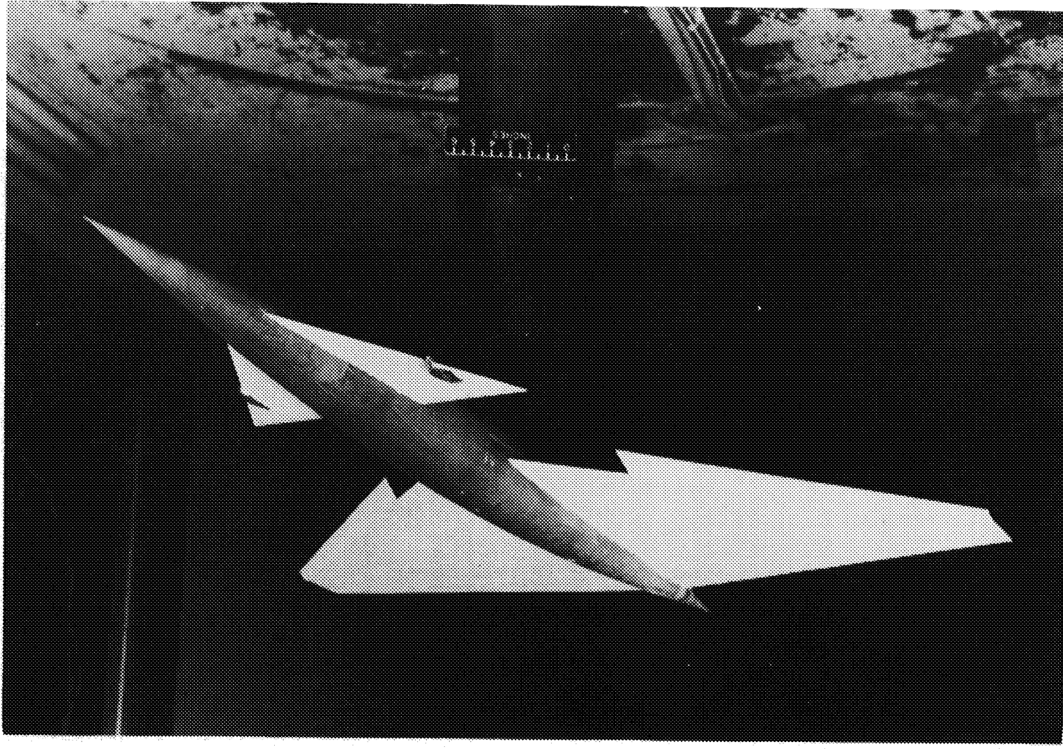
L-60-6524 Figure 3.- Configuration having a delta canard with fence and wing with partial-span chord-extension, mounted in the Langley 300-MPH 7- by 10-foot tunnel.
