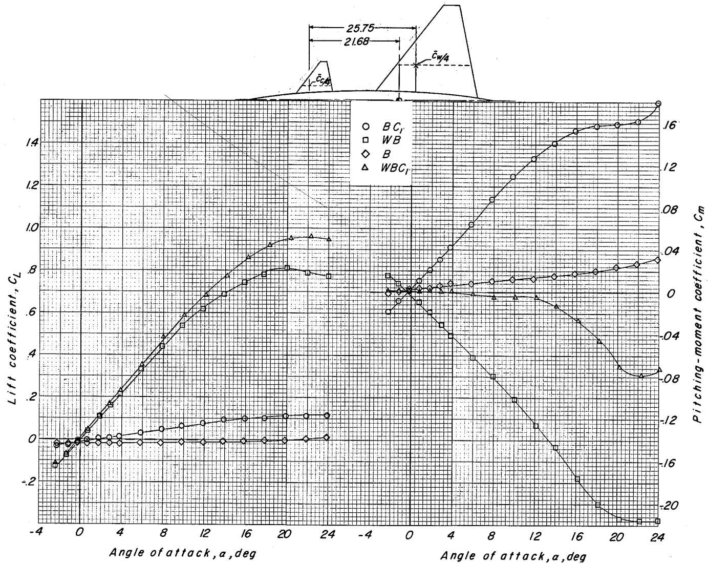
Figure 5.- Effect of various component parts on the longitudinal aerodynamic characteristics of the basic-wing—trapezoidal-canard configuration. All controls at zero deflection.
