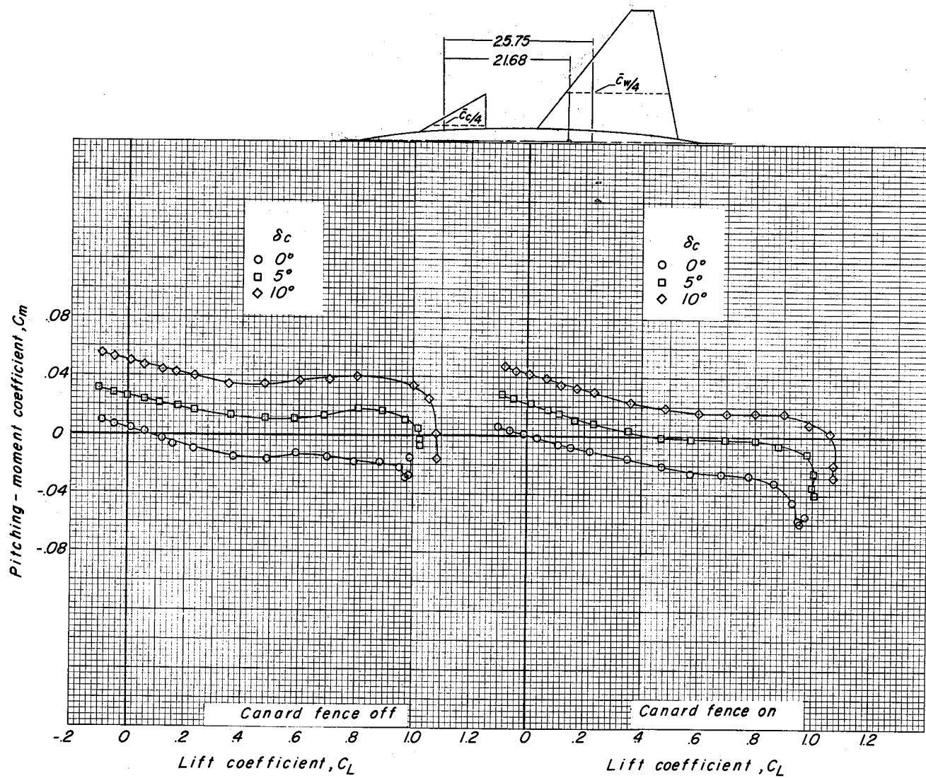
(b) Delta canard with and without fence.
