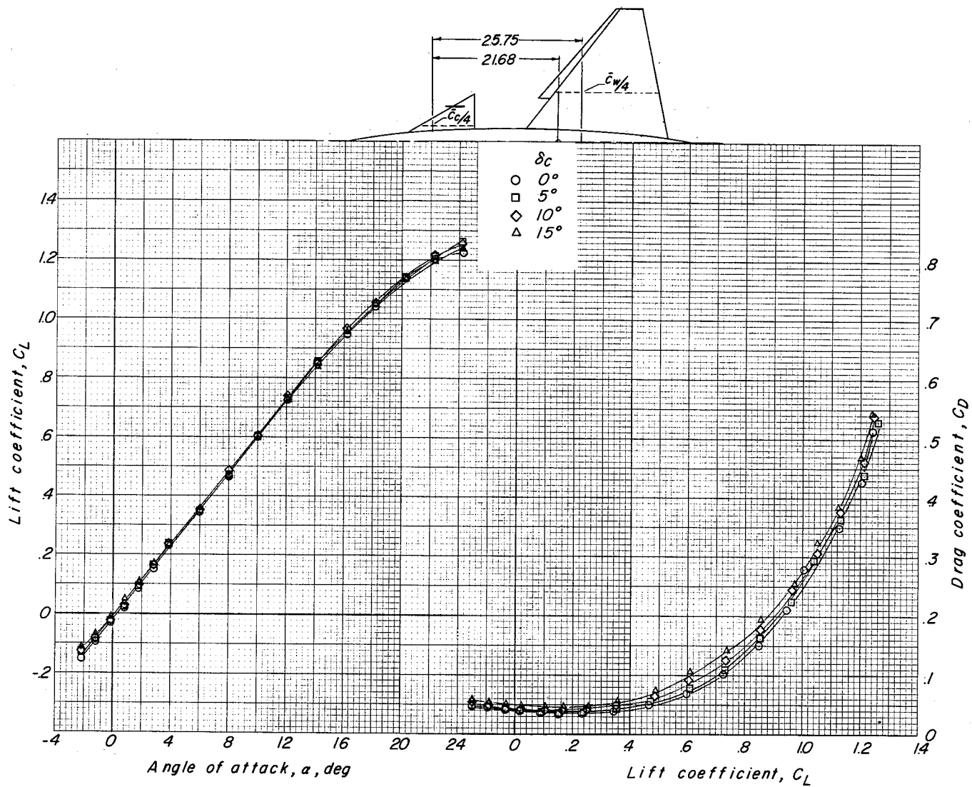
Figure 16.- Longitudinal control characteristics of the configuration having a delta canard with a fence and the wing having a partial-span chord-extension, WBC_{2,f} \cdot \delta_{n,w} = -30^\circ .
