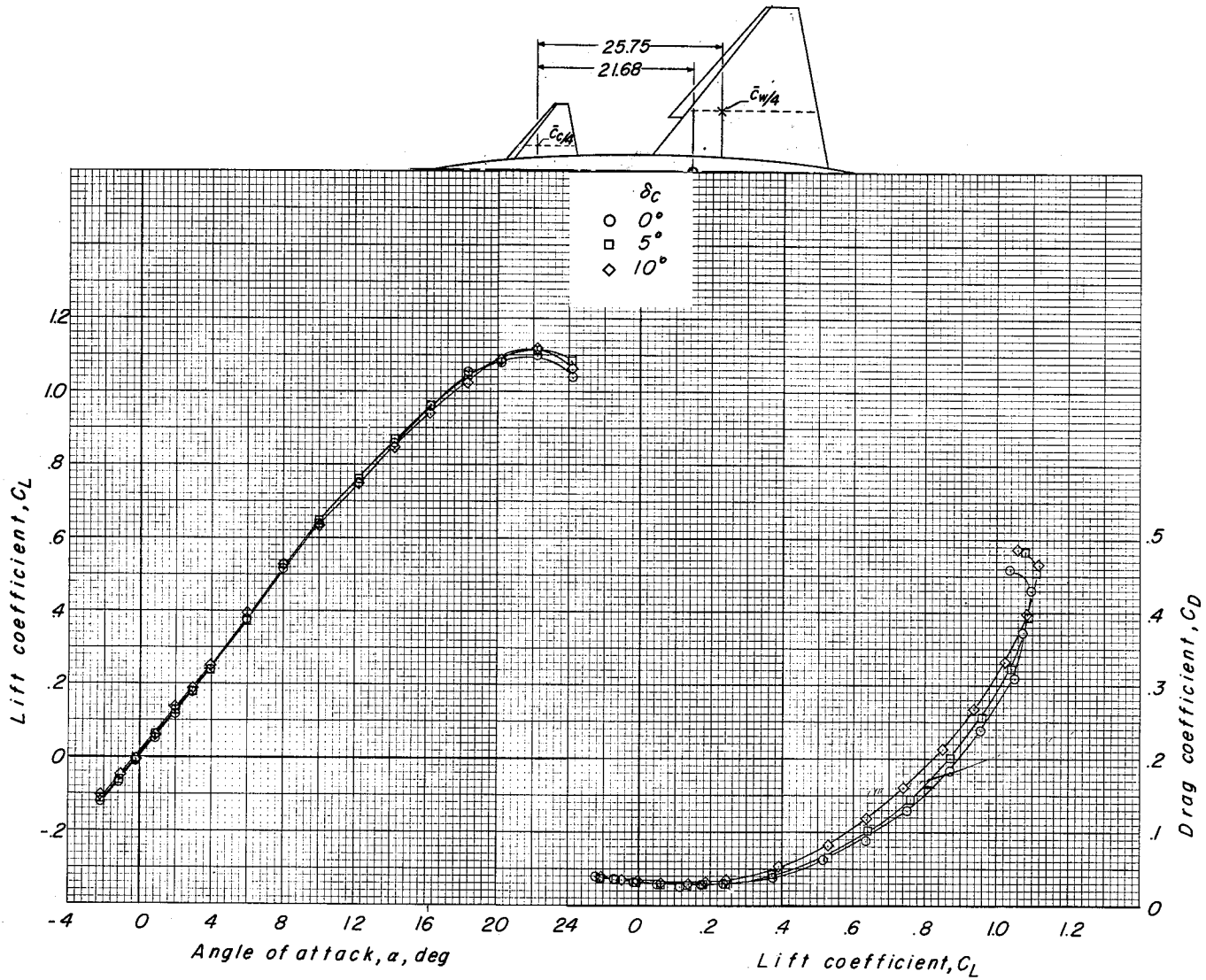
Figure 12.- Longitudinal aerodynamic characteristics of the configuration having a trapezoidal canard with full-span chord-extension and the wing having partial-span chord-extension. \delta_{n,cl} = -30^\circ ; \delta_{n,w} = -10^\circ .
