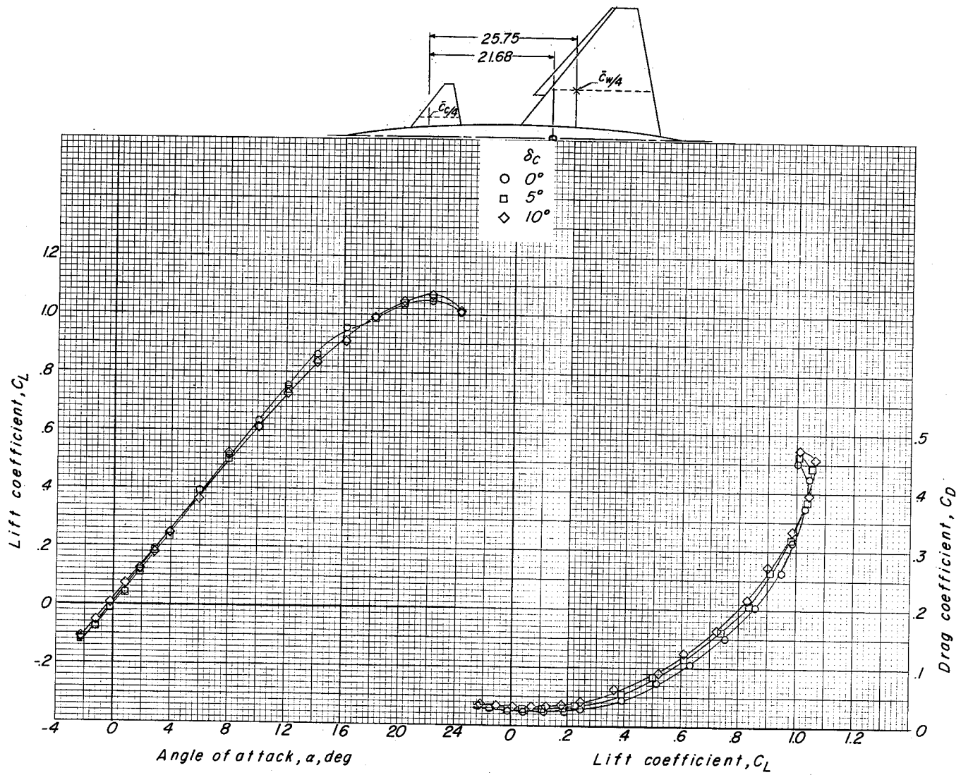
Figure 8.- Longitudinal aerodynamic characteristics of the configuration having a trapezoidal canard and the wing with partial-span leading-edge chord-extension, WBC_1 . \delta_{n,w} = 0^\circ .
