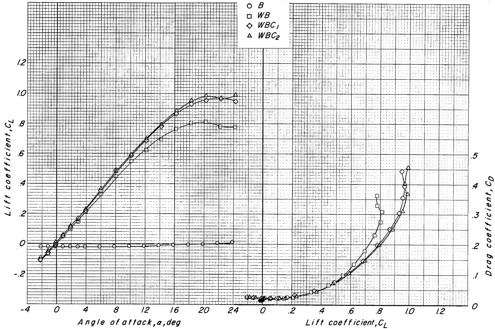
Figure 4.- Effect of the addition of delta and trapezoidal canard surfaces on the longitudinal aerodynamic characteristics of various configuration component parts. All control surfaces at zero deflection.
