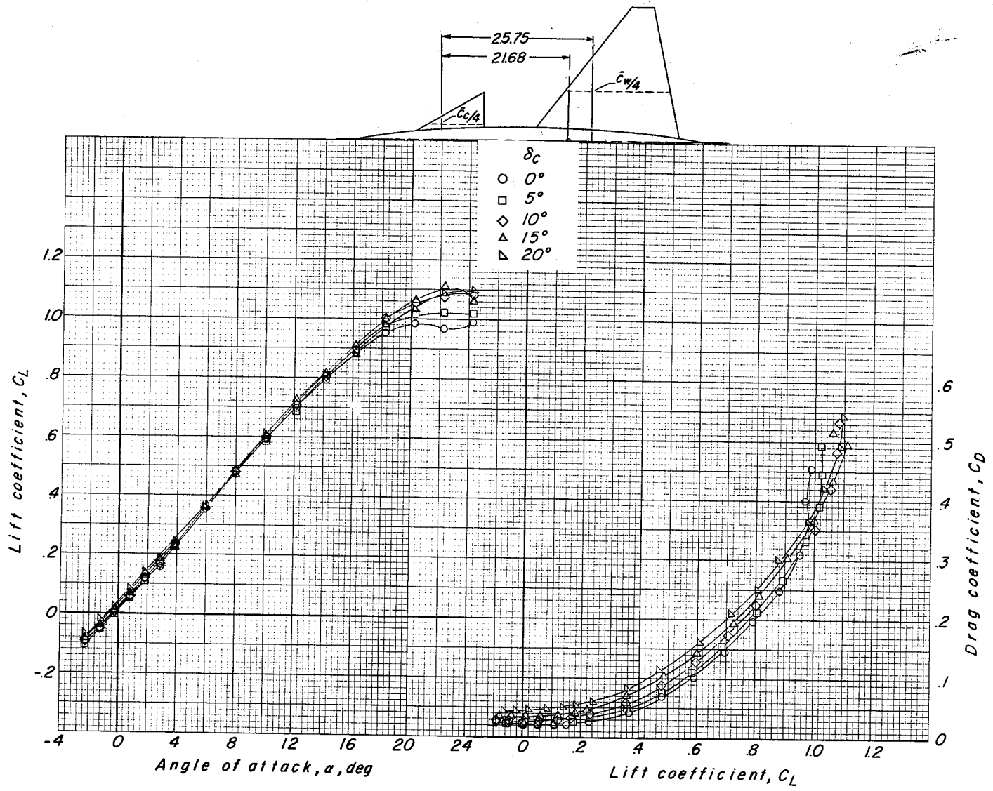
Figure 14.- Longitudinal control characteristics of the configuration having a delta canard and the basic wing, WBC 2 .
