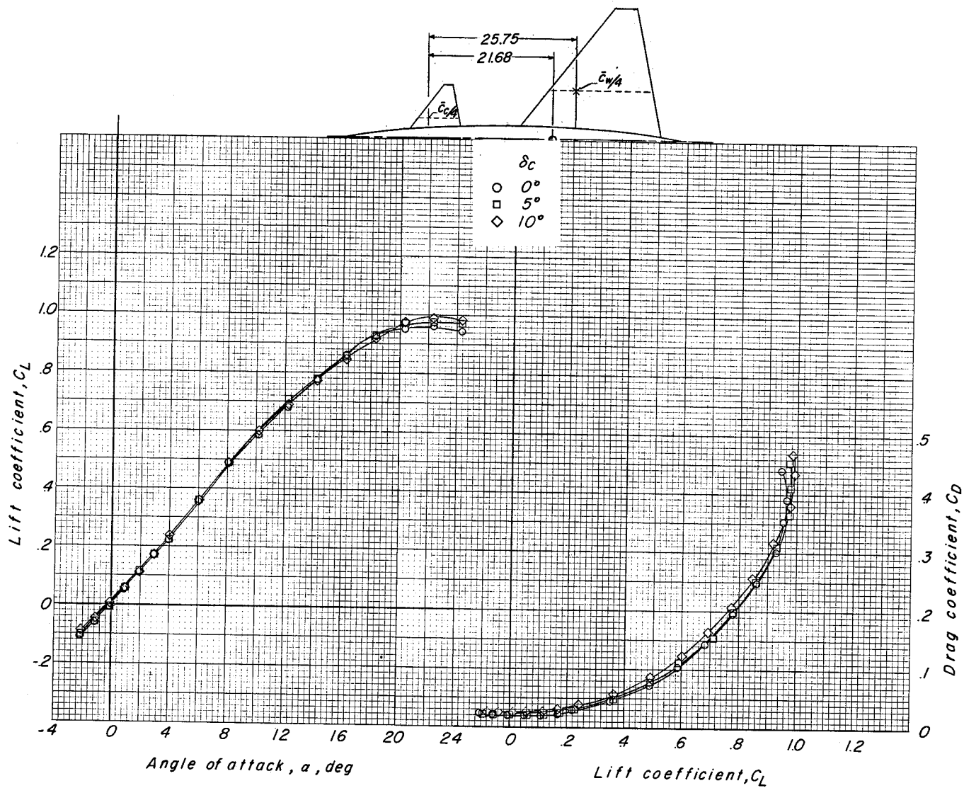
Figure 6.- Longitudinal control characteristics of the basic-wing--trapezoidal-canard configuration, WBC_1 .
