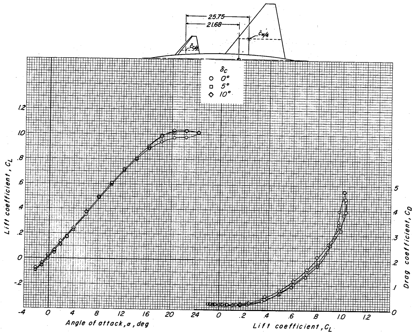
Figure 11.- Longitudinal aerodynamic characteristics of the configuration having the basic wing and a trapezoidal canard with full-span chord-extension, WBC_1 . \delta_{n,c1} = -30^\circ .
