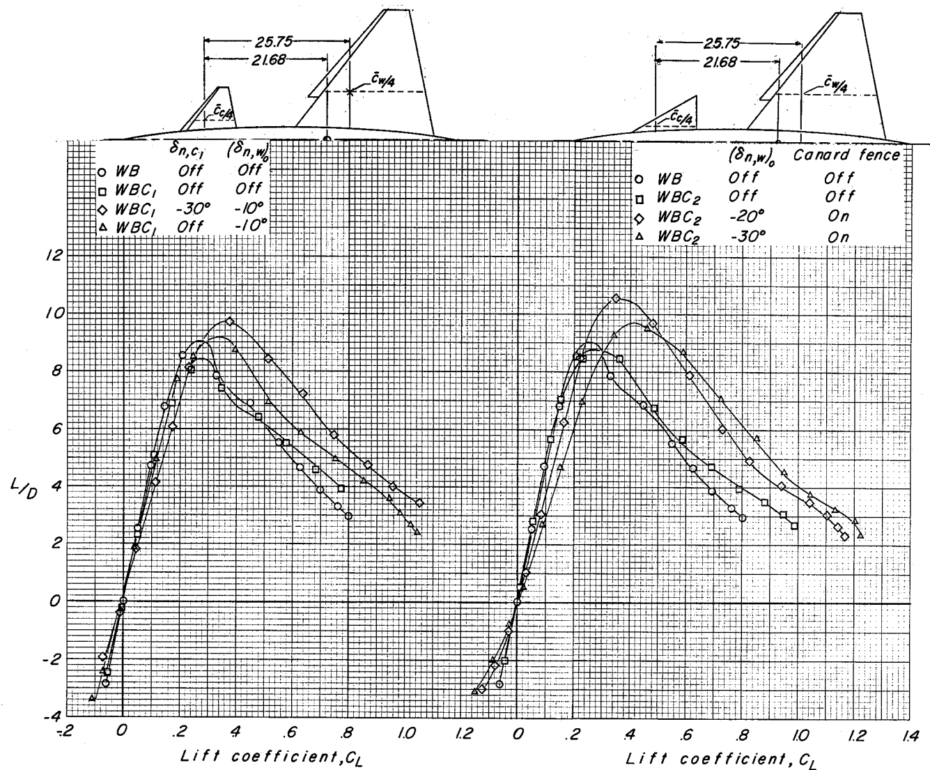
Figure 21.- Comparison of the trends in L/D for various configurations with the trapezoidal canard and delta canard. \delta_c = 0^\circ .
