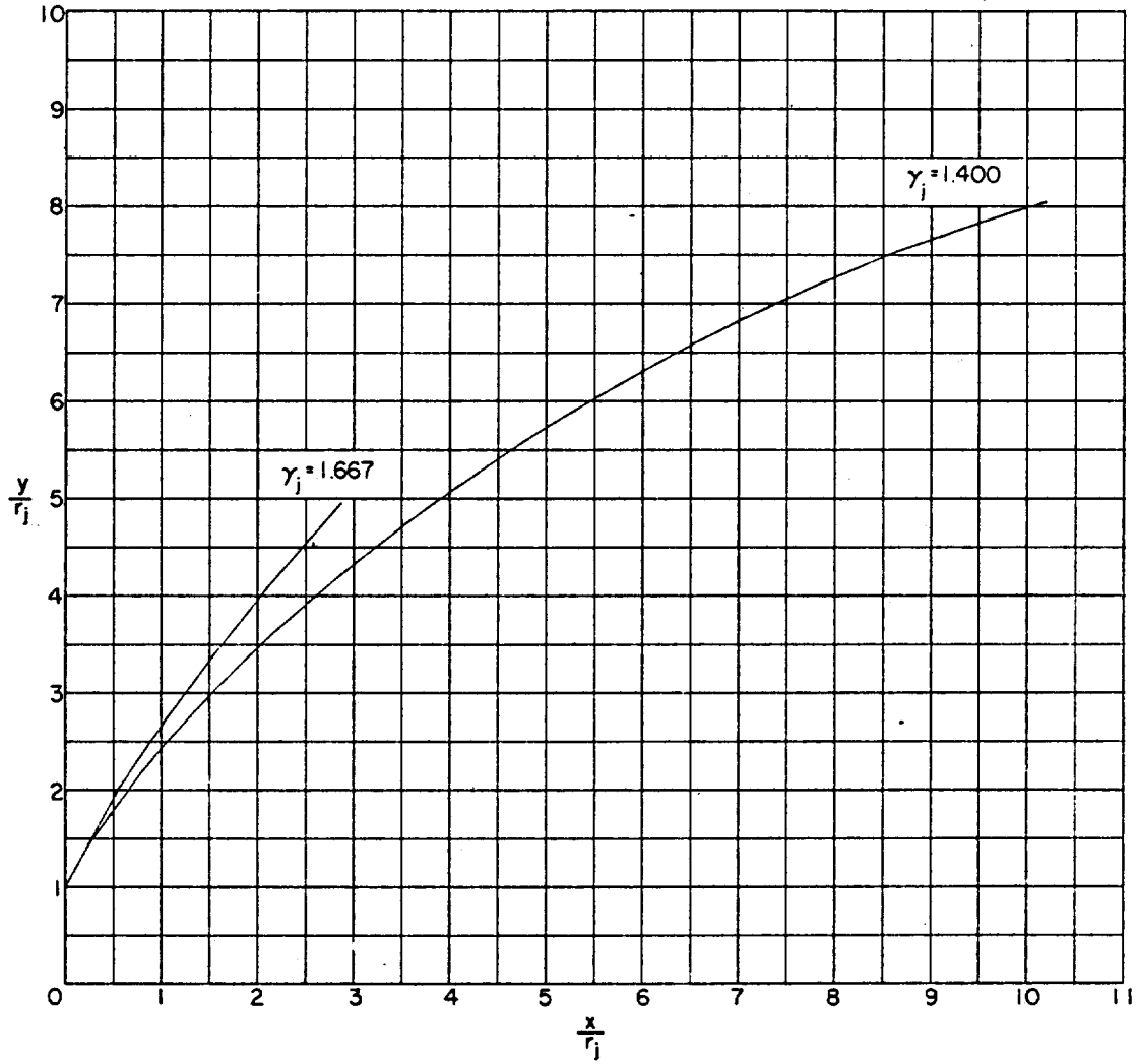
FIGURE 41.—Example of effect of \gamma_j at large pressure ratios upon shape of boundary for similar initial inclinations of boundary. Jet exhausting into still air; M_j=2.5 ; \theta_N=15^\circ ; \delta_j \approx 60^\circ .
