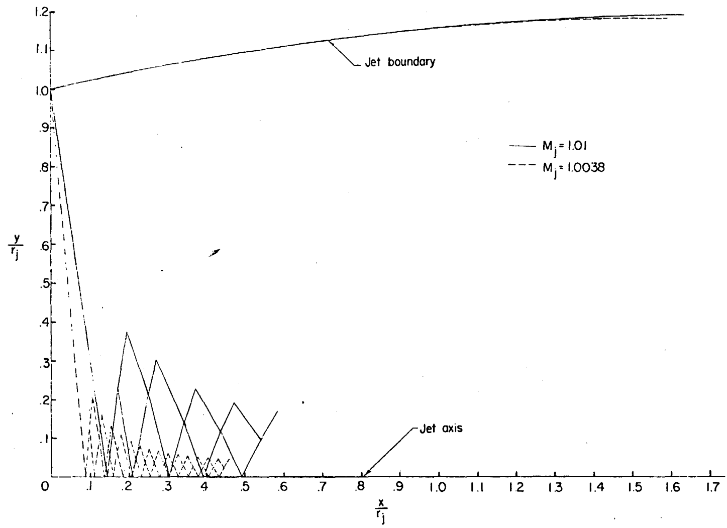
Figure 73.—Comparison of characteristic calculations for near-sonic exit to show effect of errors in flow field near jet axis upon jet boundary \gamma_i=1.400 ; \rho_j/p_\infty=2 .
