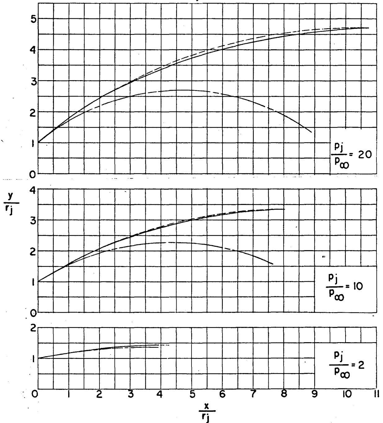
FIGURE 23.—Comparison of jet boundary given by characteristic calculations, circular-arc boundary passing through (\frac{y}{r_j})_{\max} , and the circular-arc defined by initial radius of curvature. M_j = 2.00 .
