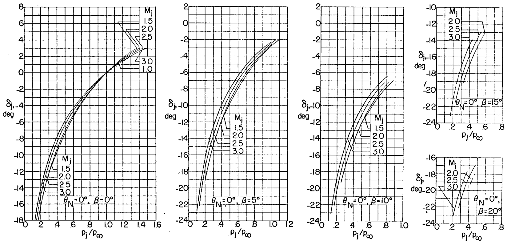
FIGURE 57.—The effects of jet pressure ratio upon the initial inclination of the mixing boundary at M_\infty = 1.2, \gamma_\infty = 1.400, \gamma_j = 1.286 .
