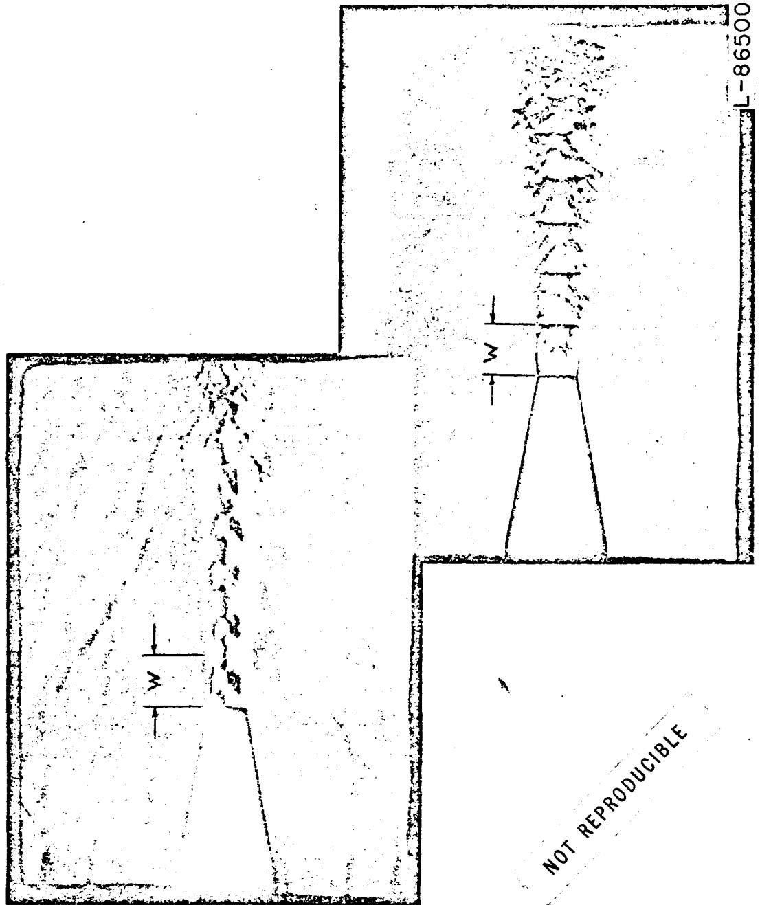
FIGURE 6.—Example of primary wavelength. M_1 = 1.00 ; \theta_N = 0^\circ ; p_1/p_\infty = 1.76 .
