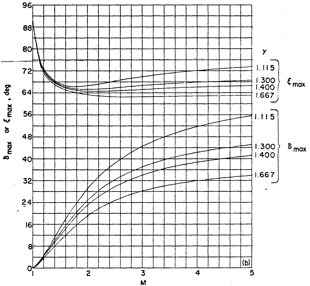
FIGURE 15.—Effect of the ratio of specific heats upon the maximum turning angle of two-dimensional flow through an attached shock and upon the inclination of the shock.
