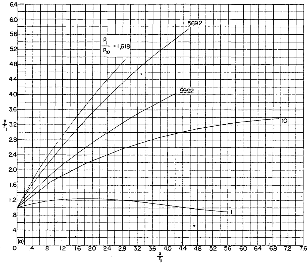
FIGURE 39.—Composite presentation of calculated boundaries for jet exhausting into still air with M_j = 2.5 and \theta_N = 15^\circ .
