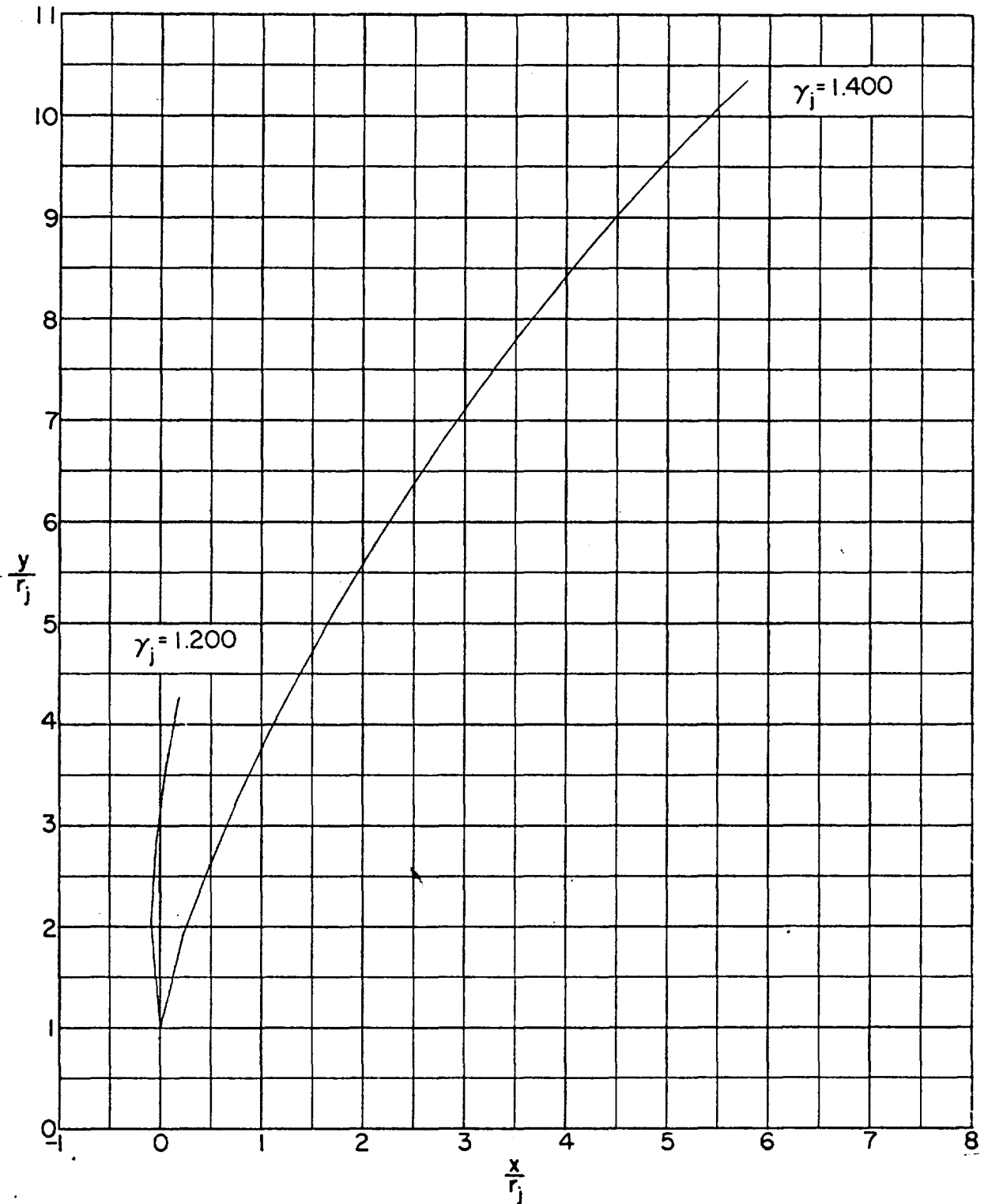
FIGURE 40.—Example of the effect of \gamma_j at large pressure ratios upon shape of boundary for similar pressure ratios. Jet exhausting into still air; M_j = 2.5 ; \theta_N = 15^\circ ; p_i/p_\infty \approx 1,300 .
