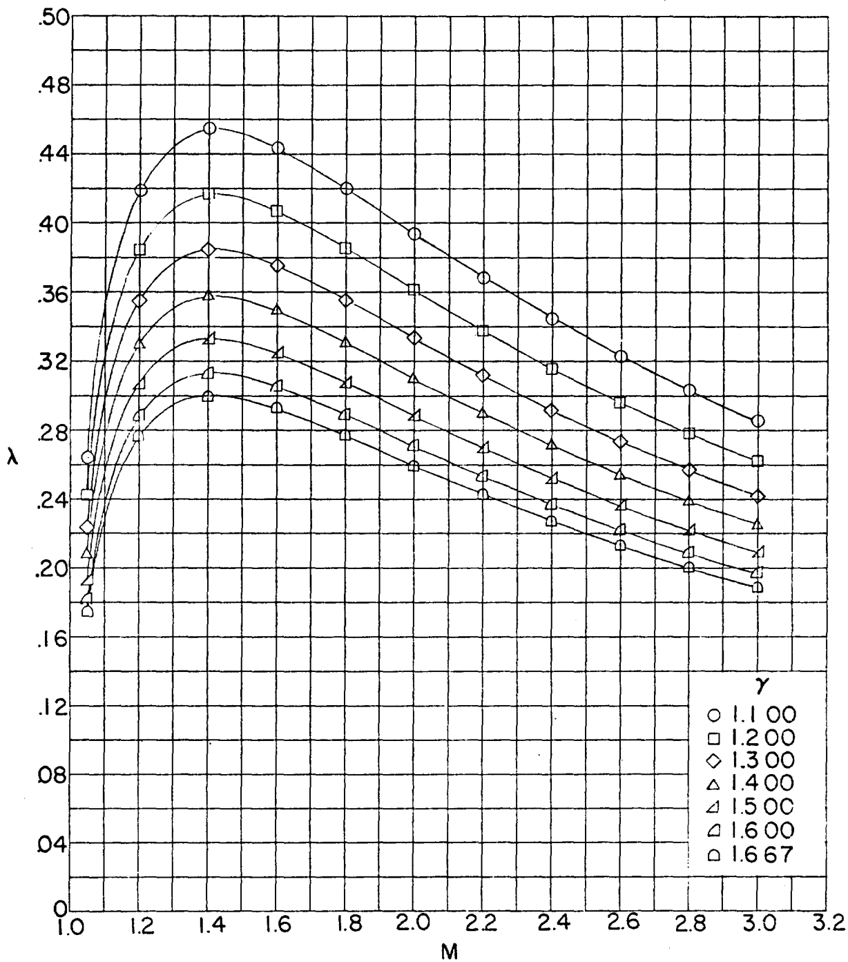
FIGURE 62.—Variation of basic Kawamura parameter with Mach number for several ratios of specific heats.
