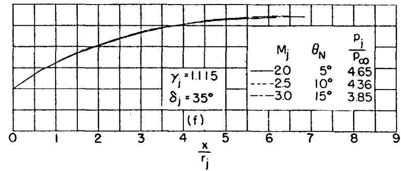
FIGURE 33.—Examples of jet boundary simulation.
