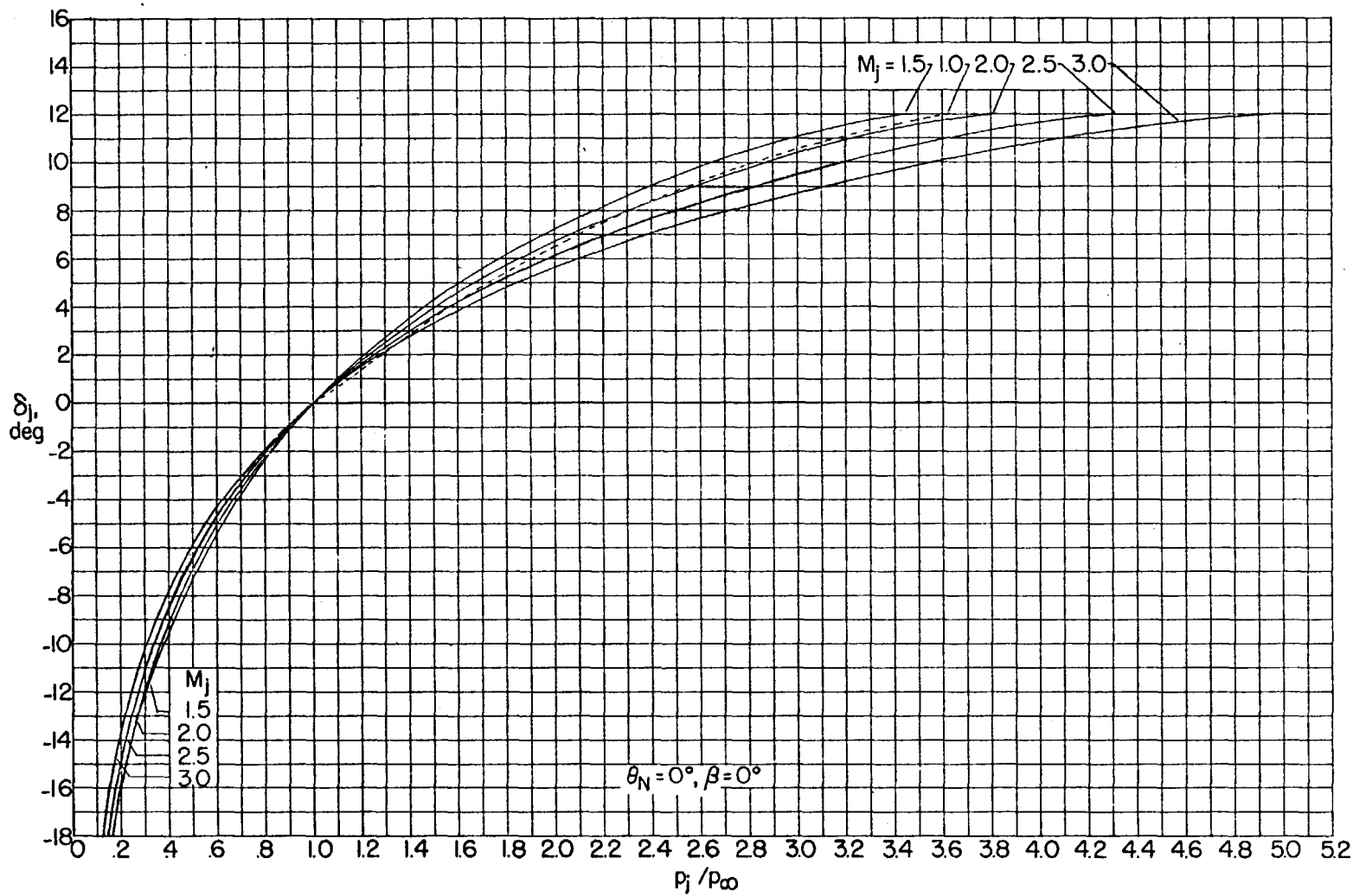
FIGURE 58.—The effects of jet pressure ratio upon the initial inclination of the mixing boundary at M_\infty = 1.5 , \gamma_\infty = 1.400 , \gamma_j = 1.286 .
