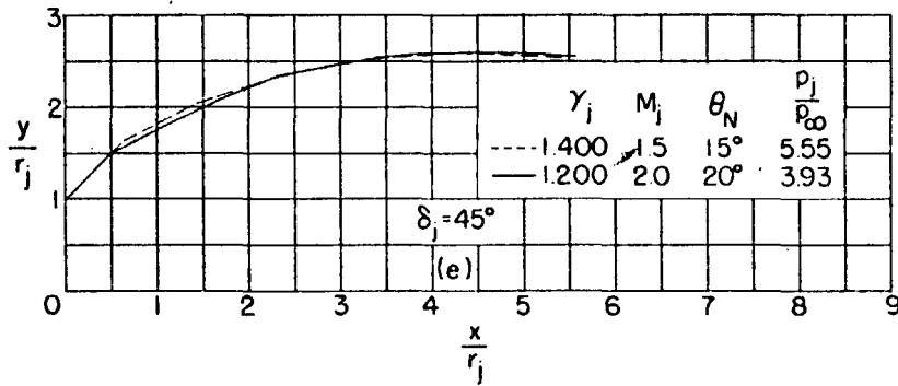
FIGURE 33.—Examples of jet boundary simulation.
