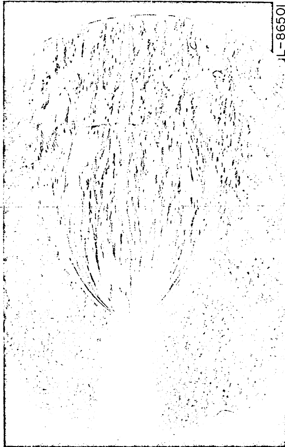
FIGURE 12.—Example of large initial inclination of jet boundary. M_j = 1.00 ; \theta_N = 0^\circ ; p_i/p_\infty = 105 .
