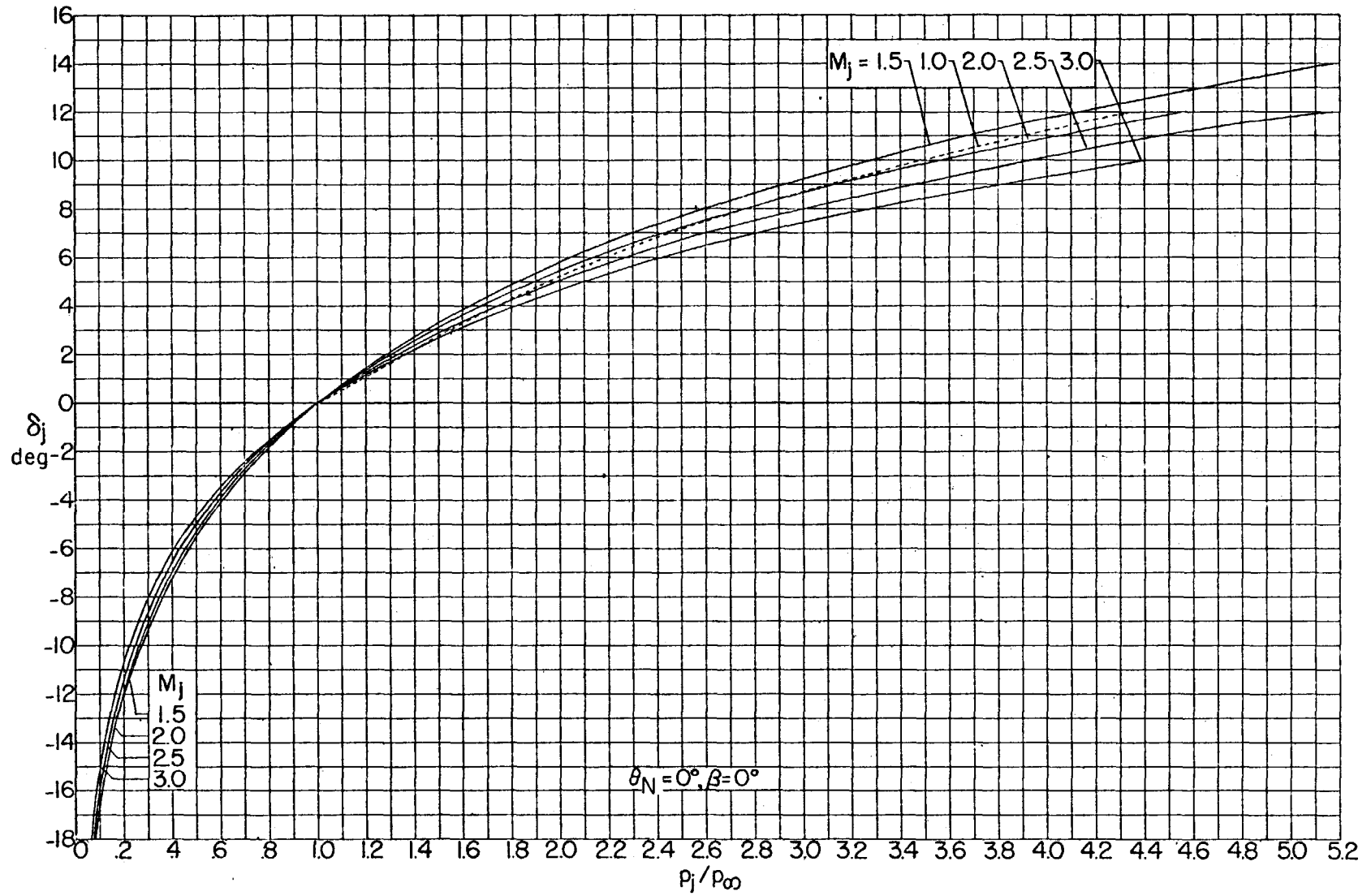
FIGURE 61.—The effects of jet pressure ratio upon the initial inclination of the mixing boundary at M_\infty = 3.0, \gamma_\infty = 1.400, \gamma_i = 1.286 .
