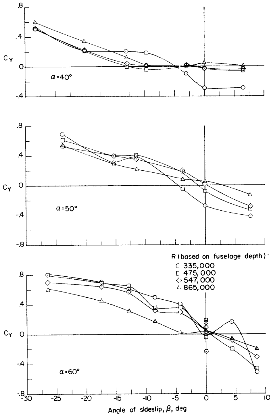
Figure 12.- Variation of side-force coefficient with sideslip for various Reynolds numbers and angles of attack. (Complete model.)
