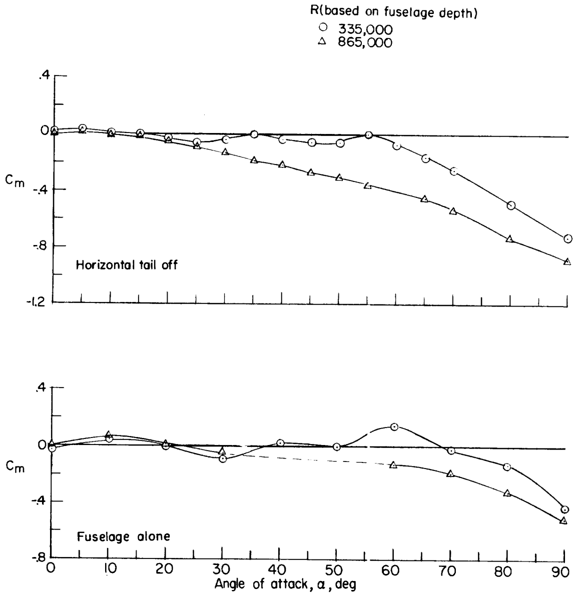
(b) Horizontal tail off and fuselage alone.
