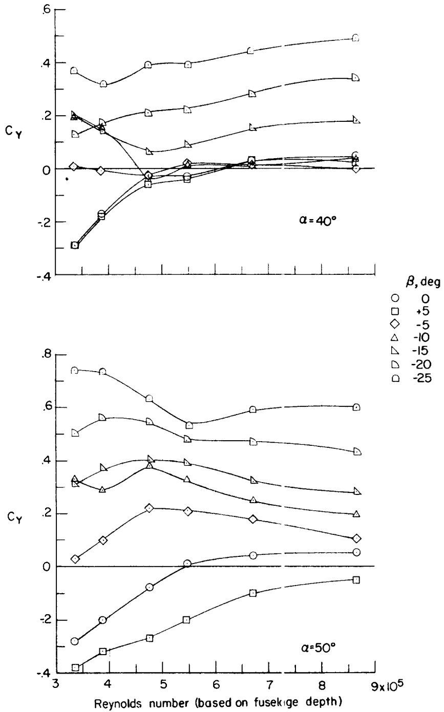
Figure 14.- Variation of side-force coefficient with Reynolds number for various sideslip angles and angles of attack. (Complete model.)
