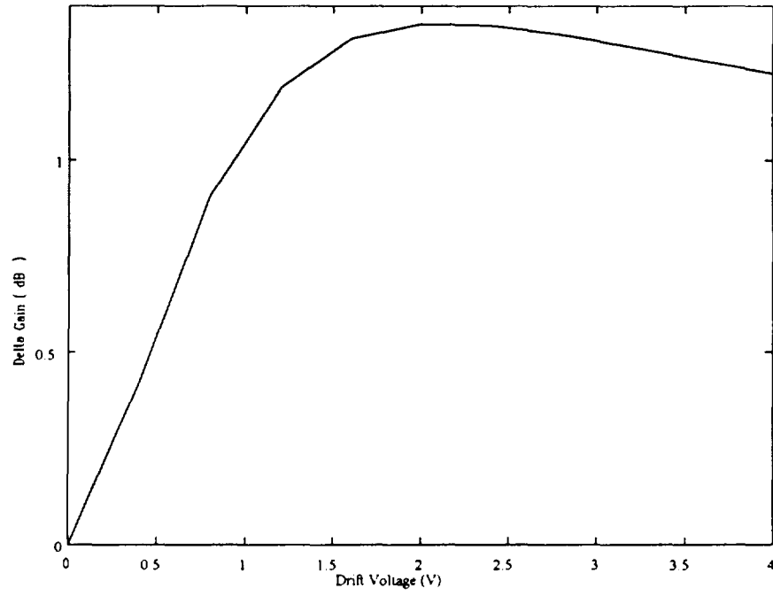
Figure 4.23: Predicted gain curve for the device of Figure 4.16 with a 1 \mu\text{m} ZnO overlay
