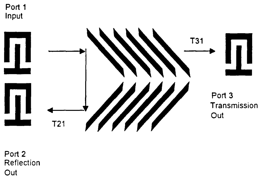
Figure 5.3: Reflection test structure.
