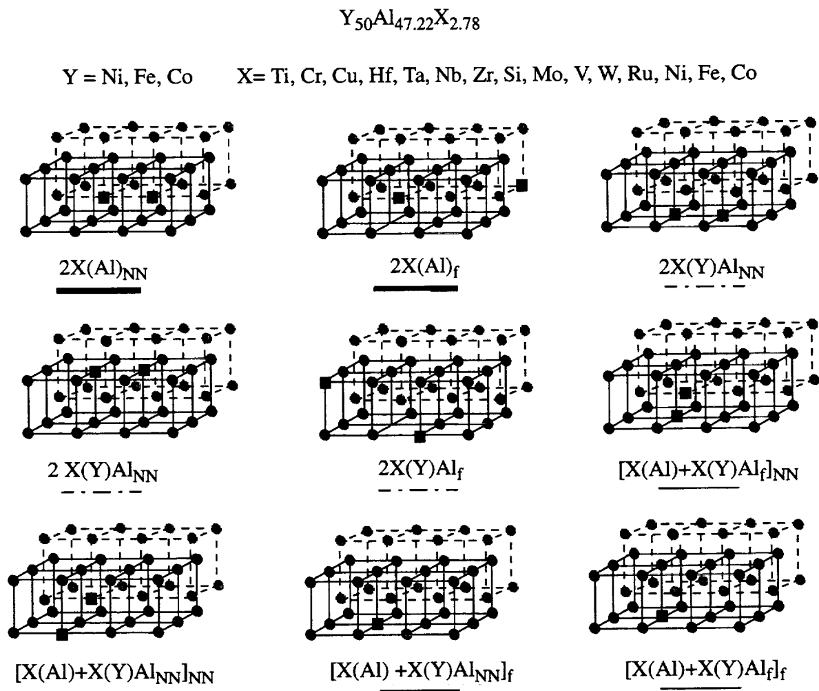
Figure 3: Configurations for two atoms in a 72-atom cell. A section of the cell containing the defect is shown. Y atoms (Ni, Fe, Co in NiAl, FeAl and CoAl, respectively) are indicated with solid black disks, Al atoms with grey disks and the additive X with a solid square.
