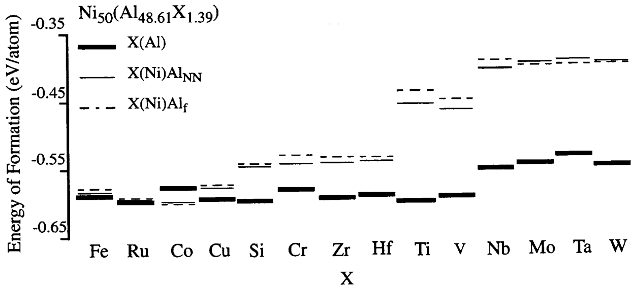
Figure 2: Energy spectrum for alloying additions to \text{Ni}_{50}(\text{Al},\text{X})_{50} . The thick solid line corresponds to X(Al) defects (see Fig. 1.a), whereas thin solid lines and dashed lines correspond to X(Ni)Al defects as shown in Figs. 1.b and 1.c, respectively.
