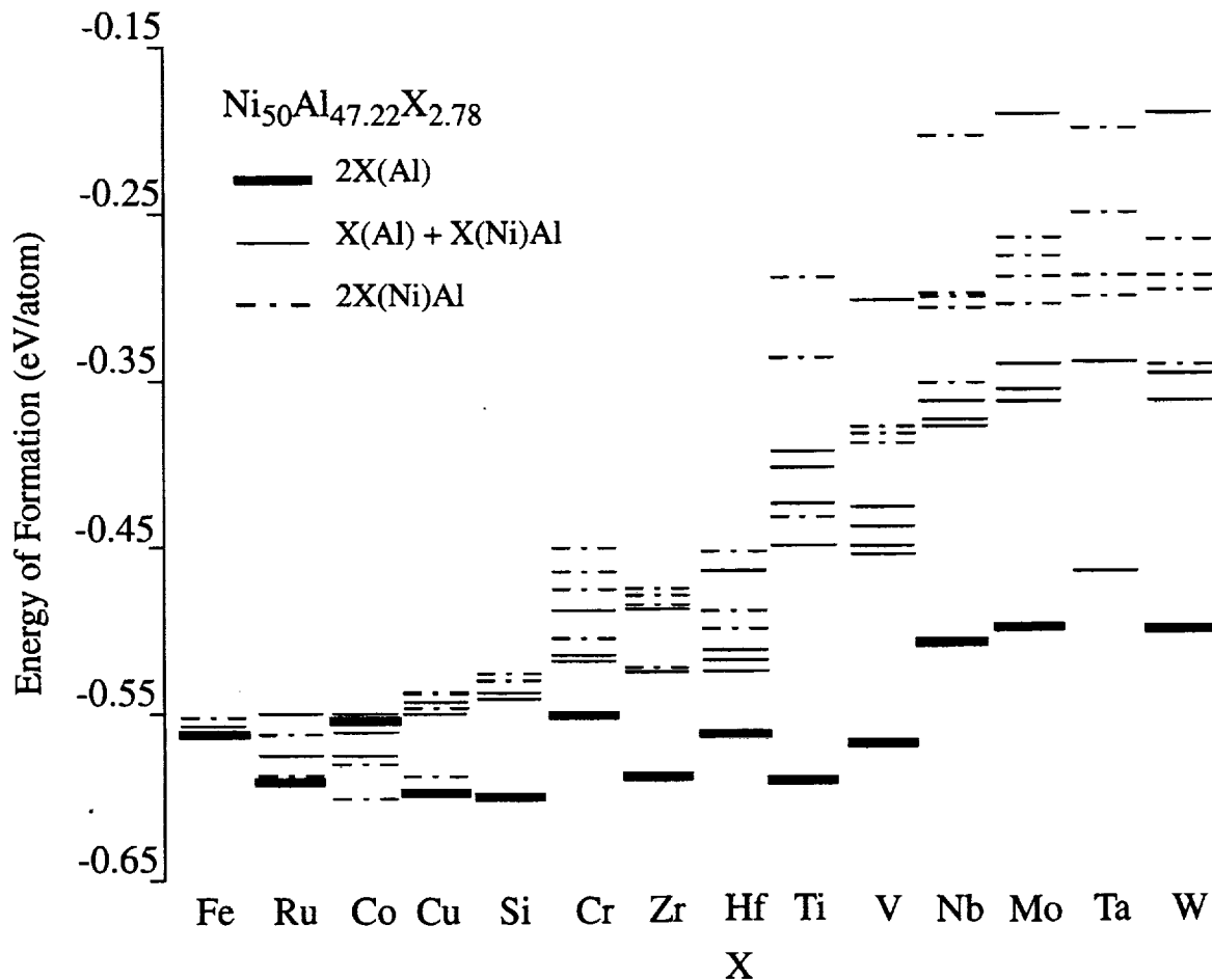
Figure 4: Energy spectrum of the configurations shown in Fig. 3. For each element, the different energy states are grouped depending on the type of defect: two X atoms in Al sites (solid thick line), one X atom in an Al site and one in a Ni site (thin solid line) and both X atoms in Ni sites (dashed lines). In those cases where the X atom occupies a Ni site, an antistructure defect is also created. The different levels for the same type of defect correspond to the differences due to the relative location of the defects with respect to each other.
