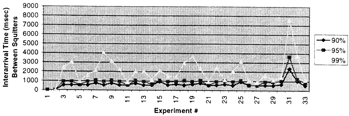
Figure R7 : Confidence Levels for Interarrival Times of Long Squitters (NASA Vehicles)
