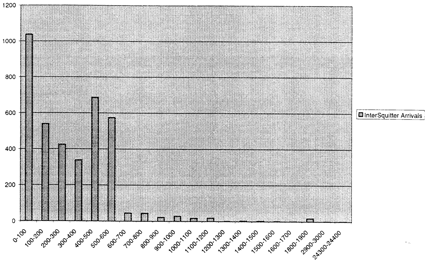
Figure 14-1: Histogram of InterSquitters (NASA) Low Traffic (55)
