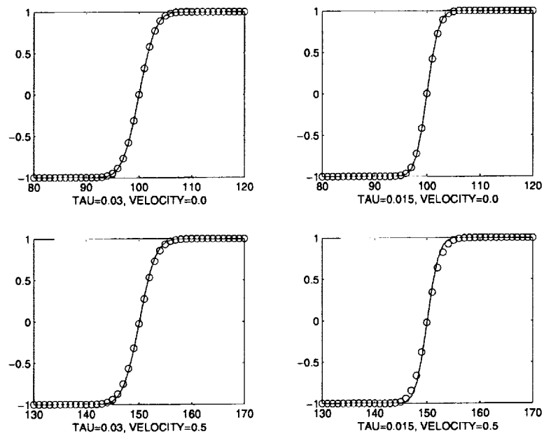
FIG. 5.1. Propagation of function Z with velocity U = 0 (top) and U = 0.5 (bottom). The collision times used are \tau = 0.03 (left) and \tau = 0.015 (right) respectively. The solid lines are exact solutions and the circles are numerical solutions.
