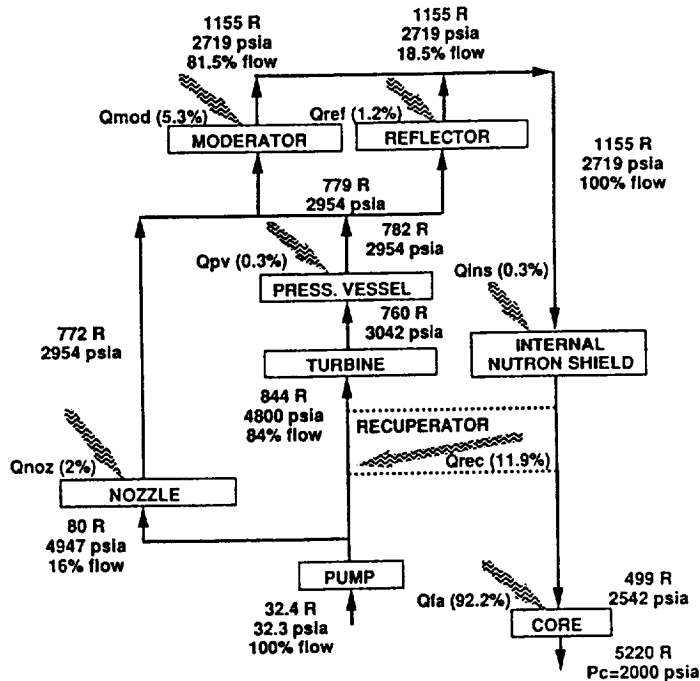
Fig. 5 Flow Schematic of Recuperated Topping Cycle for the CIS Engine
