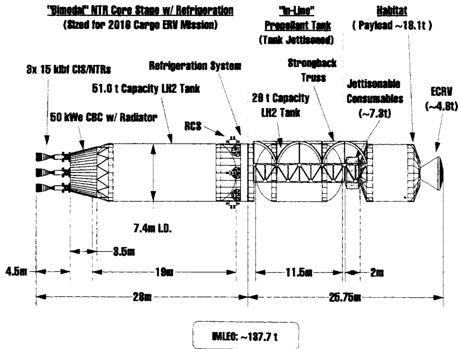
Fig. 16 Size, Mass and Key Features of BNTR-Powered ERV with Crew Habitat and Spare ECRV
