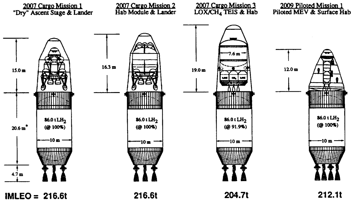
Fig. 1 Reference Mars Cargo and Piloted Vehicles Using Common “NTR-Powered” TMI Stage
