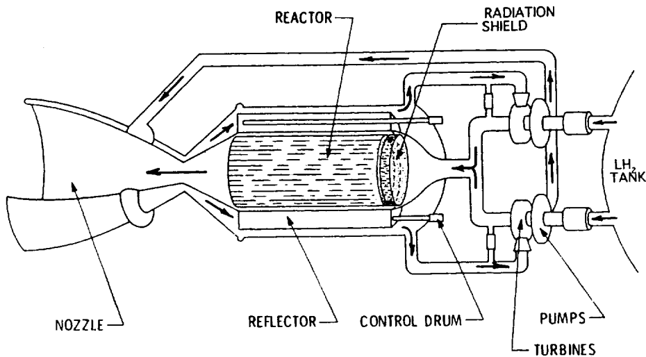
Fig. 3 Schematic of "Solid Core" NTR Using Dual Turbopump Expander Cycle
