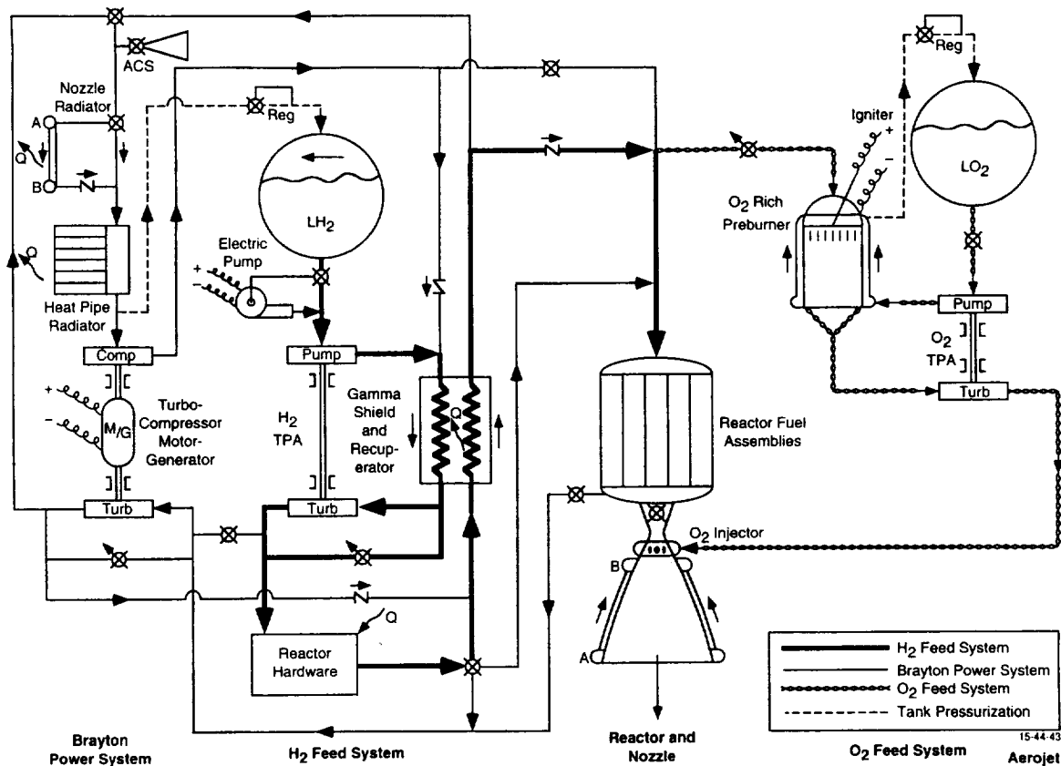
Fig. 9 Flow Schematic of "bimodal" LANTR Engine
