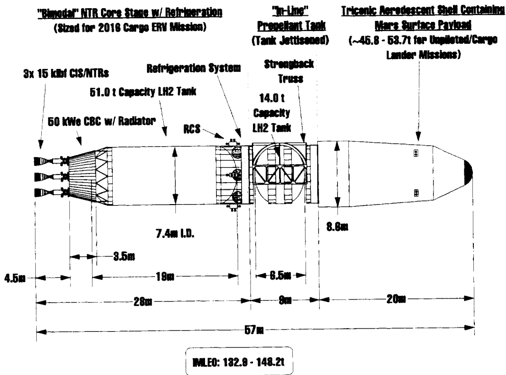
Fig. 31 Size, Mass and Key Features of BNTR Vehicles for Cargo and "Unpiloted" Hab Lander Missions
