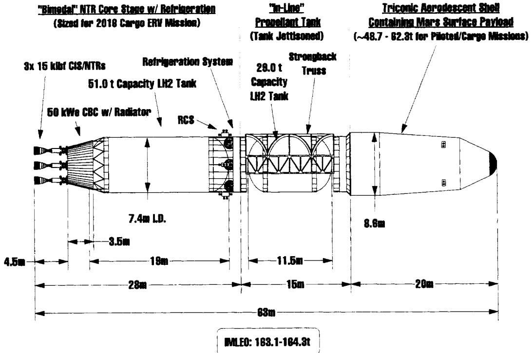
Fig. 22 Characteristics of "All BNTR" Transfer Vehicles for Piloted and Cargo Lander Missions
