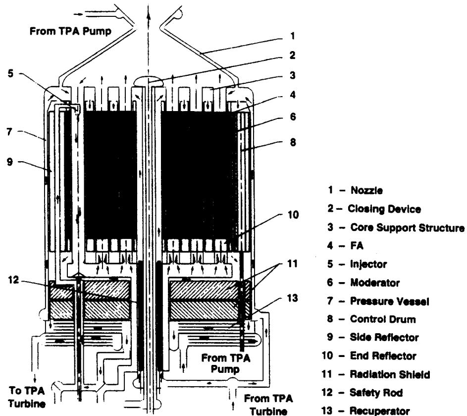
Fig. 4 Component Layout / Flow Schematic of CIS Engine
