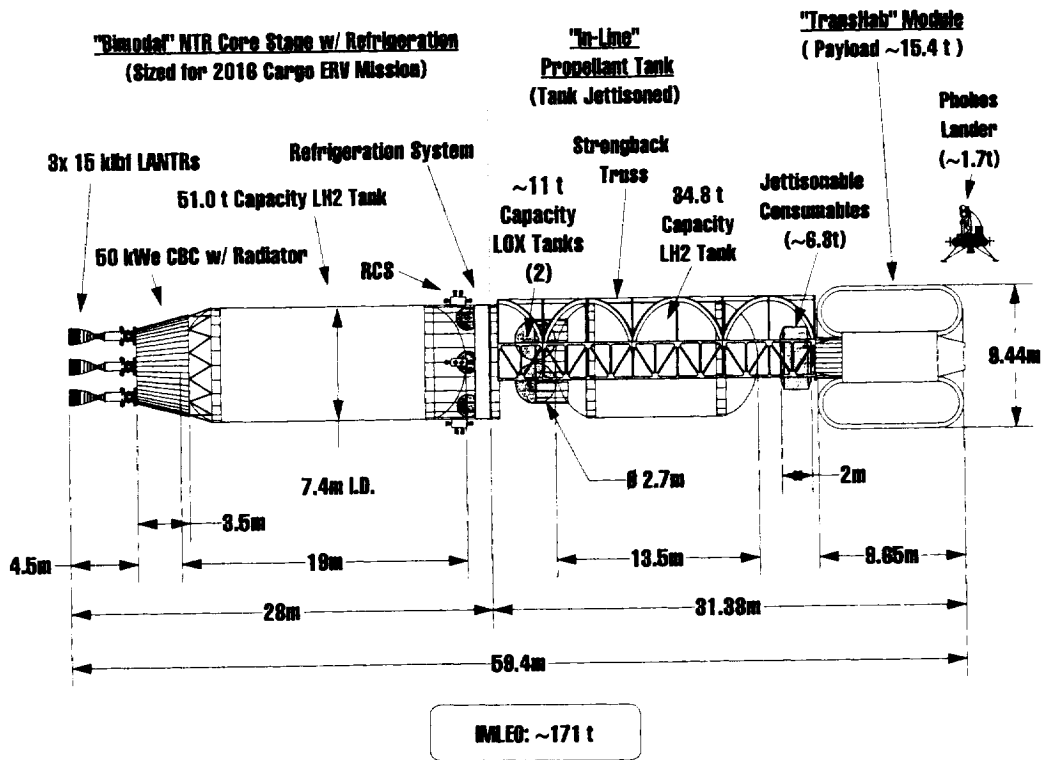
Fig. 28 Size, Mass and Key Features of "Stretch" LANTR / ERV for Phobos Lander Option
