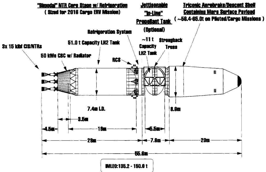
Fig. 20 Size, Mass and Key Features of BNTR Transfer Stage for Cargo and Piloted Lander Missions
