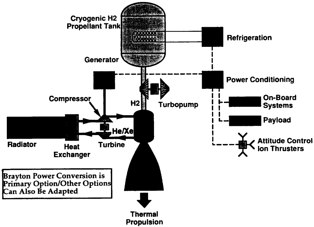
Fig. 6 Key Components of "Bimodal" NTR Stage -- "A Fully Integrated System"
