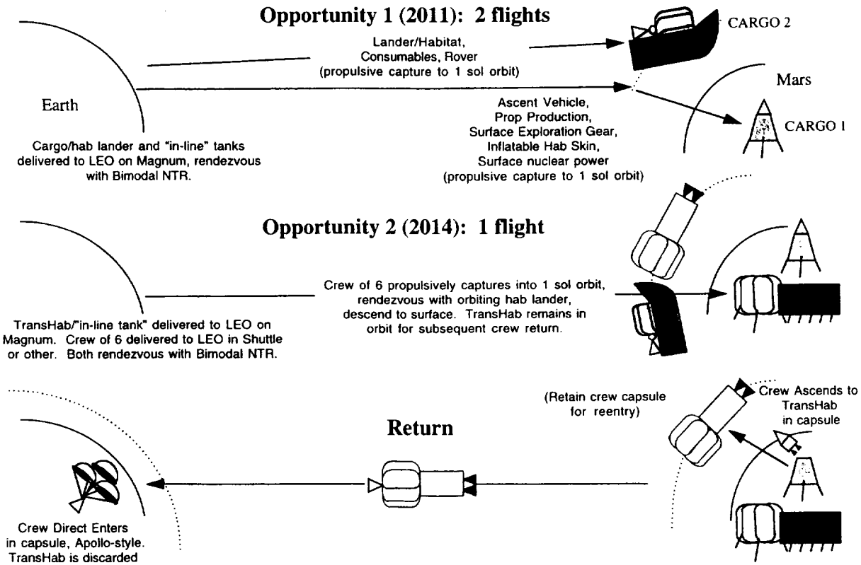
Fig. 29 "Alternative Mission Profile": Round Trip Piloted Transfer Vehicle Using BNTR and TransHab
