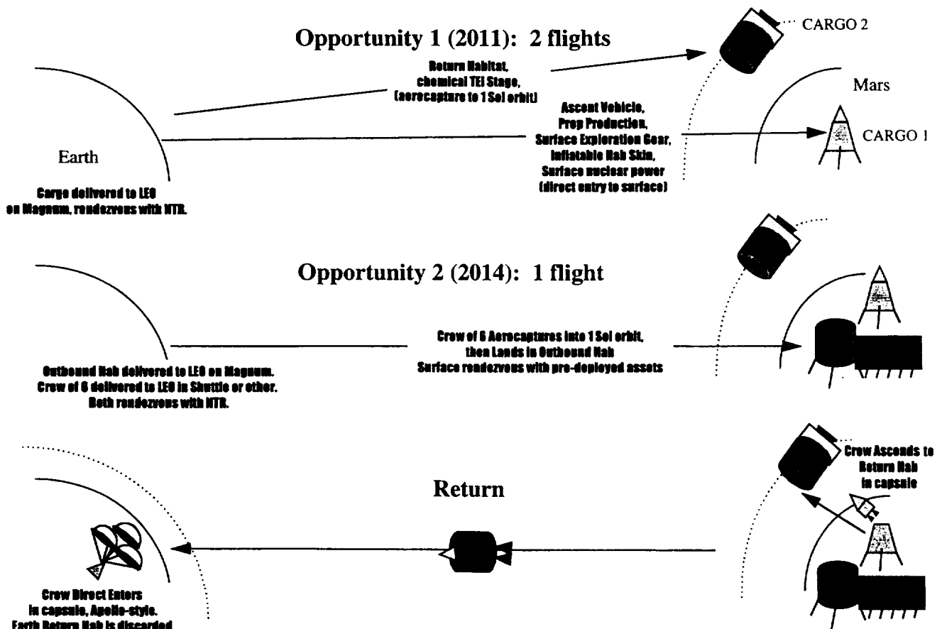
Fig. 10 Candidate Mission Profile for Mars Design Reference Mission
