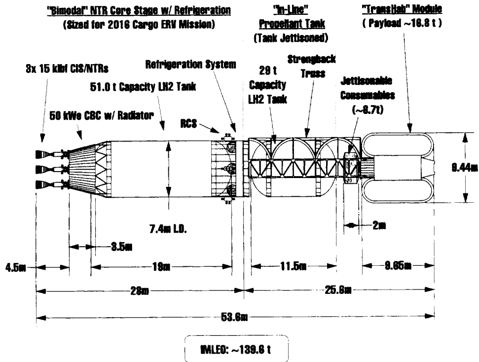
Fig. 30 Size, Mass and Key Features of Round Trip Piloted Transfer Vehicle
