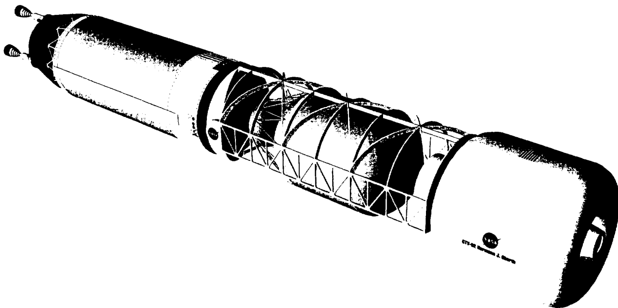
Fig. 27 3-D Image of Bimodal LANTR Transfer Vehicle for Mars / Phobos Mission Option
