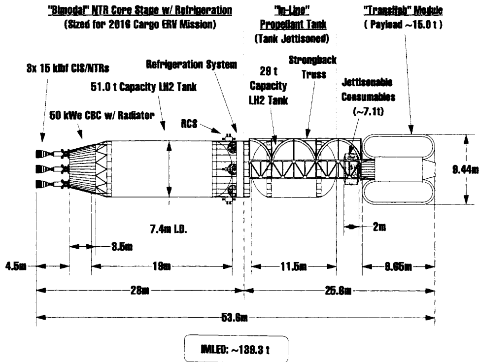
Fig. 24 Size, Mass and Key Features of Reusable Bimodal ERV Using TransHab
