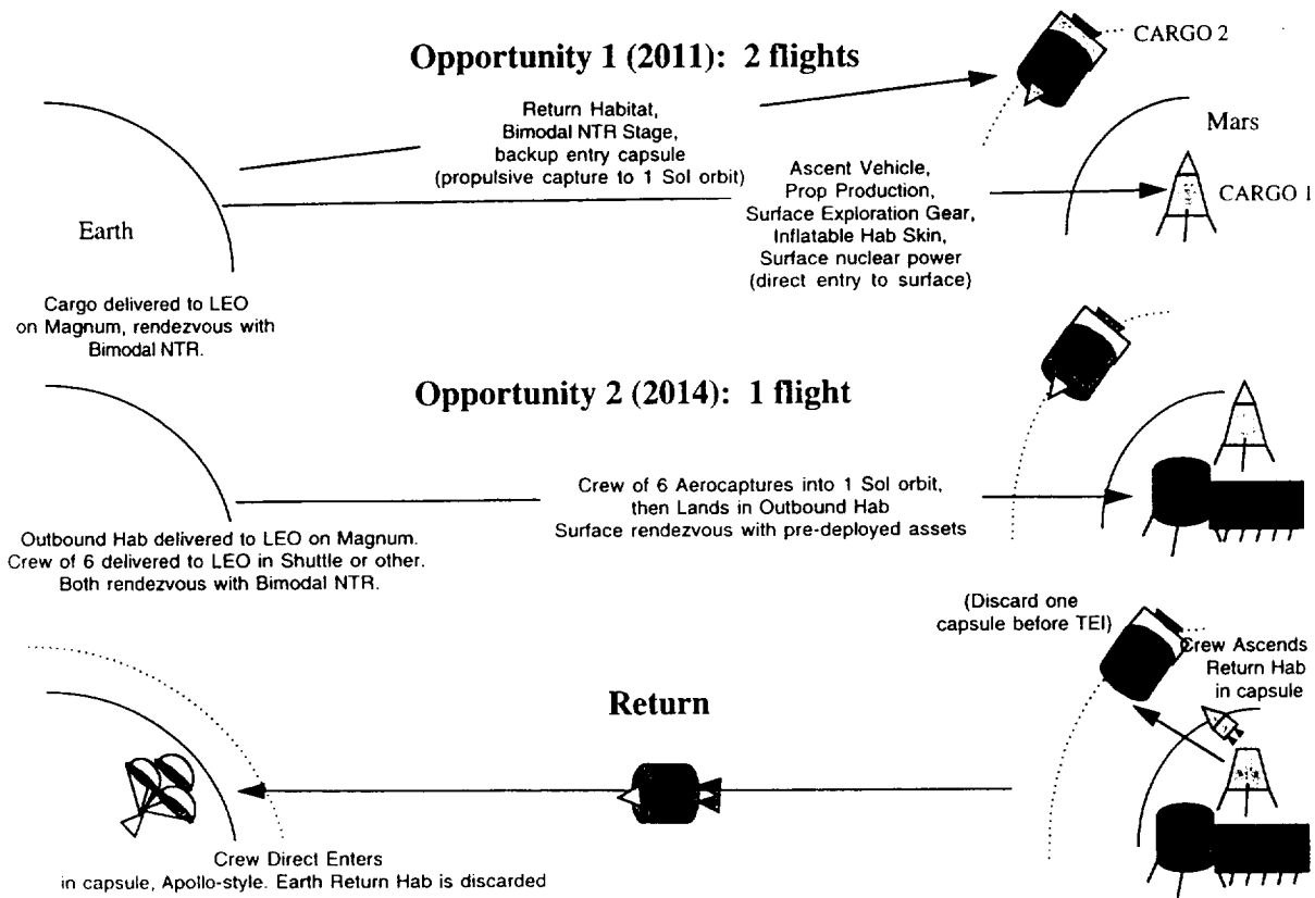
Fig. 15 "Modified" Mars Mission Profile Using Bimodal NTR Vehicle Concept
