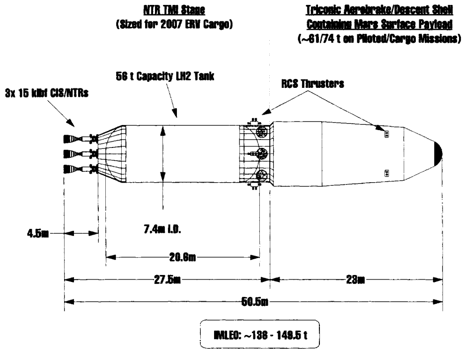
Fig. 11 Size, Mass and Key Features of "Common" TMI Stage and Aerobraked Payloads
