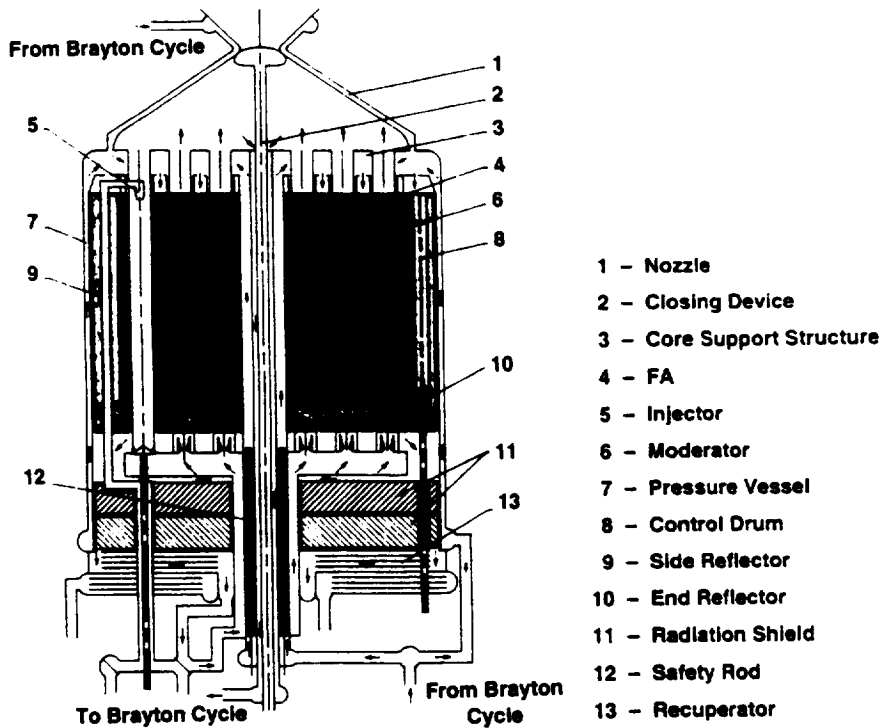
Fig. 7 Design Features of "Bimodal" CIS Engine Concept
