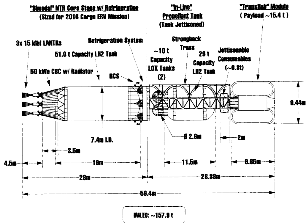
Fig. 26 Size, Mass and Key Features of Bimodal LANTR Transfer Vehicle for Mars / Phobos Mission Option
