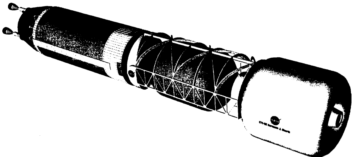
Fig. 25 3-D Image of Reusable Bimodal ERV with Inflatable TransHab Crew Module
