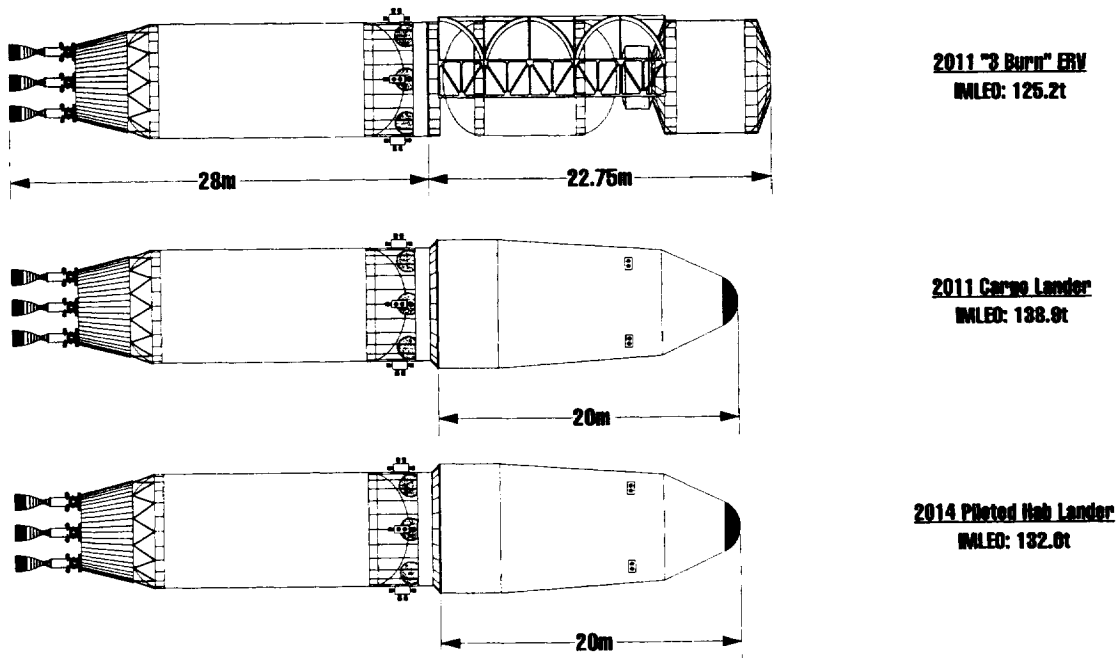
Fig. 21 BNTR Transfer Vehicles Used in Comparison with the DRM
