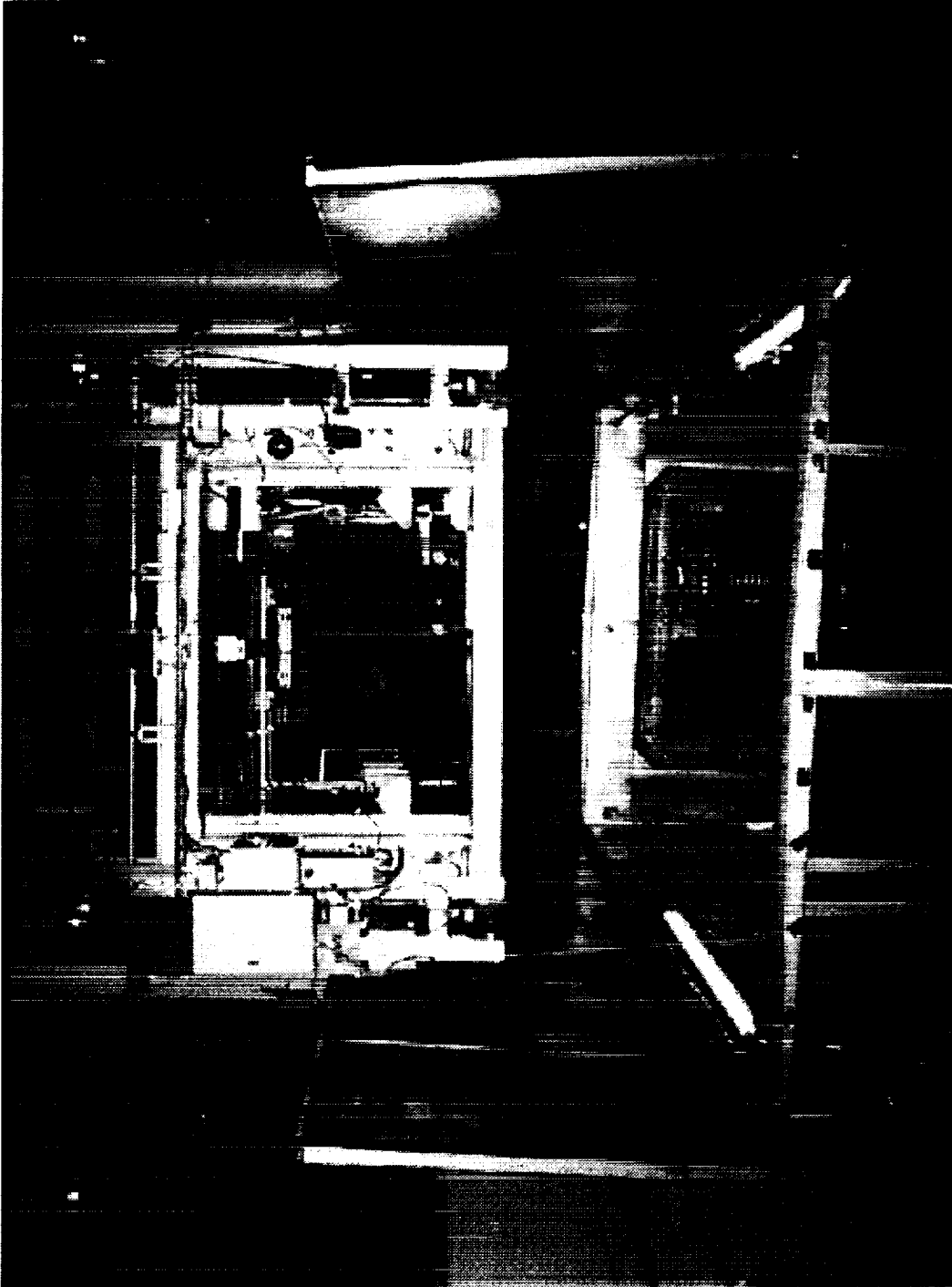
Figure 17. Access Housing closest to the NTF's control room being lifted by overhead crane.
