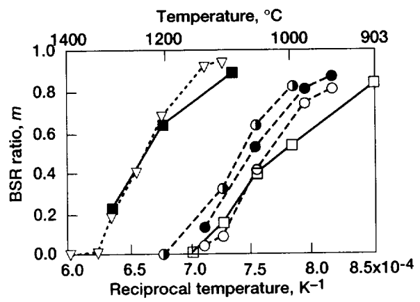
Figure 8.—Results of 1-hr BSR test on polycrystalline oxide fibers in their as-received condition and on Nextel 610 and Altex fibers before and after annealing at 1100 and 1300 °C [8,9].
