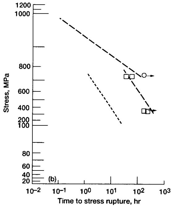
Figure 6.—Annealing increases rupture time of as-received oxide fibers (arrows indicate interrupted tests). (a) Nextel 610. (b) Altex.
