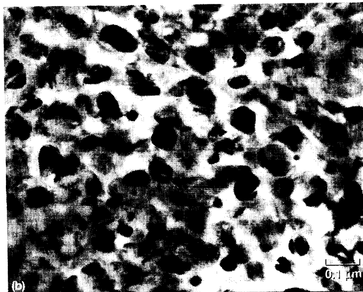
Figure 10.—Altex fiber grain size increased fourfold after 3-hr exposure at 1300 °C. (a) As-received grain size = 0.02 μm. (b) After annealing at 1300 °C.
