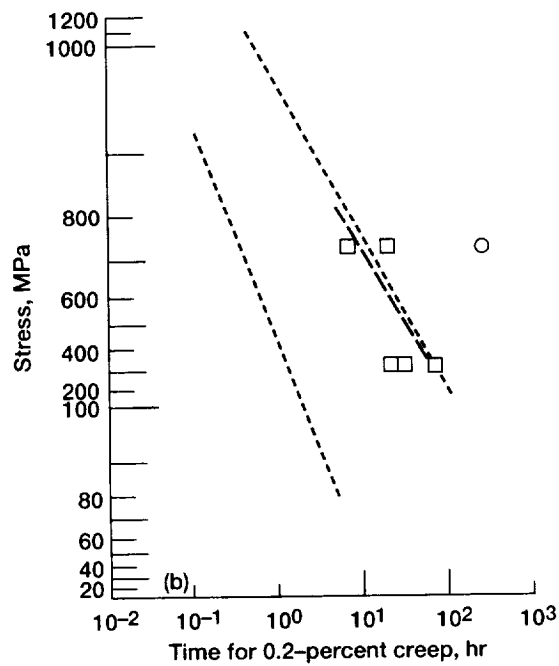
Figure 5.—Effects of annealing on 0.2-percent creep strength. (a) Nextel 610. (b) Altex.
