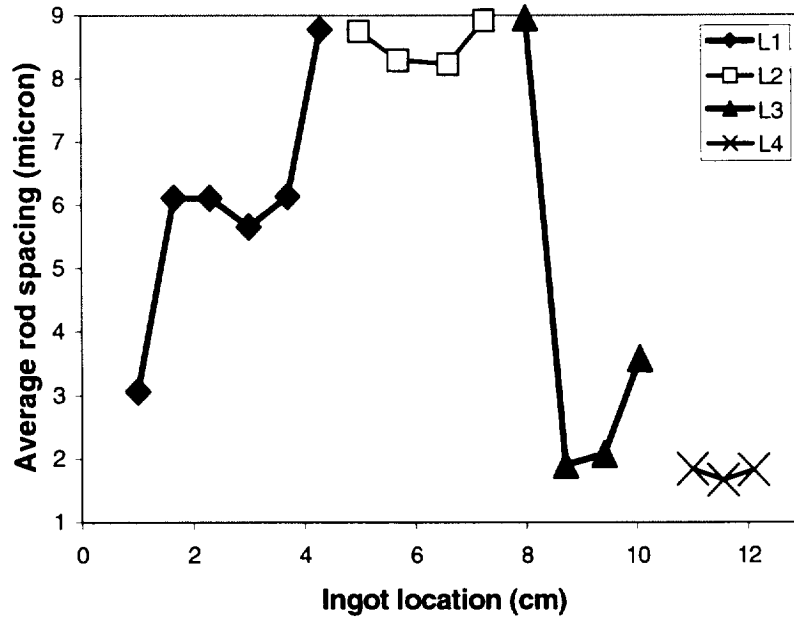
Figure 1. Average rod spacing \lambda along the ingot number 3. Gussed translation rates: L1: V=6.8\text{cm/hr} ; L2: V=4.1\text{cm/hr} ; L3: V=2.1\text{cm/hr} ; L4: V=0.83\text{cm/hr}
