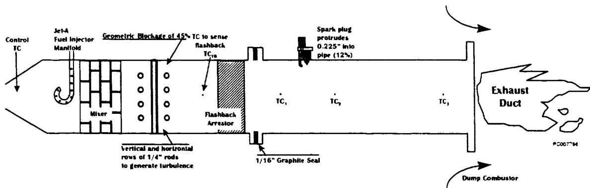
Fig. 4 Flashback arrester test rig
