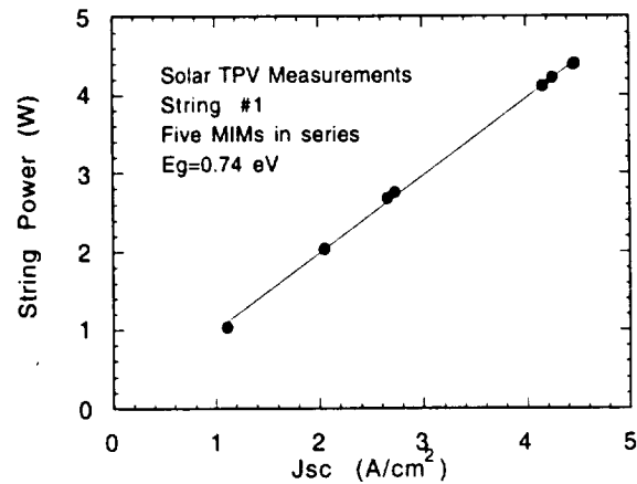
Figure 21.—Variation of output power ( P_{om} ) with J_{sc} for string #1 (STPV Data).
