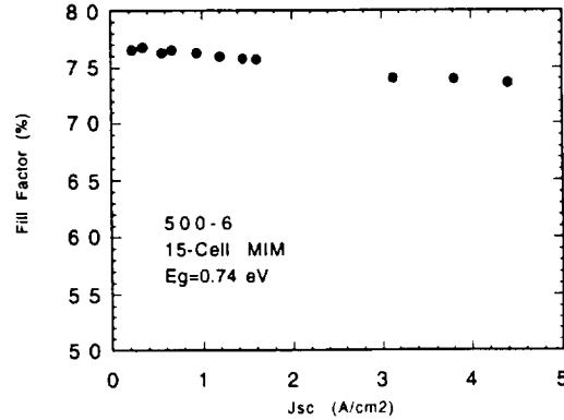
Figure 13.—Variation of the fill factor (FF) with the current density ( J_{sc} ) for a MIM with E_g = 0.74 \text{ eV} .
