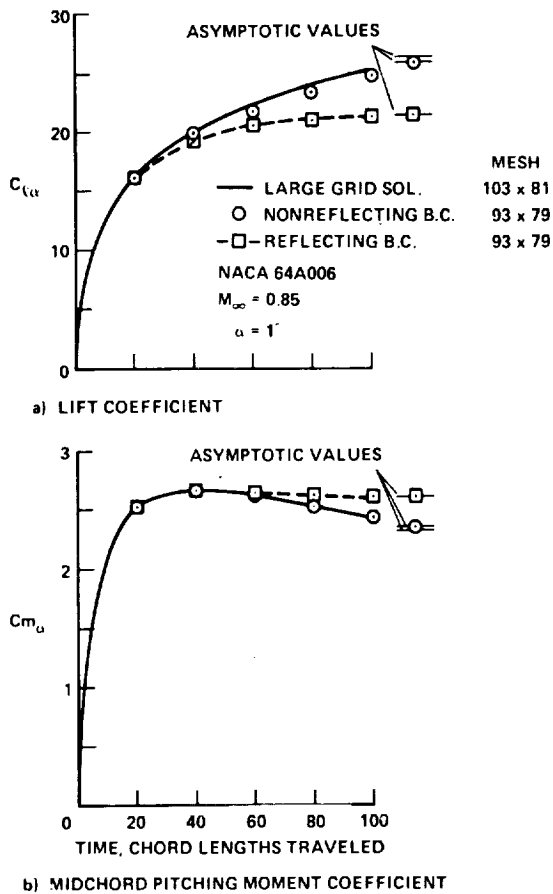
Fig. 2 Effect of far-field boundary distance on C_{L\alpha} and C_{m\alpha} vs t for step change in angle of attack.
