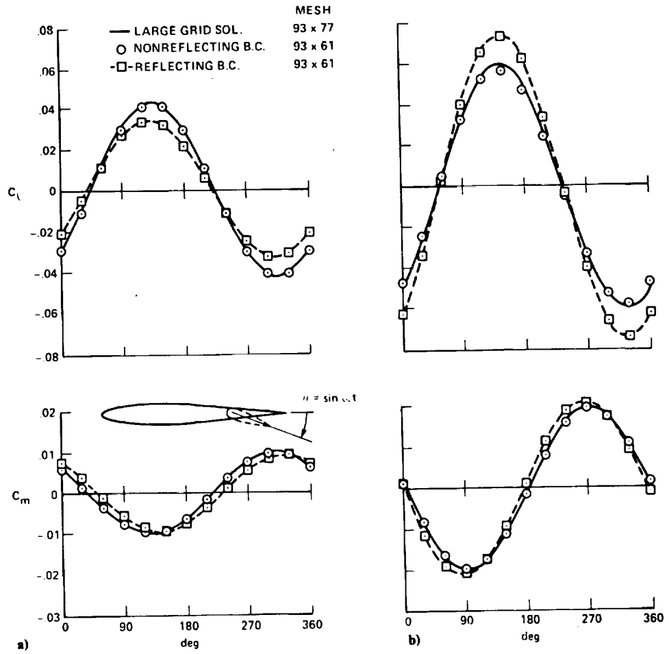
Fig. 4 Effect of far-field distance on C_m and C_l for an NACA 64A006 airfoil with oscillating trailing-edge flap: a) type A, M_\infty = 0.875 , k = 0.468 ; b) type B, M_\infty = 0.854 , k = 0.358 .
