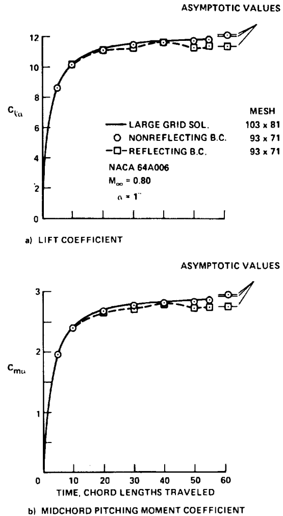
Fig. 3 Effect of far-field boundary distance on C_{L\alpha} and C_{m\alpha} for step change in angle of attack.
