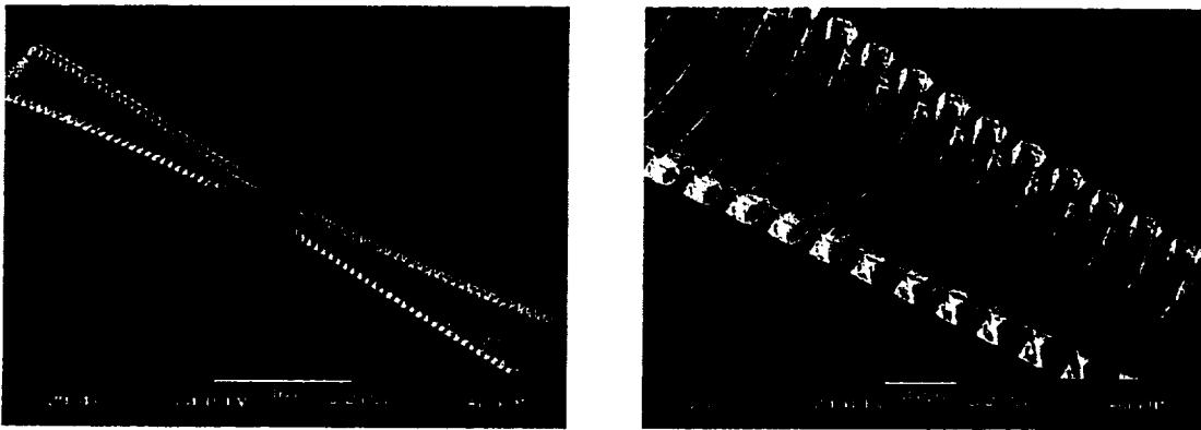
Figure 1: SEM micrograph of replicated version of 2 THz waveguide structure. The original structure was etched using 3 Watts of laser power focused into a 4\ \mu\text{m} spot in 200 Torr of chlorine gas. The laser beam was scanned at 4 cm/s and incrementally moved 2 micrometers between line scans removing 0.65\ \mu\text{m} shavings per pass of the laser over the surface. (b) SEM close-up of ridges.
