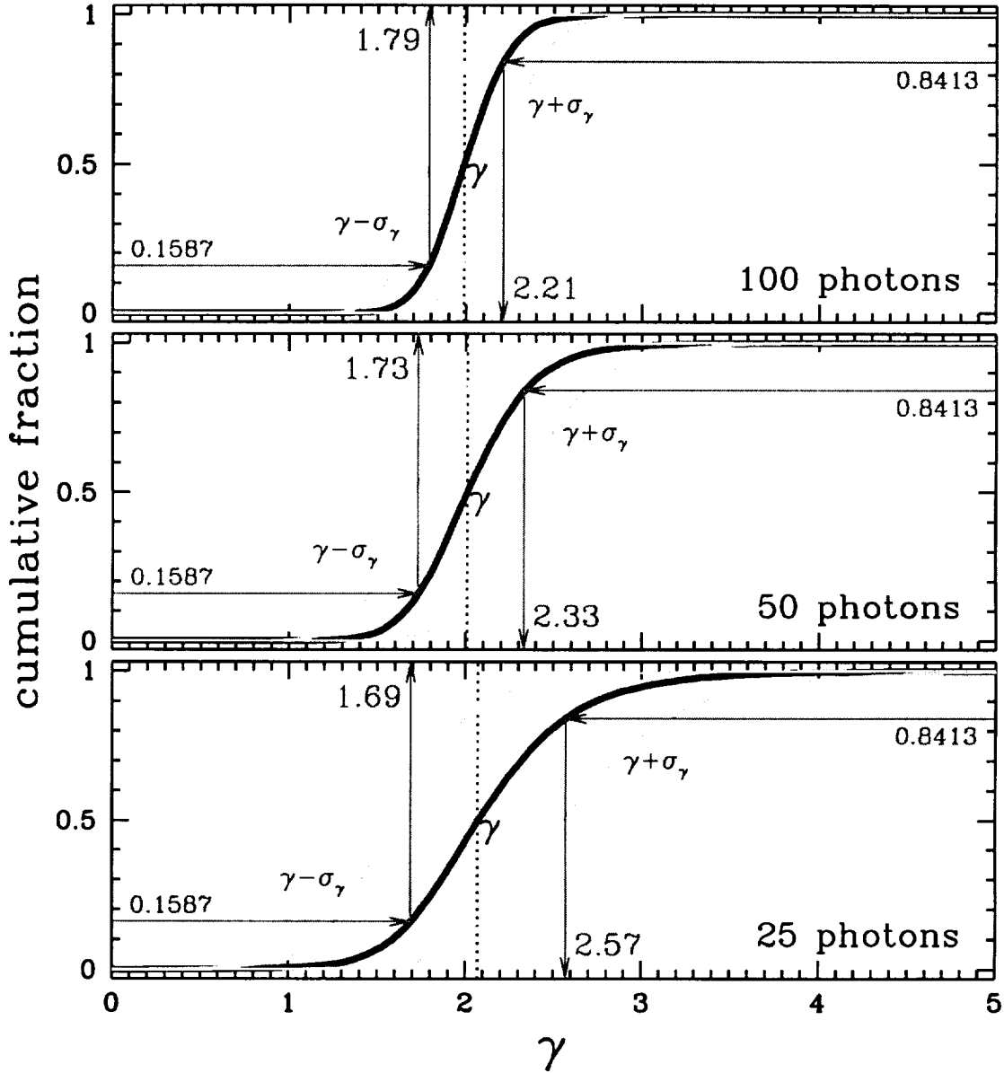
Fig. 10.— Error analysis of the Levenberg-Marquardt method results using the \chi_\gamma^2 statistic with one free parameter. The thick curve in each panel shows the cumulative distribution of the best-fit estimates of the slope \gamma . The right (left) thin curve in each panel shows the cumulative distribution of \gamma plus (minus) \sigma_\gamma which is the error estimate of the best-fit slope value. The statistical analysis of this data is presented in Table 4.
