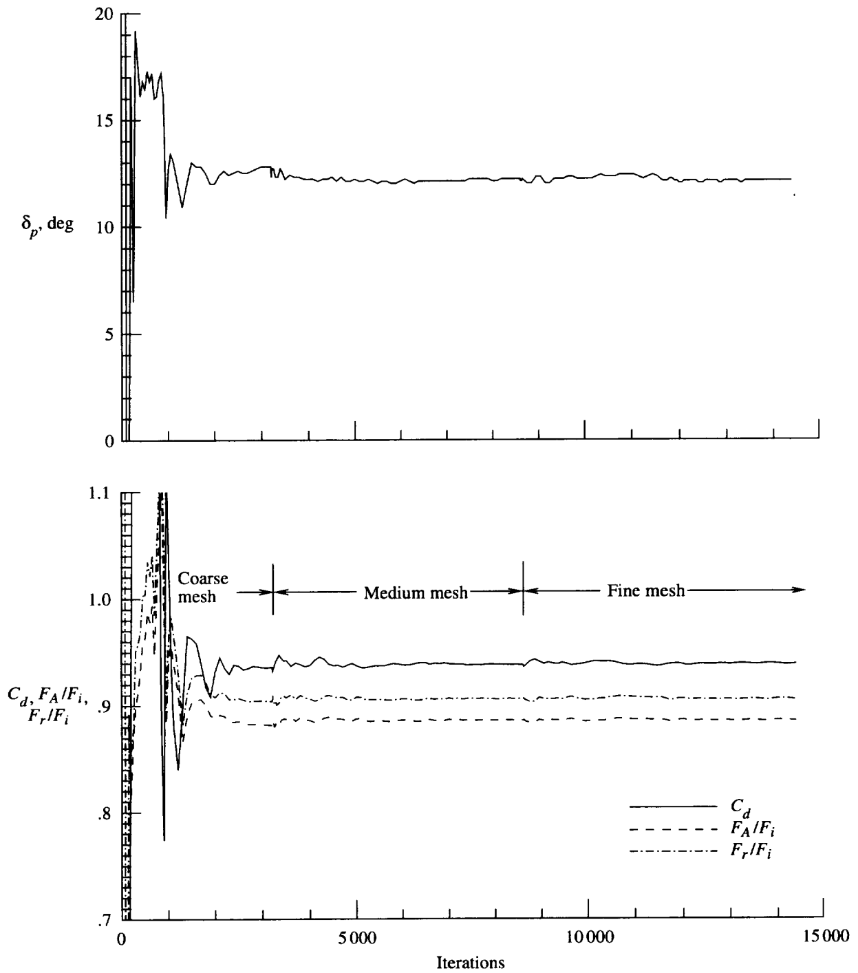
Figure 31. Solution convergence history for concave ramp, high Mach number nozzle at M = 0.1 and NPR = 102 .
