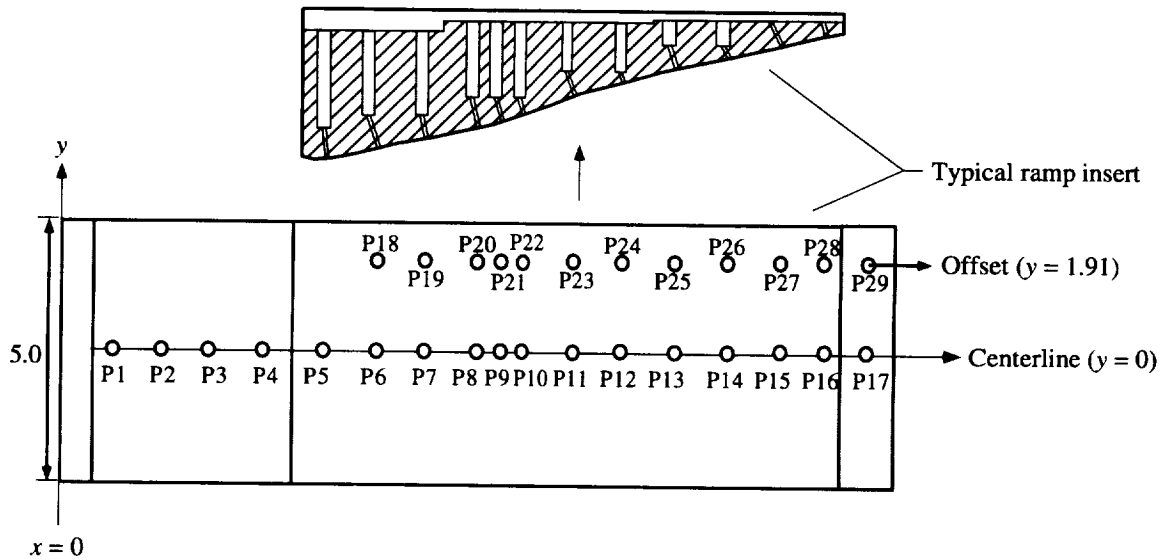
Figure 9. Orientation of static pressure orifices along expansion ramp. Dimensions are in inches.
