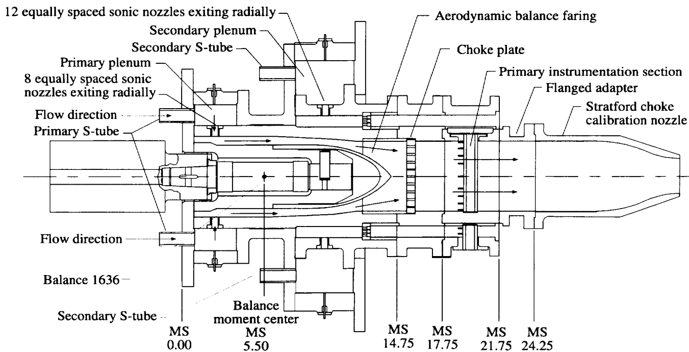
Figure 11. Typical hardware setup for balance calibrations on propulsion simulation system.
