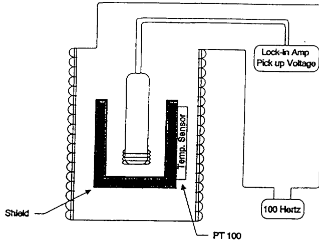
Fig. 4. Schematic cross section of the experimental setup used for measuring the transition temperature and determining the shielding factor for the magnetic shields.
