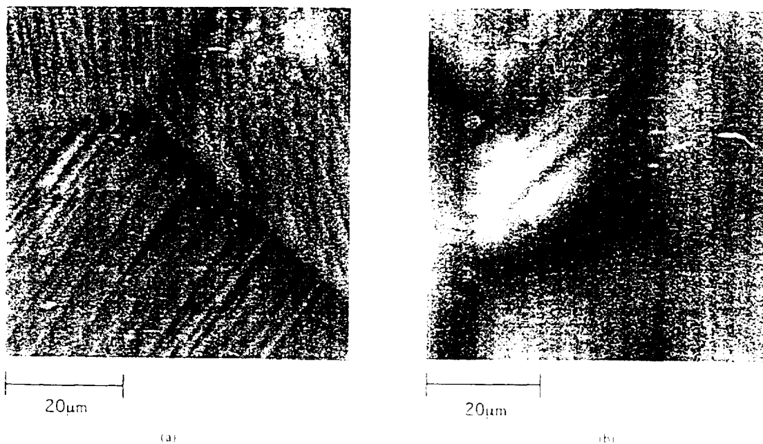
Fig. 8. These photos show the 60\text{ }\mu\text{m} \times 60\text{ }\mu\text{m} AFM image of grain boundaries for a) BSCCO and b) 99.9% pure silver. The 99.9% silver shows smaller grains with impurities.
