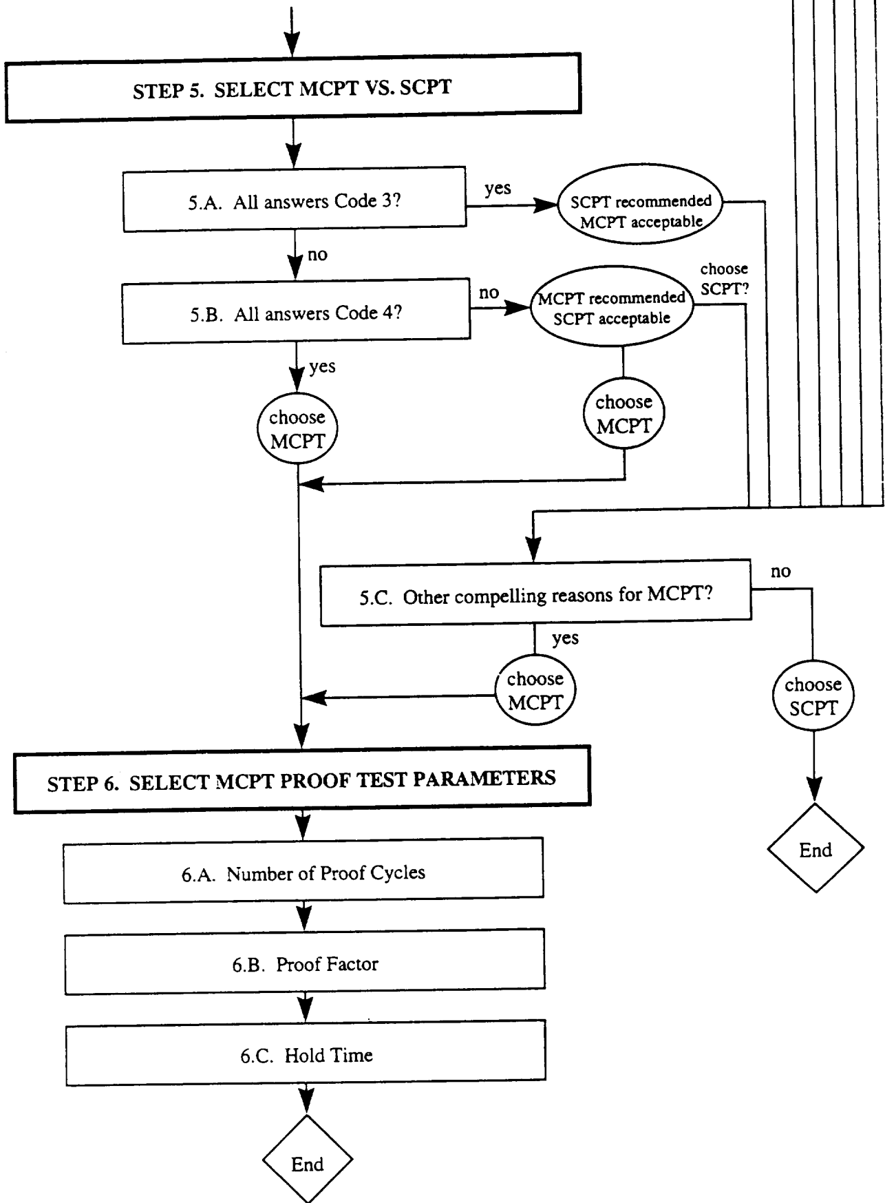
Figure 7.1 Flow chart for Engineering Guidelines (Cont.)
