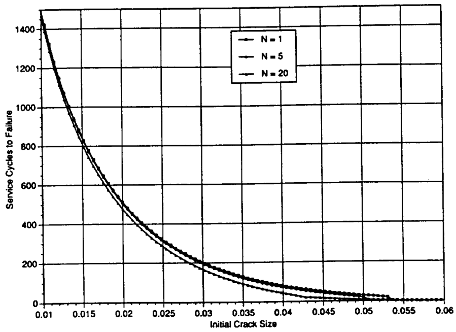
Figure 4.6. Service cycles to failure as a function of initial crack depth for a sample problem
