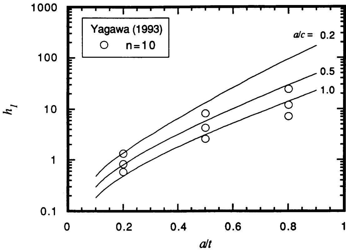
Figure A13. Comparison of reference stress h , predictions with Yagawa (1993) finite element results
