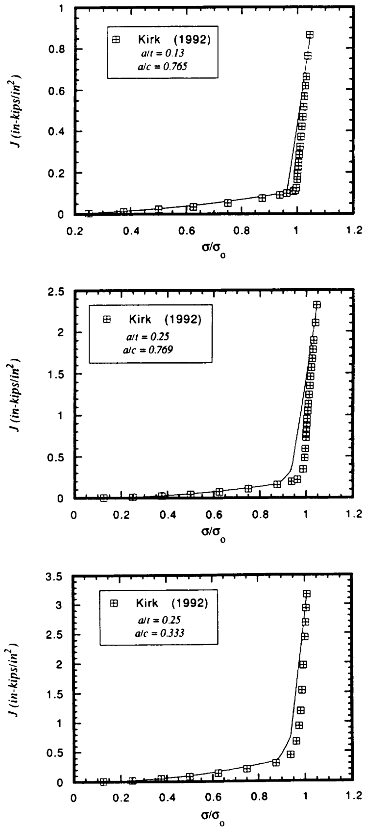
Figure A11. Comparison of reference stress J predictions with Kirk (1992) finite element results in terms of normalized applied stress
