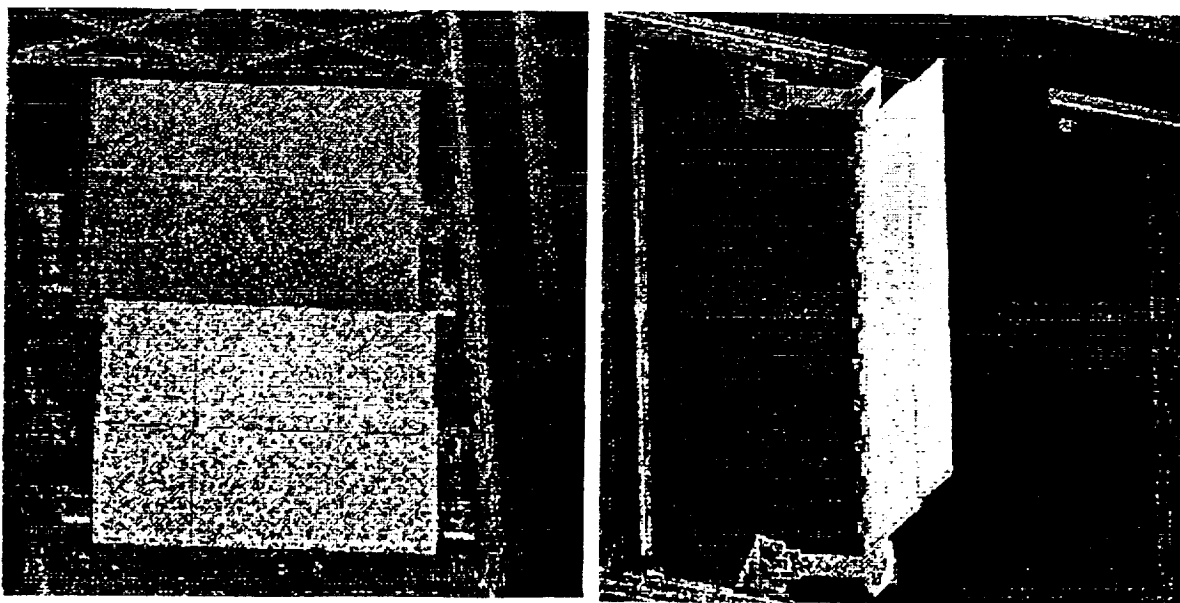
Fig. 4 : SEM IMAGE OF LOUVERS IN THE SEMI-OPEN AND OPEN POSITION. THE WIDTH OF EACH LOUVER IS 500 \mu\text{m}
