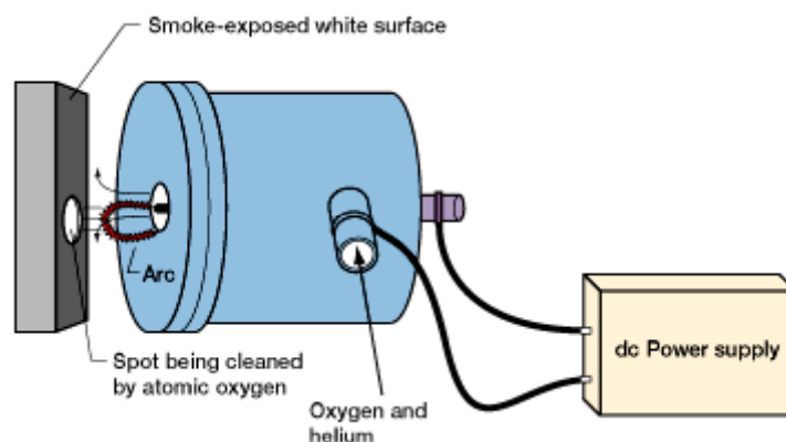
Atmospheric atomic oxygen cleaning system.
