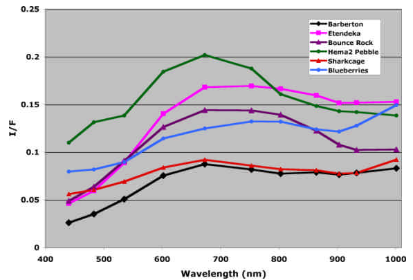
Figure 4. Pancam spectra for various cm-size cobbles seen at Meridiani Planum compared to a typical spectrum for the blueberries.
