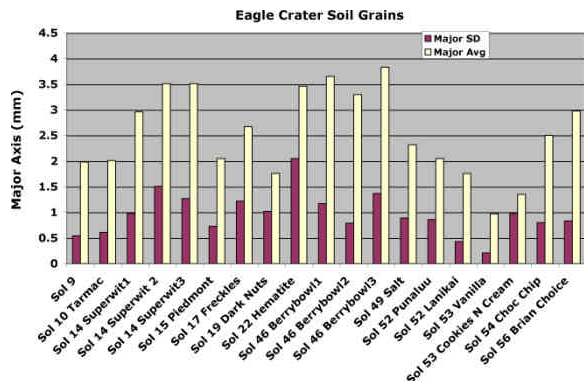
Figure 1. Average major axis grain size (yellow) and standard deviation (red) based upon MI images for soils inside Eagle crater.
