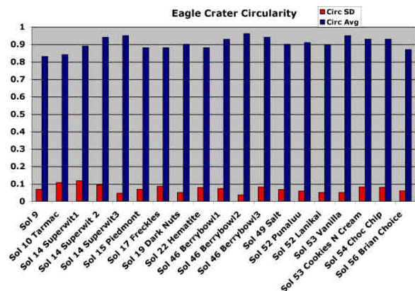
Figure 3. Average circularity of grains (blue) and standard deviation (red) within Eagle crater soils indicates most grains are very circular in shape.
