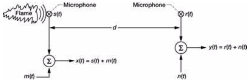
Measurement of sound speed using two microphones.
